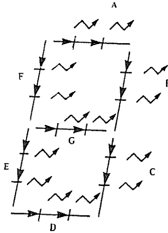
Fig. 6.10: Seven-Segment LED
