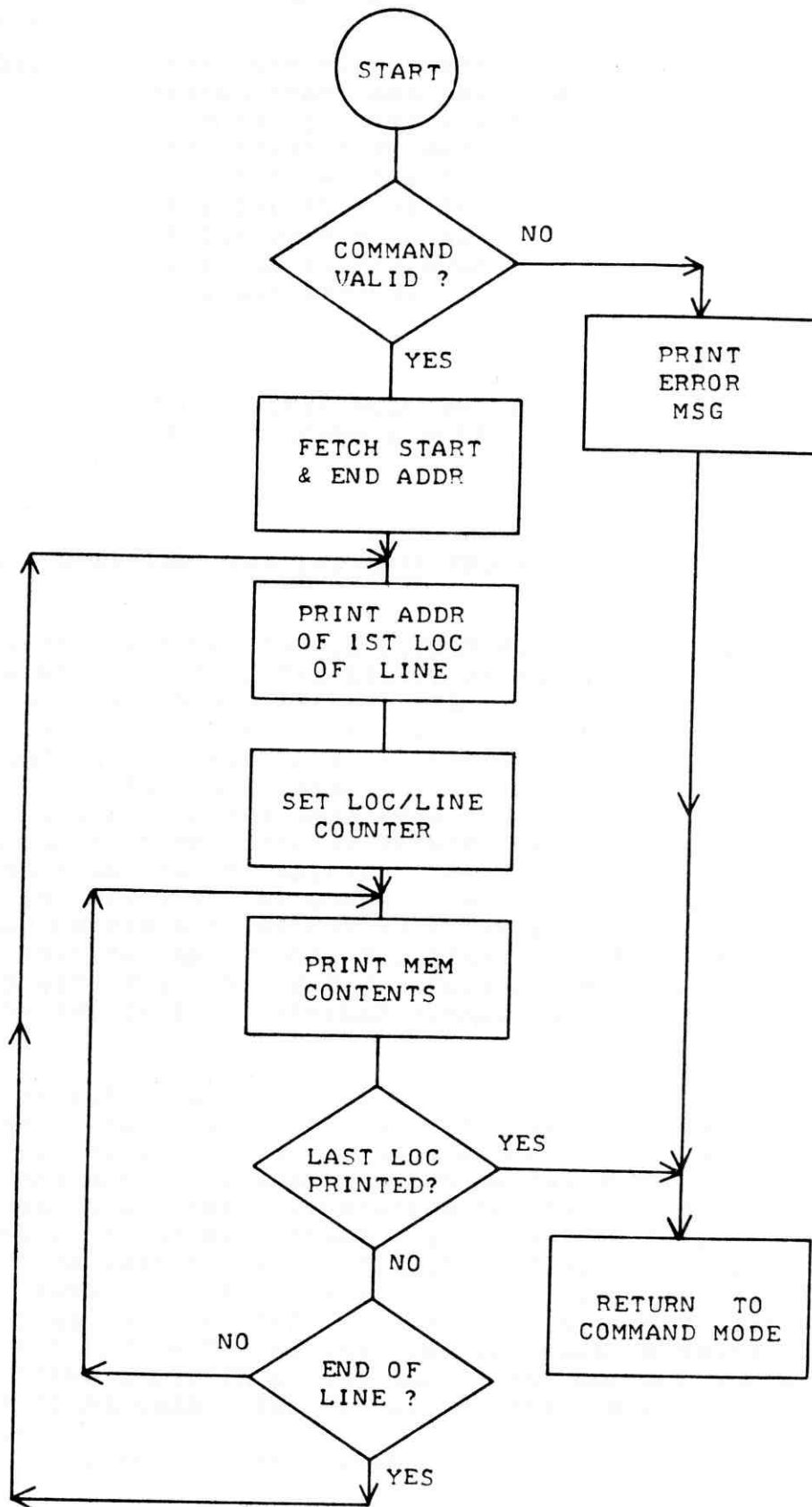
MEMORY "DUMP" ROUTINE FLOW CHART
