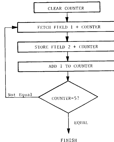
Moving Five Bytes of Data with Counter FIGURE 6.2
