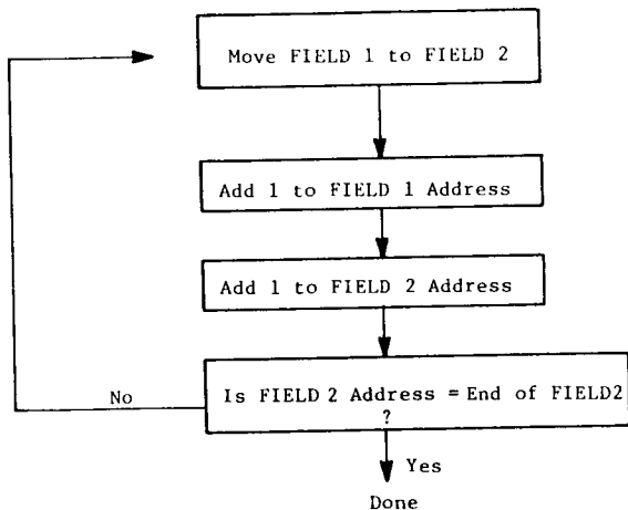
Moving Five Bytes of Data with Loop FIGURE 6.1
