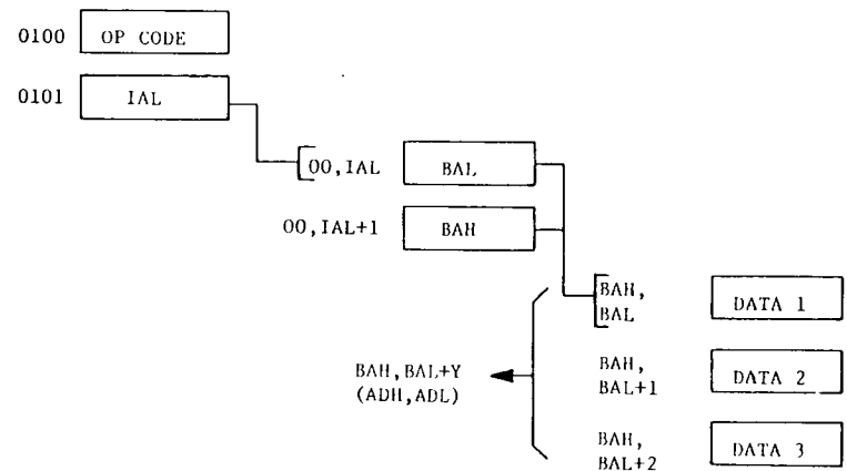
Indirect Indexed Addressing FIGURE 6.6
