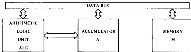
Partial Block Diagram Including Arithmetic Logic Unit of a R6500 Computer System Microprocessor
