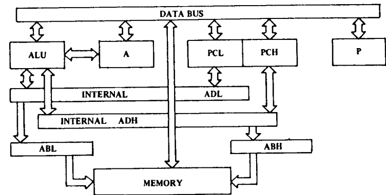
Partial Block Diagram of a R6500 Microcomputer System Microprocessor Including Program Counter and Internal Address Bus
