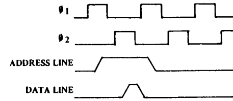
Example of Timing -- A R6500 Microcomputer System Microprocessor
