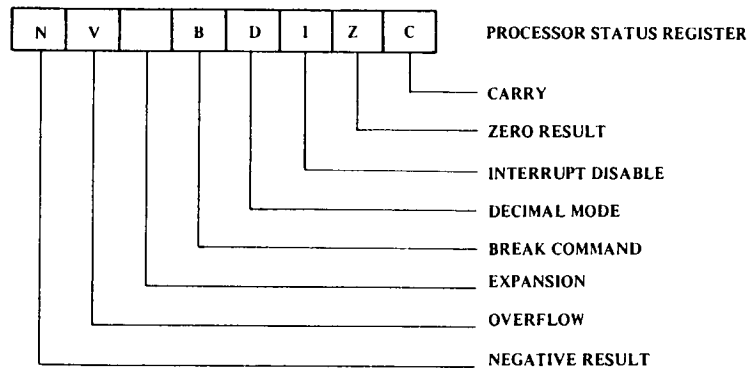
Processor Status Register "P"
