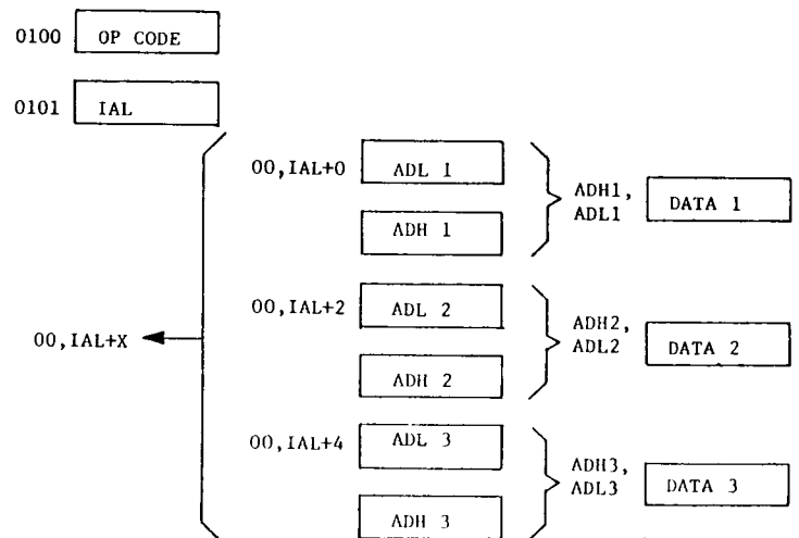
Indexed Indirect Addressing FIGURE 6.5
