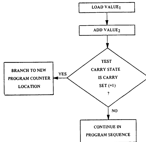
Use of Conditional Test FIGURE 4.2
