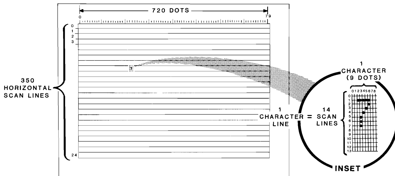
Figure 3.1. Character Generation
