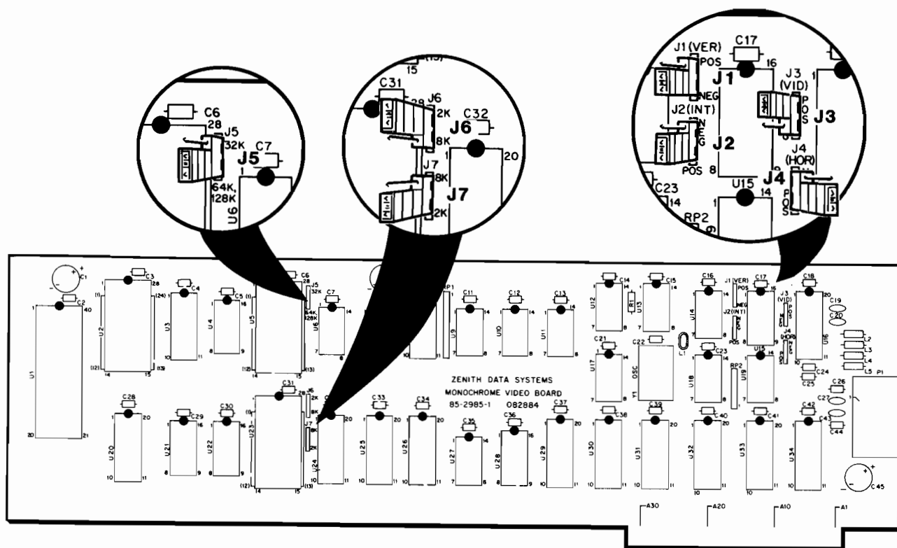
Figure 2.12. Z-329 Component Layout
