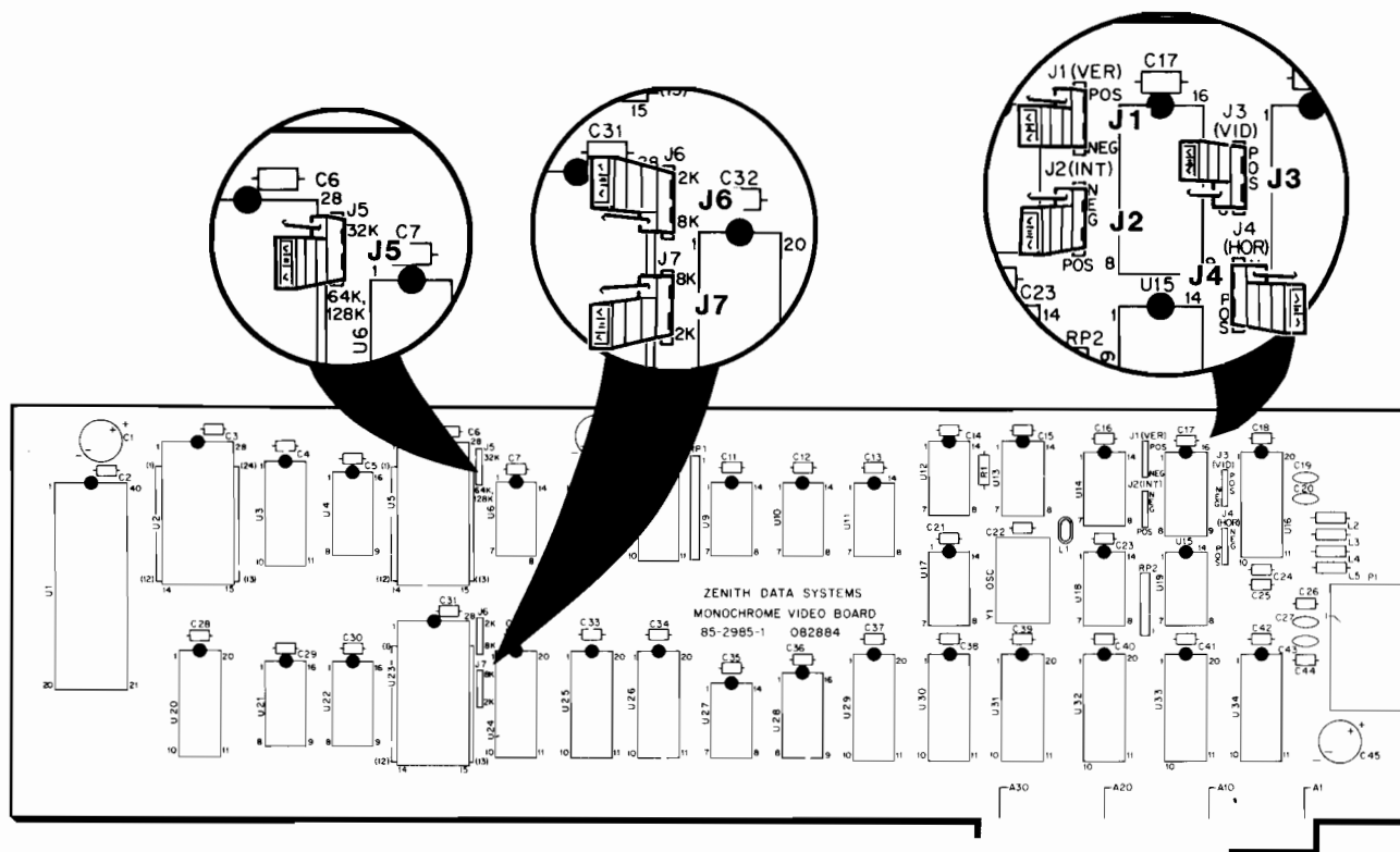
Figure 2.4. Z-329 Card Component Layout
