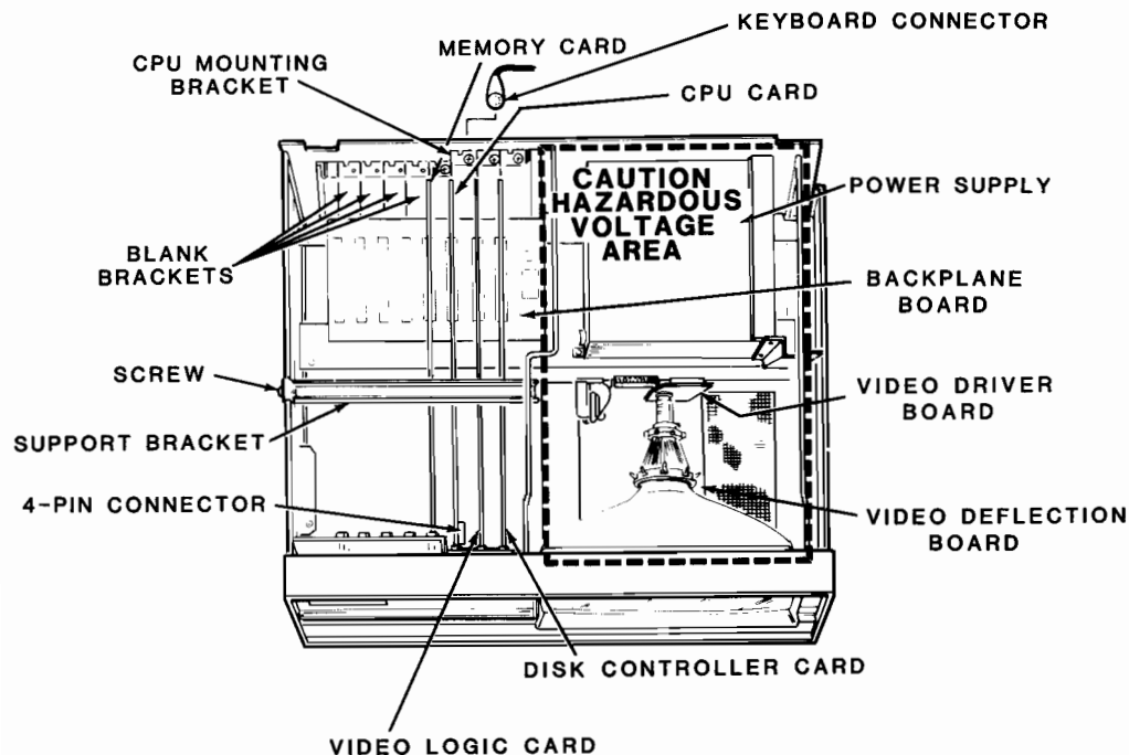
Figure 2.2. Z-160 Chassis
