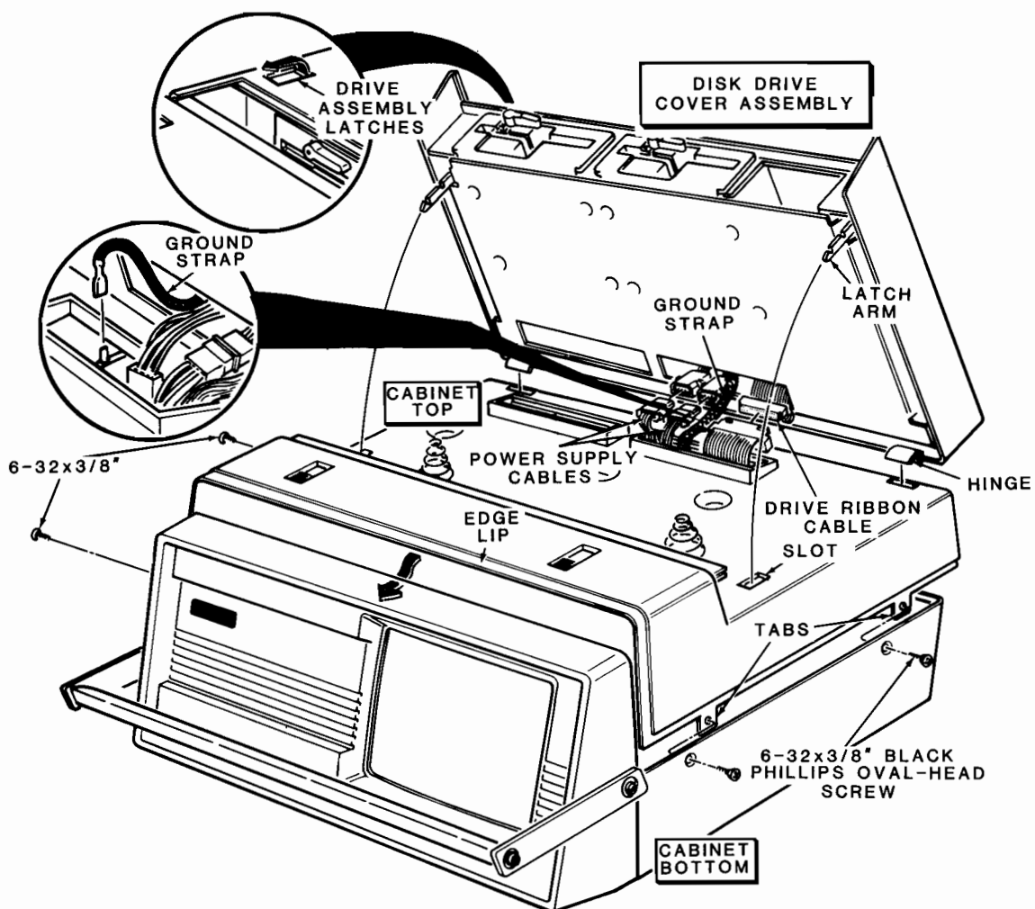
Figure 2.9. Z-160 Reassembly
