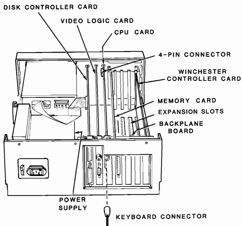
Figure 2.5. Z-150 Chassis
