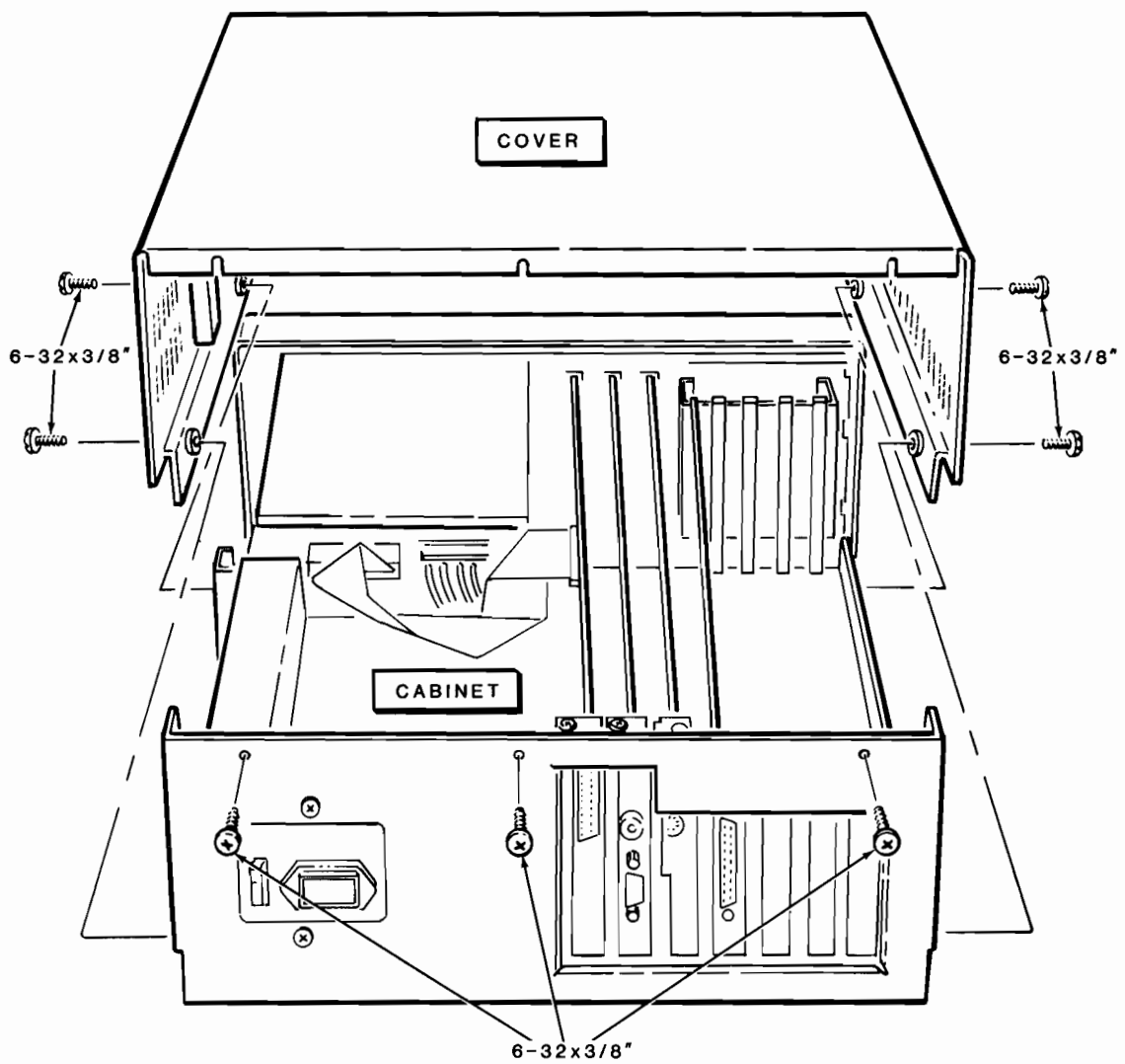
Figure 2.10. Z-150 Reassembly
