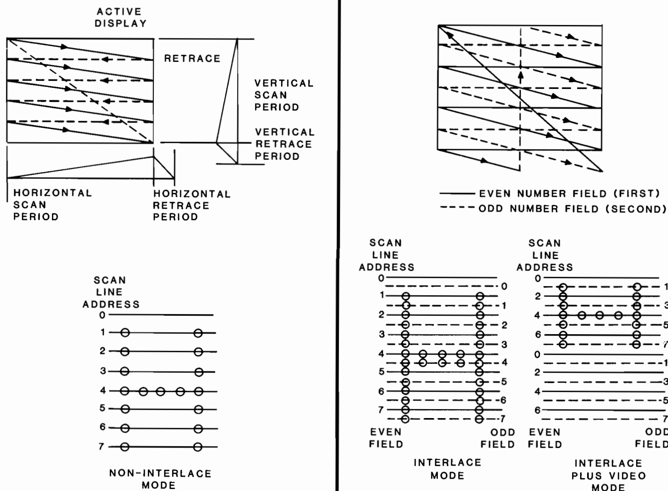
Figure 3.2. Interlace/Non-Interlace Modes
