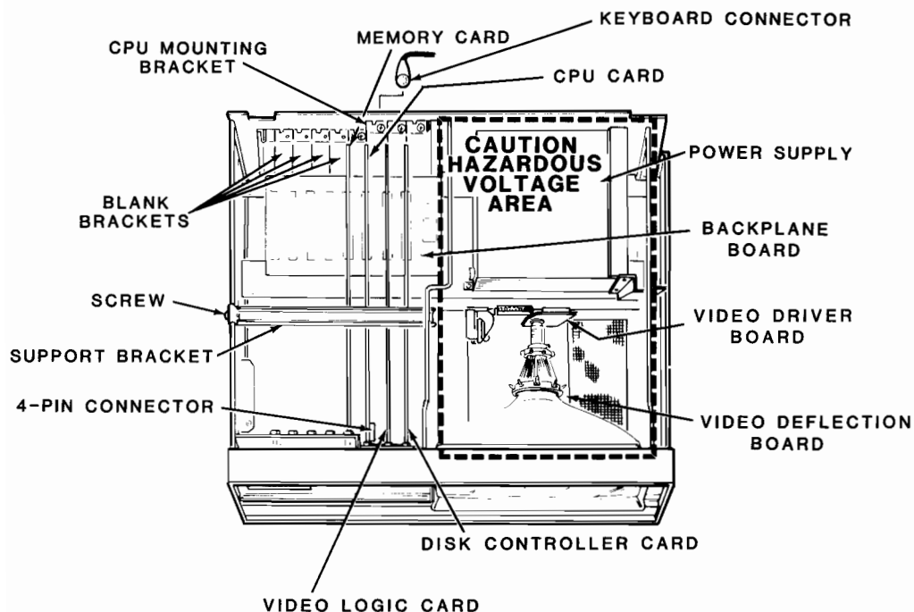
Figure 2.8. Z-160 Chassis
