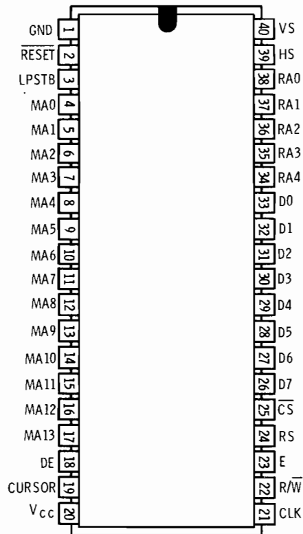
Figure 5.2. 6845 Pinout
