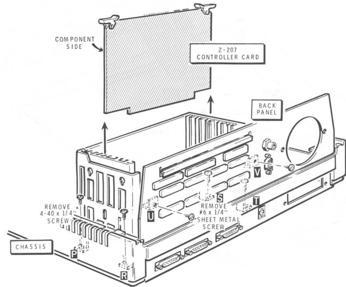
PICTORIAL 5-9
