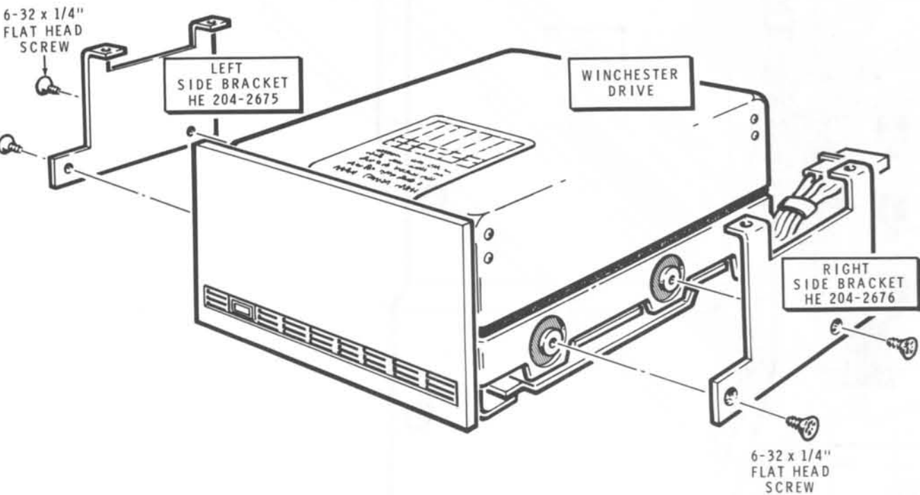
PICTORIAL 5-20 Winchester installation
