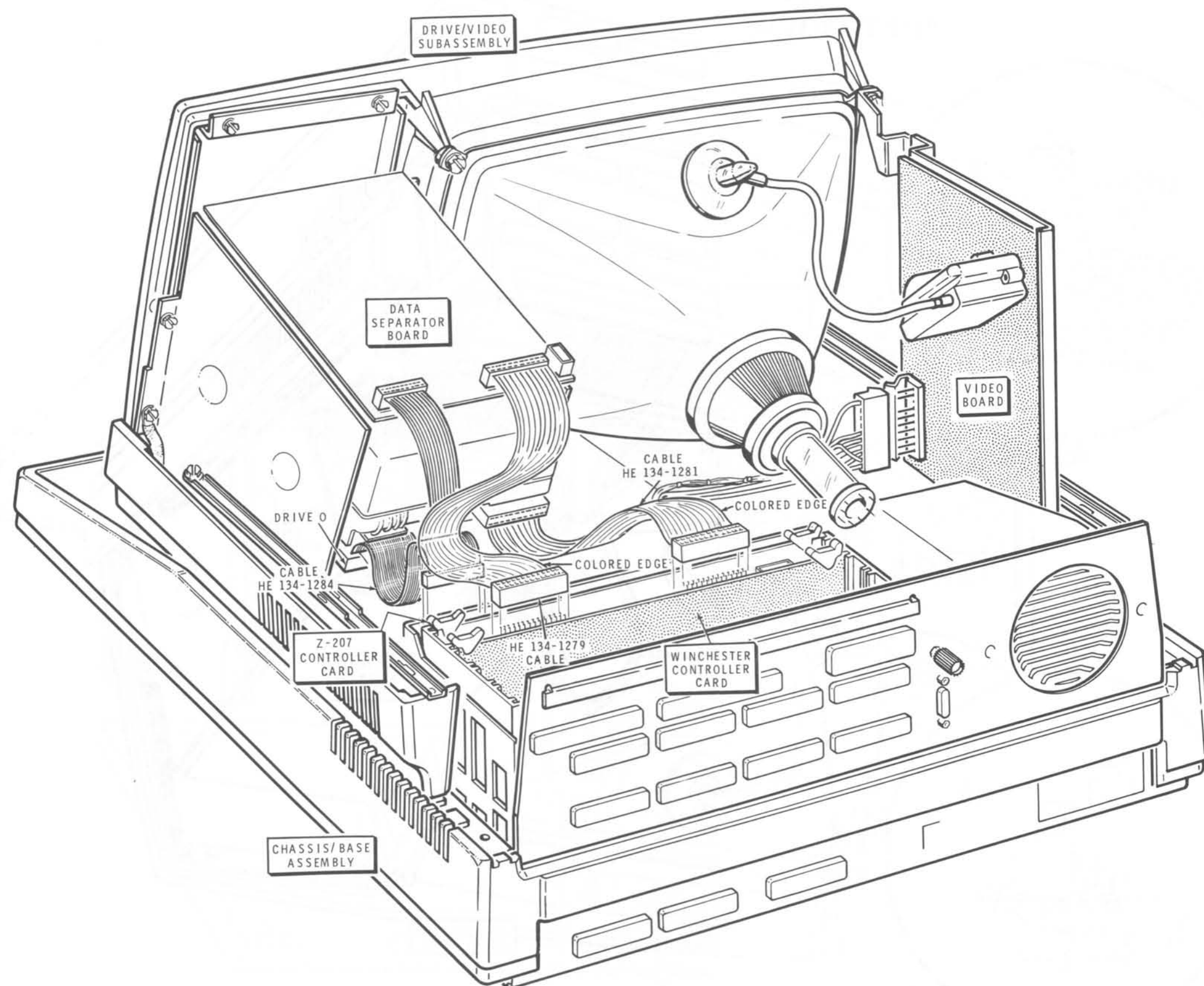
PICTORIAL 4-31
