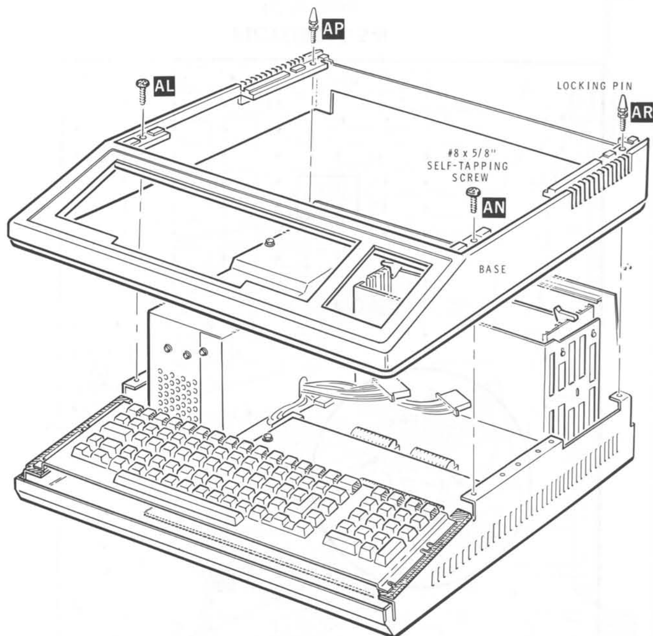
PICTORIAL 5-6 Base removal
