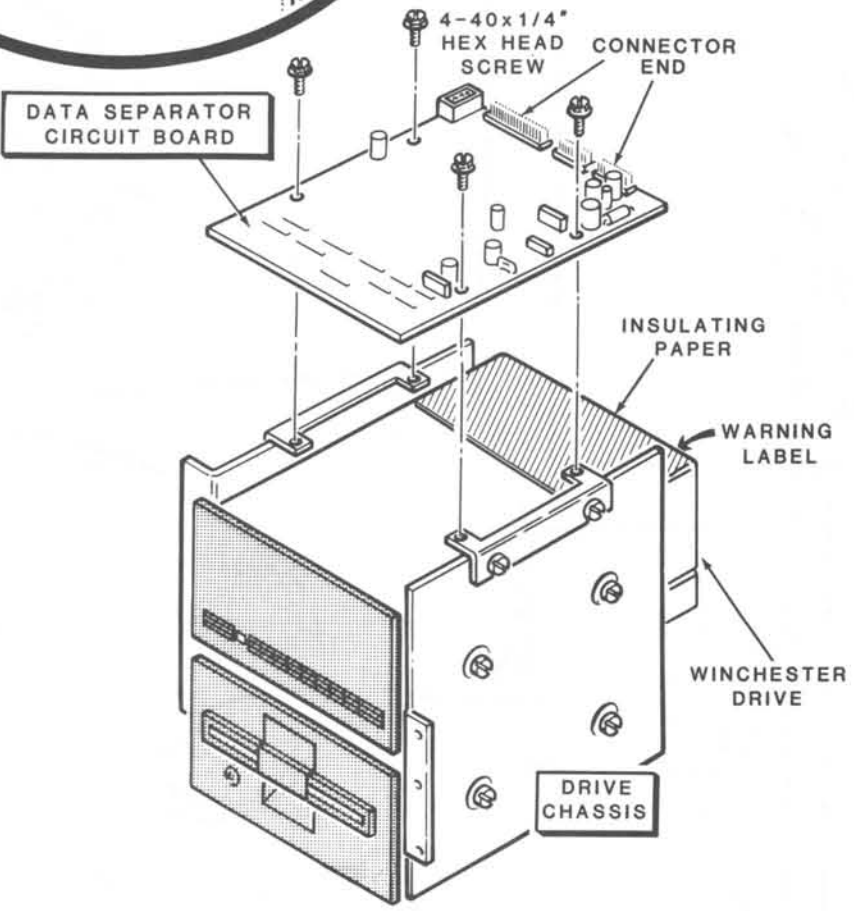
PICTORIAL 4-26
