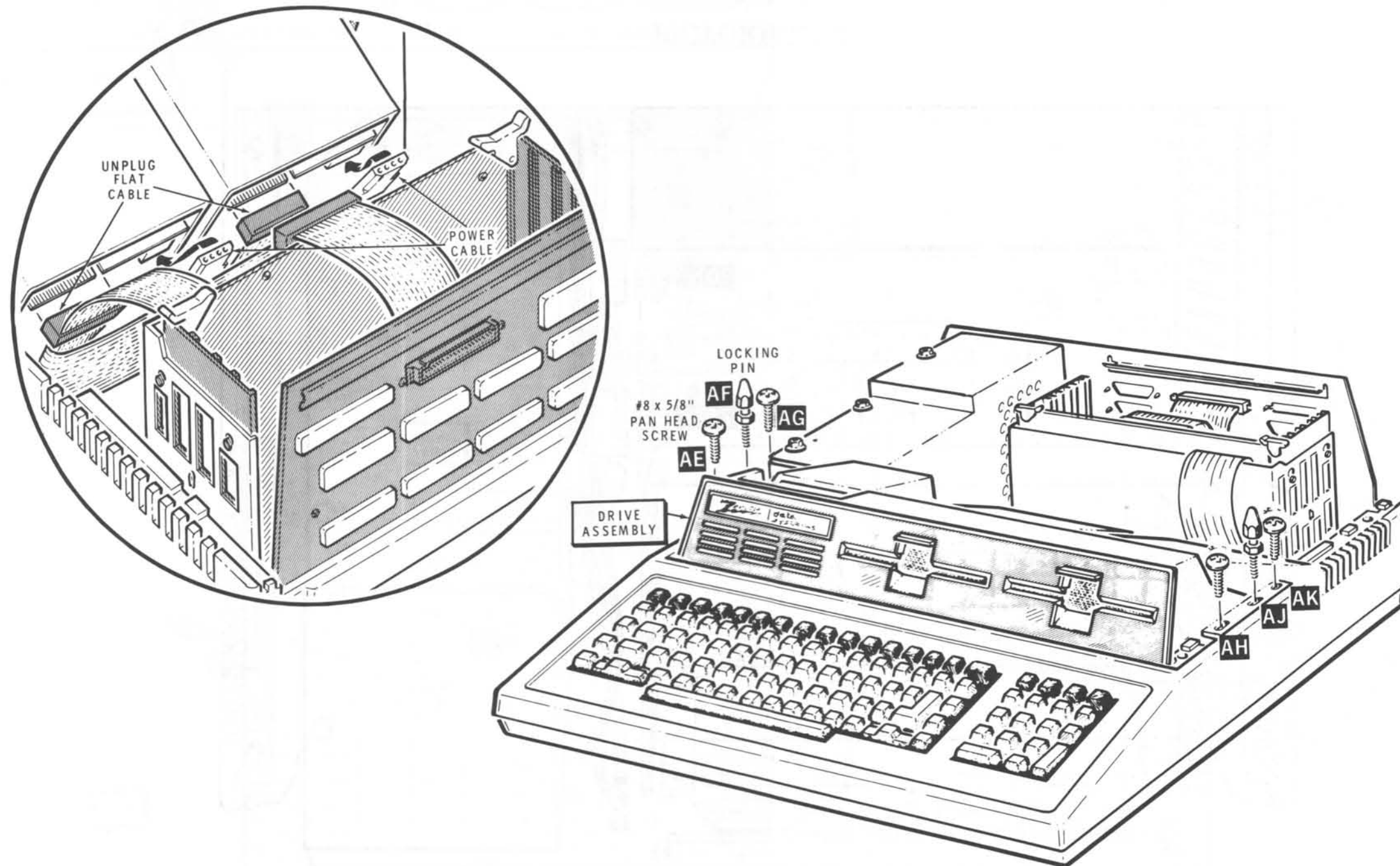
PICTORIAL 5-3 Drive assembly removal
