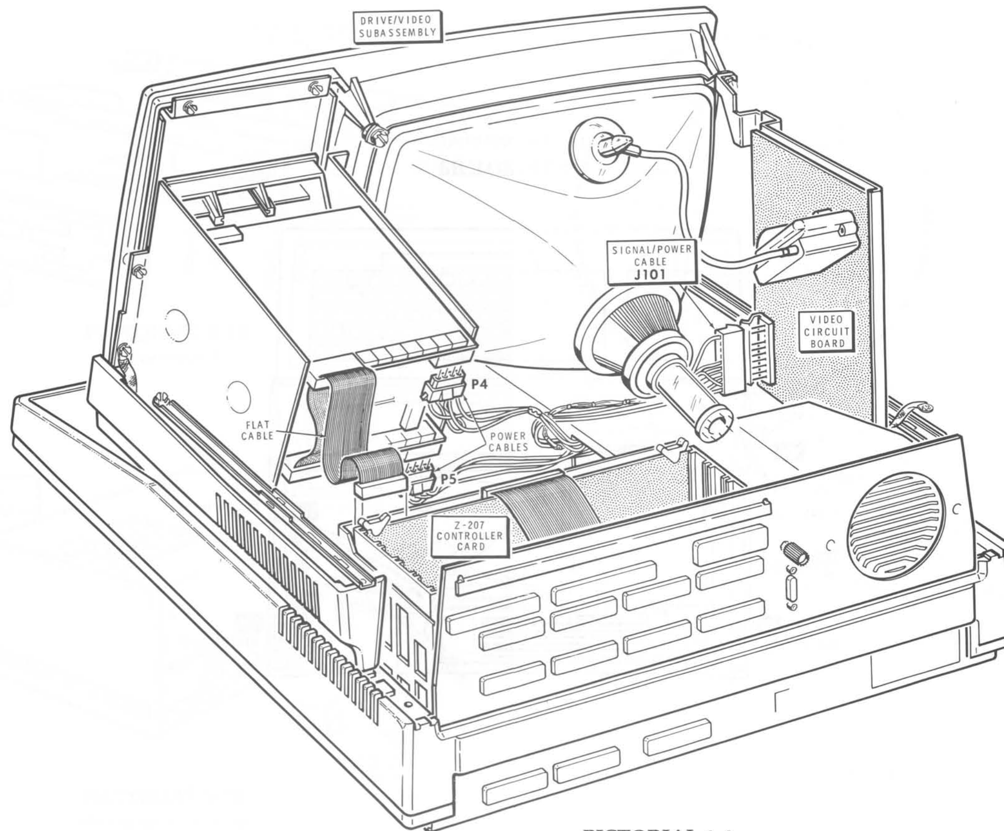
PICTORIAL 4-4
