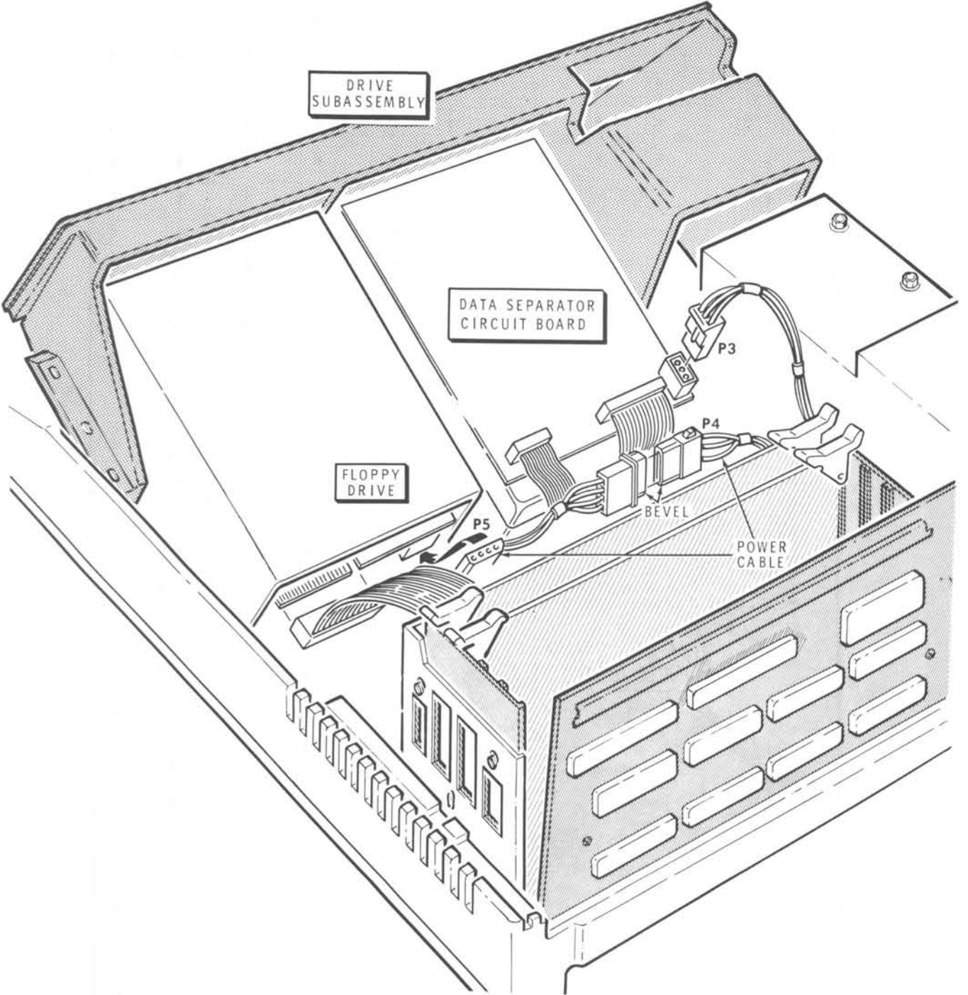
PICTORIAL 5-25 Cable connections
