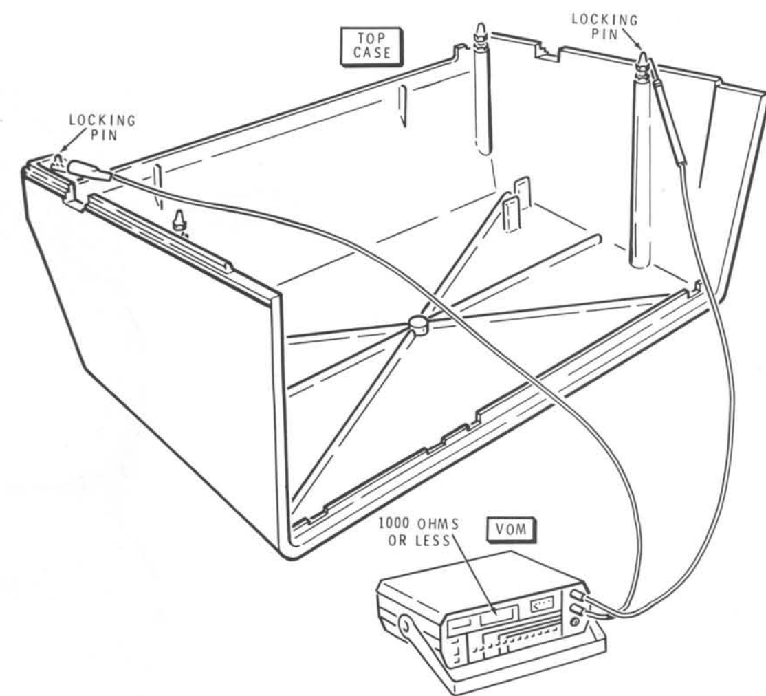
Detail 4-2B Case resistance
