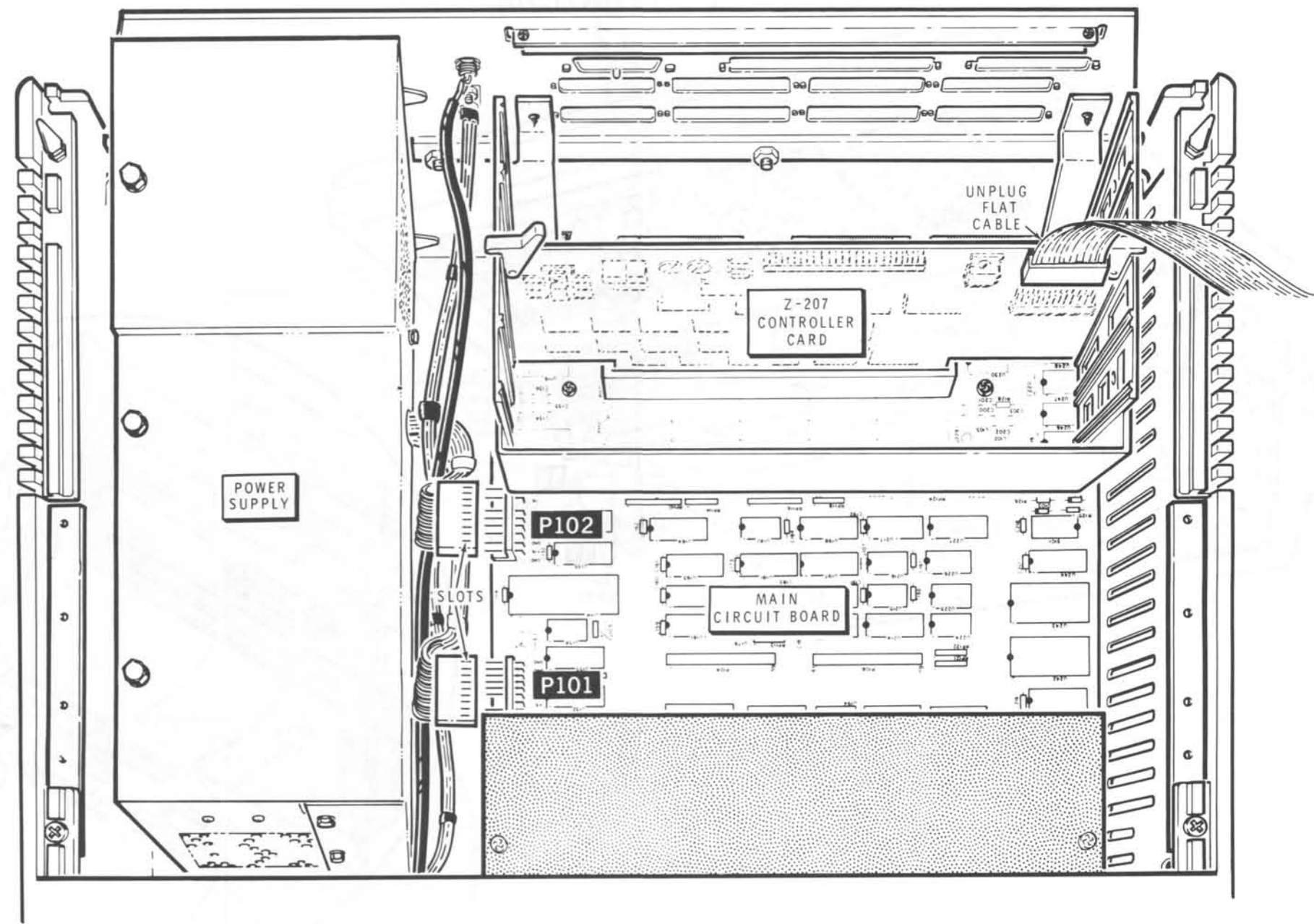
PICTORIAL 5-5 Cables
