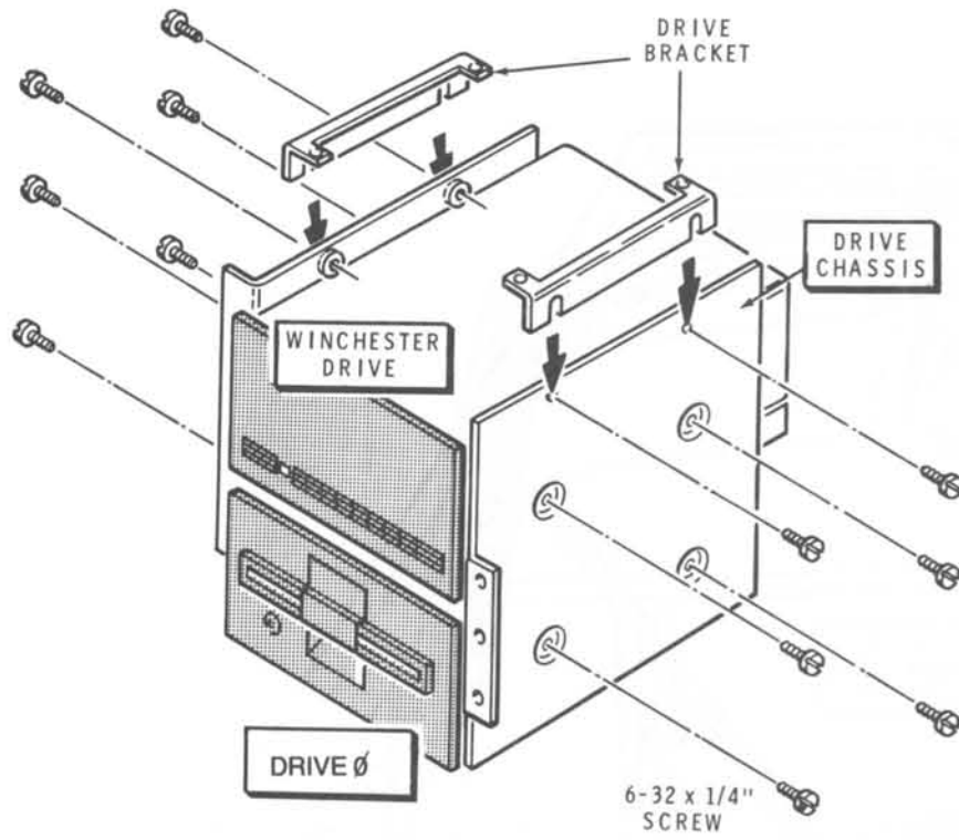
PICTORIAL 4-25
