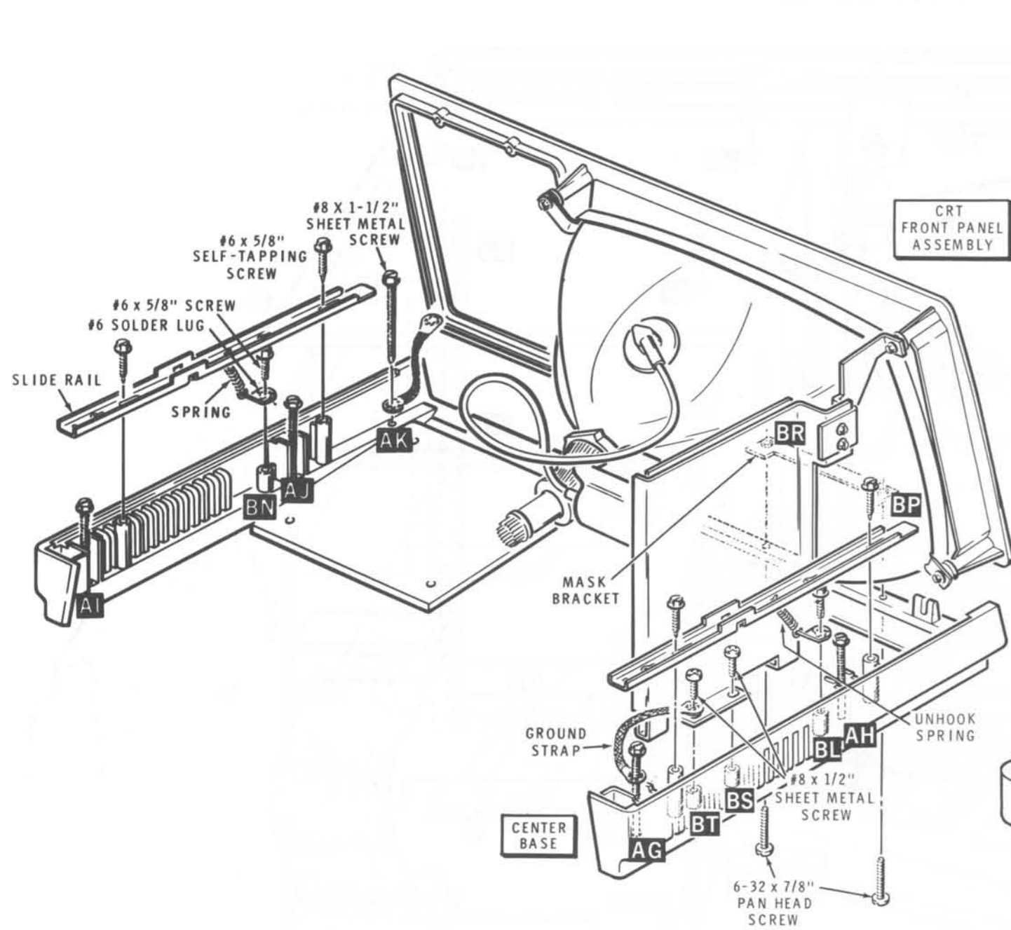
PICTORIAL 4-21 Center base removal
