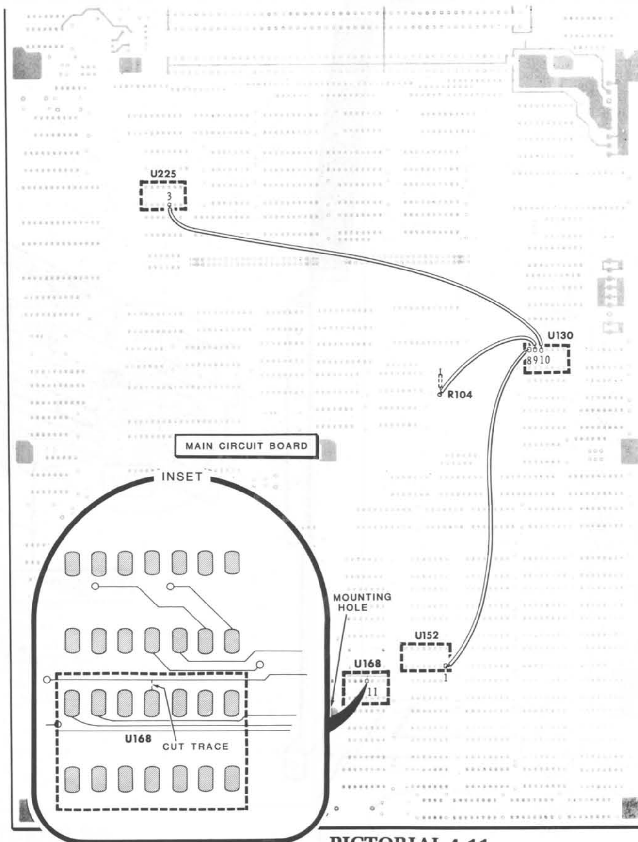
PICTORIAL 4-11
