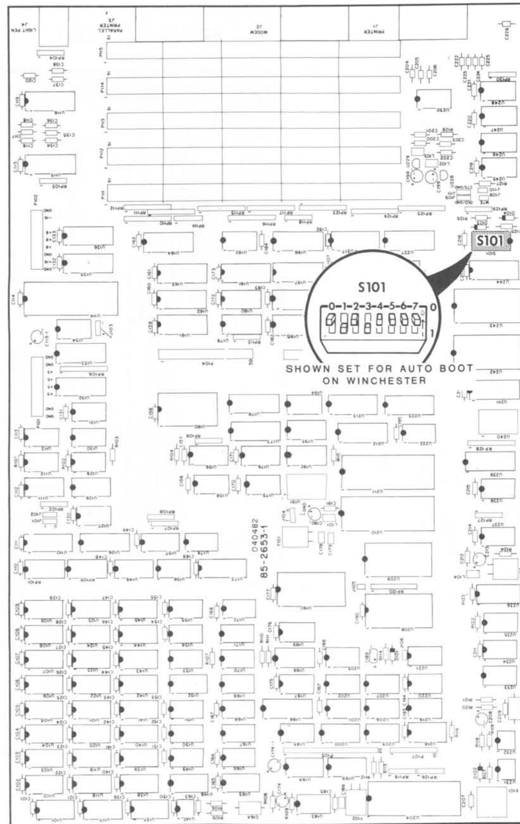
PICTORIAL 4-30
