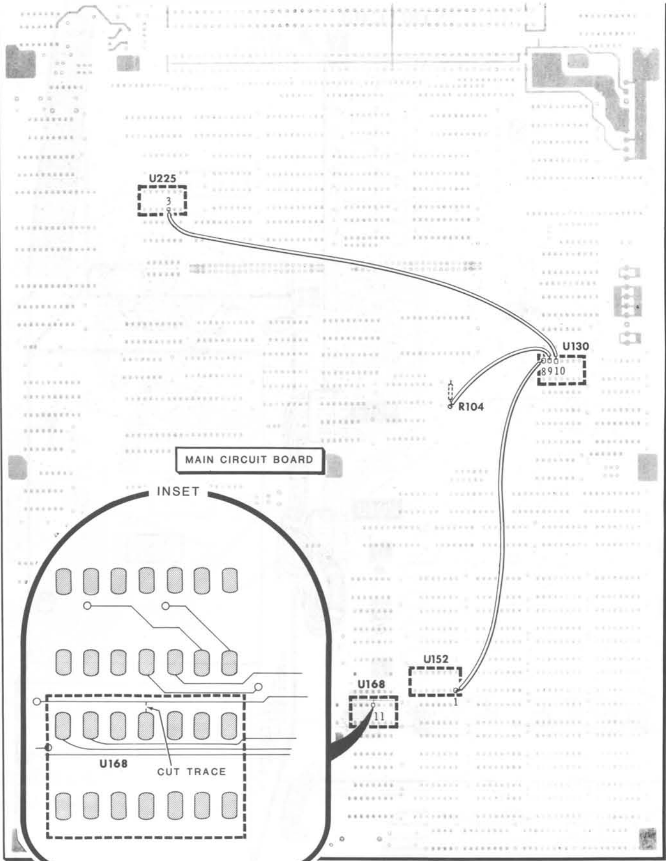
PICTORIAL 5-11
