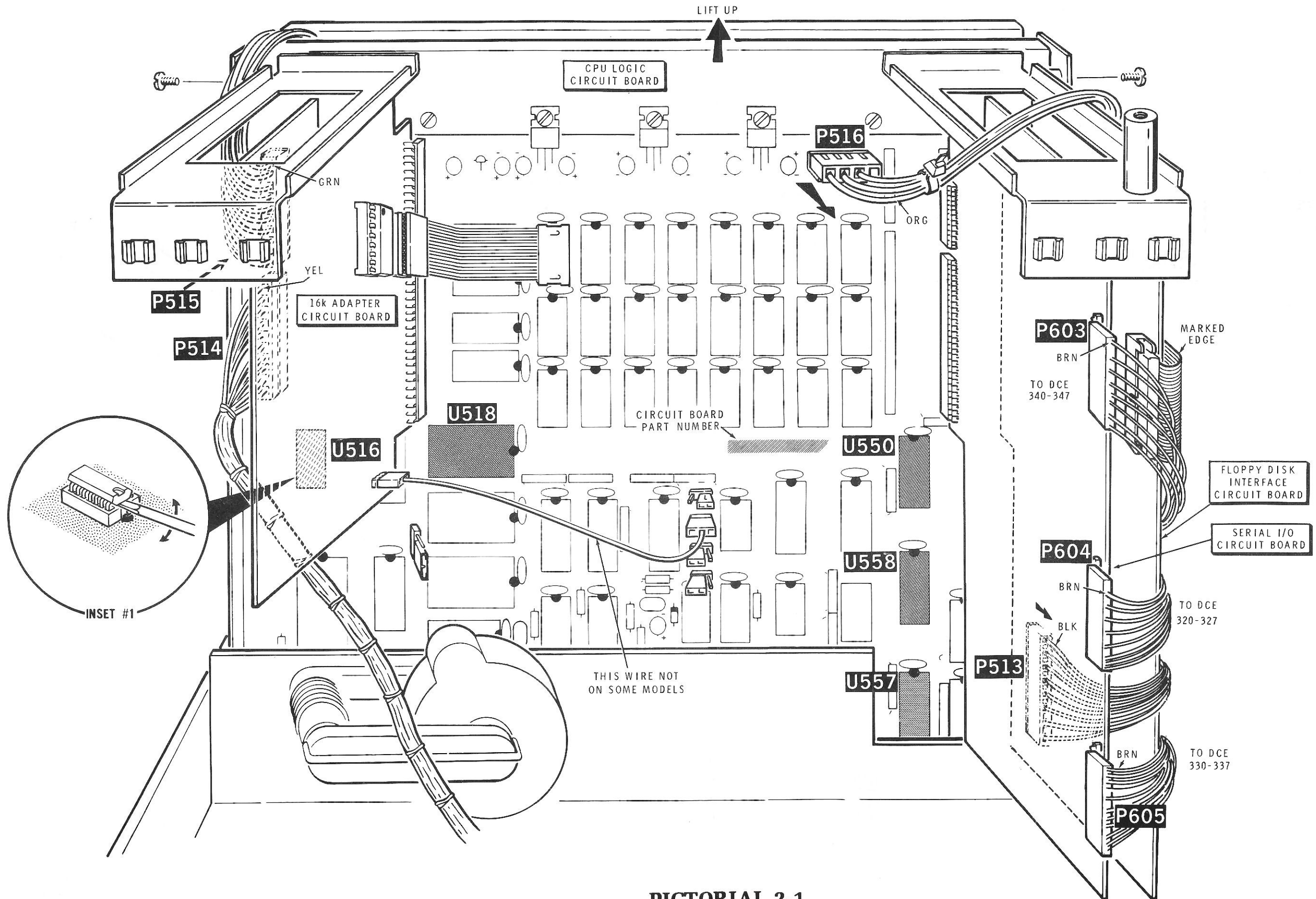
PICTORIAL 2-1
