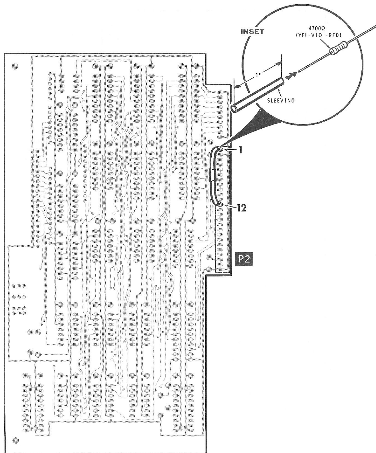
PICTORIAL 2-6
