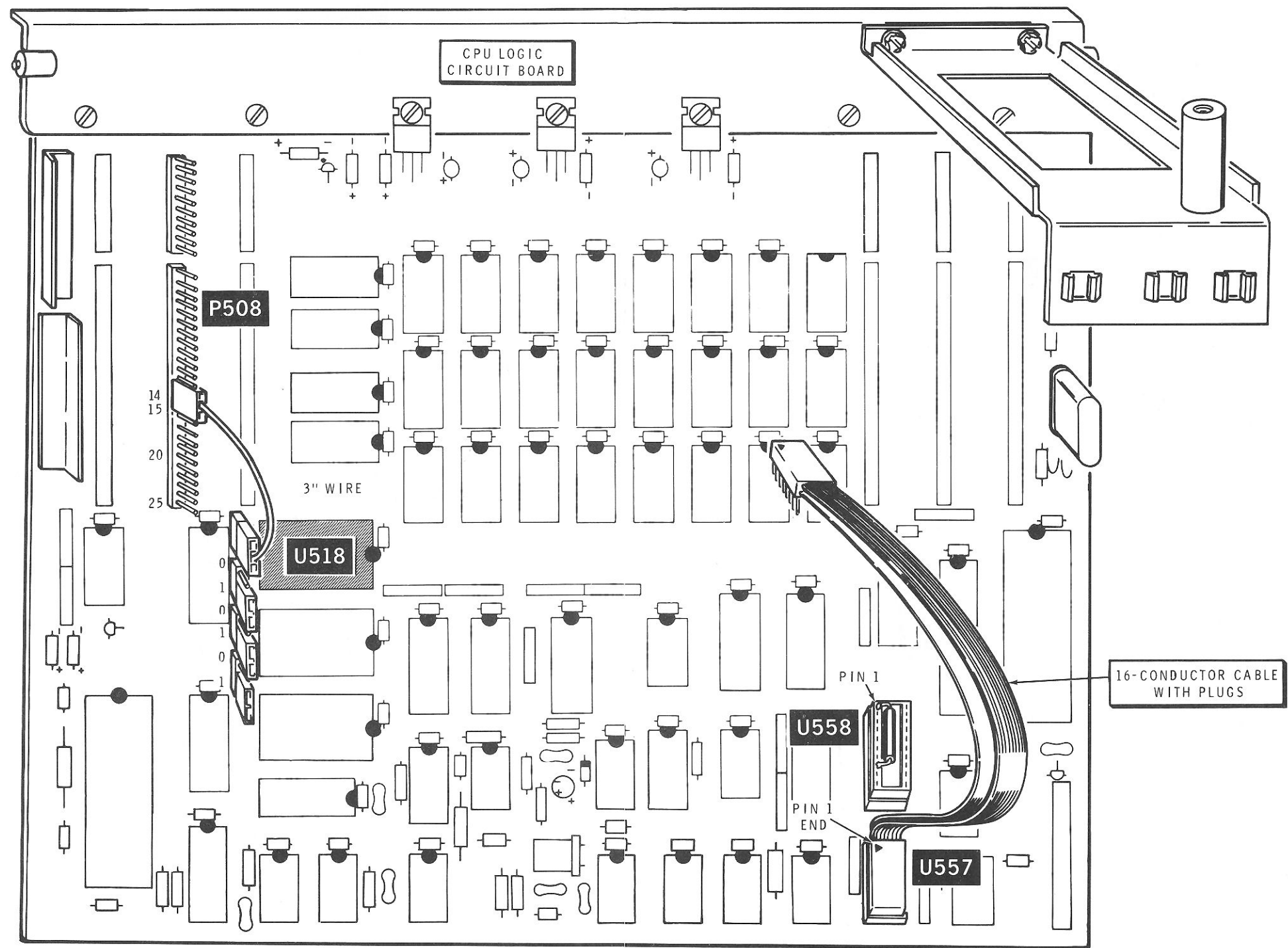
PICTORIAL 2-4
