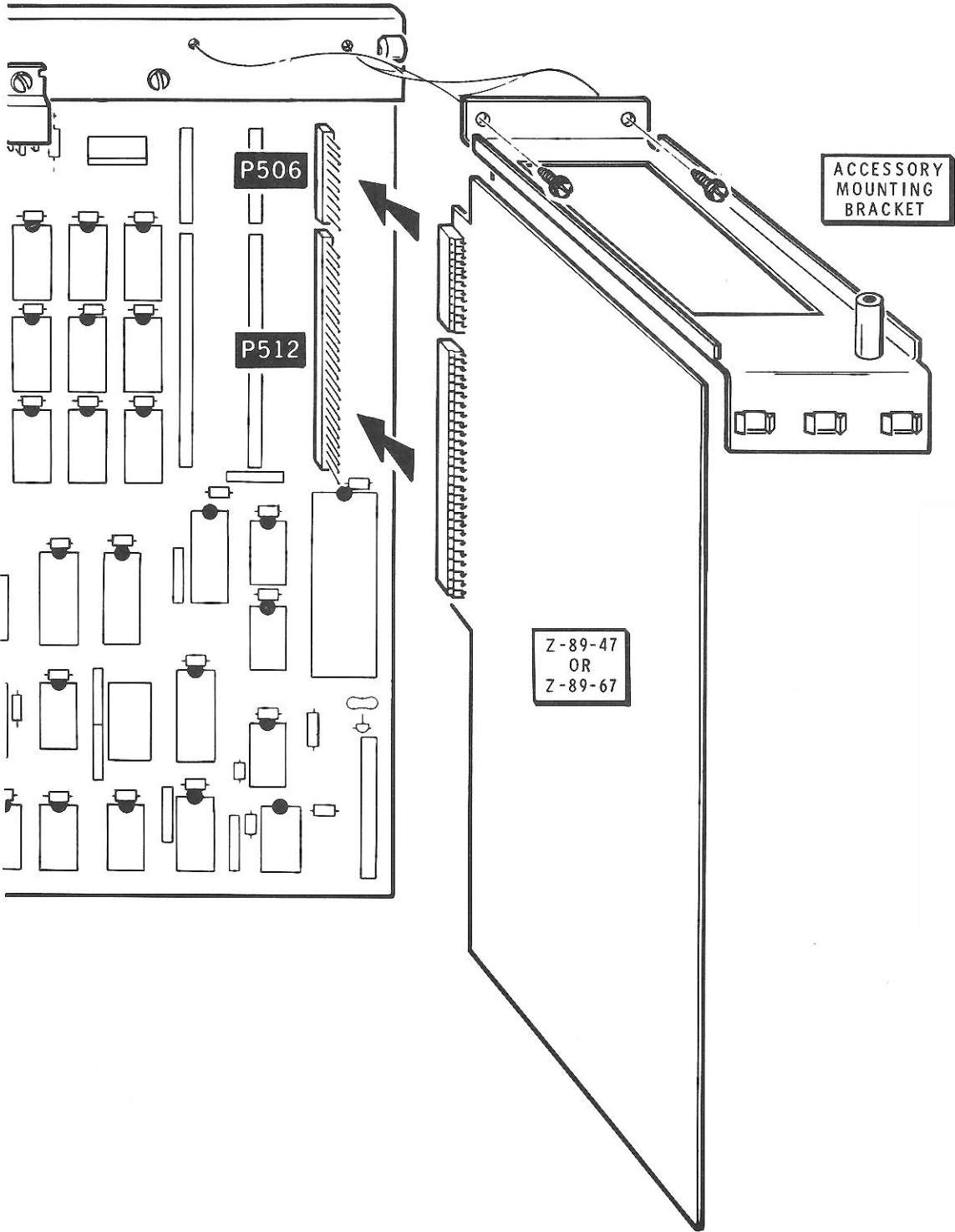
PICTORIAL 2-7
