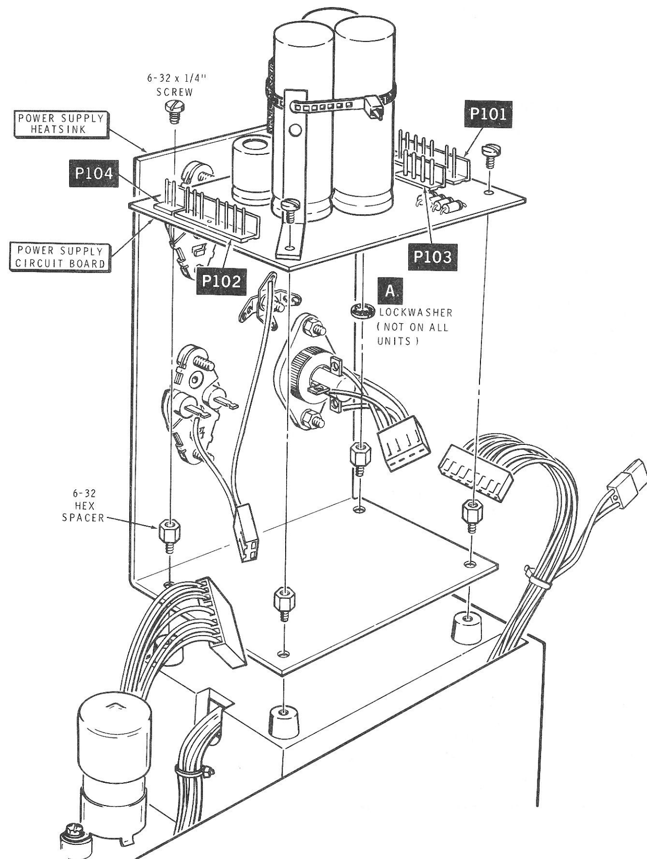
PICTORIAL 2-2
