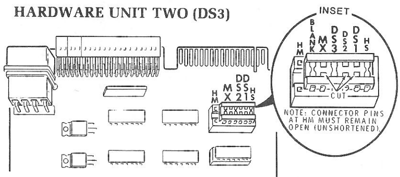
PICTORIAL 2-13
