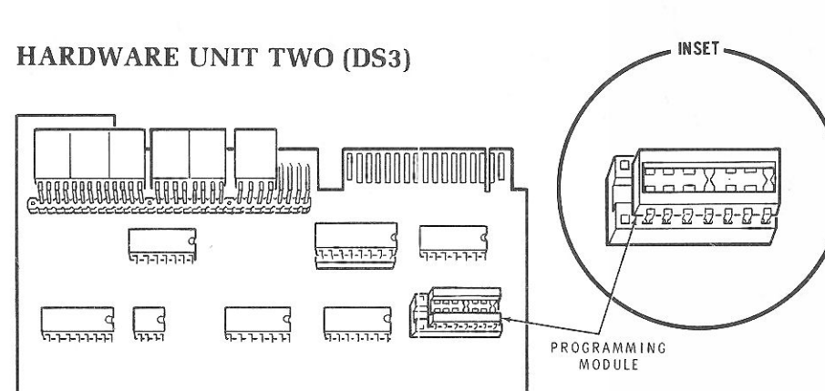
PICTORIAL 2-14
