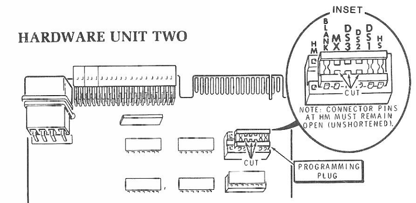
PICTORIAL 2-15
