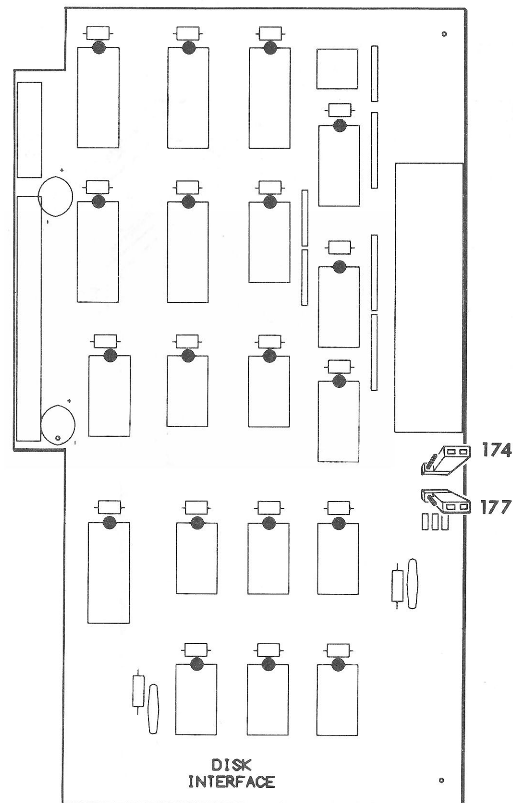
Detail 2-6A
