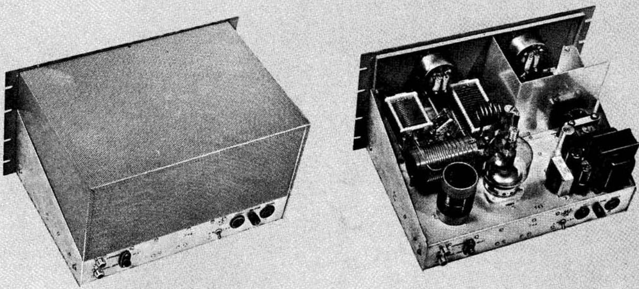
Eimac 4-250A radial-beam power tetrode amplifier stage of Globe King 500 showing circuit and RF shielding details. (Photo courtesy of World Radio Laboratories)
