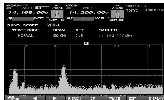
[F6(TRACE)] Key
