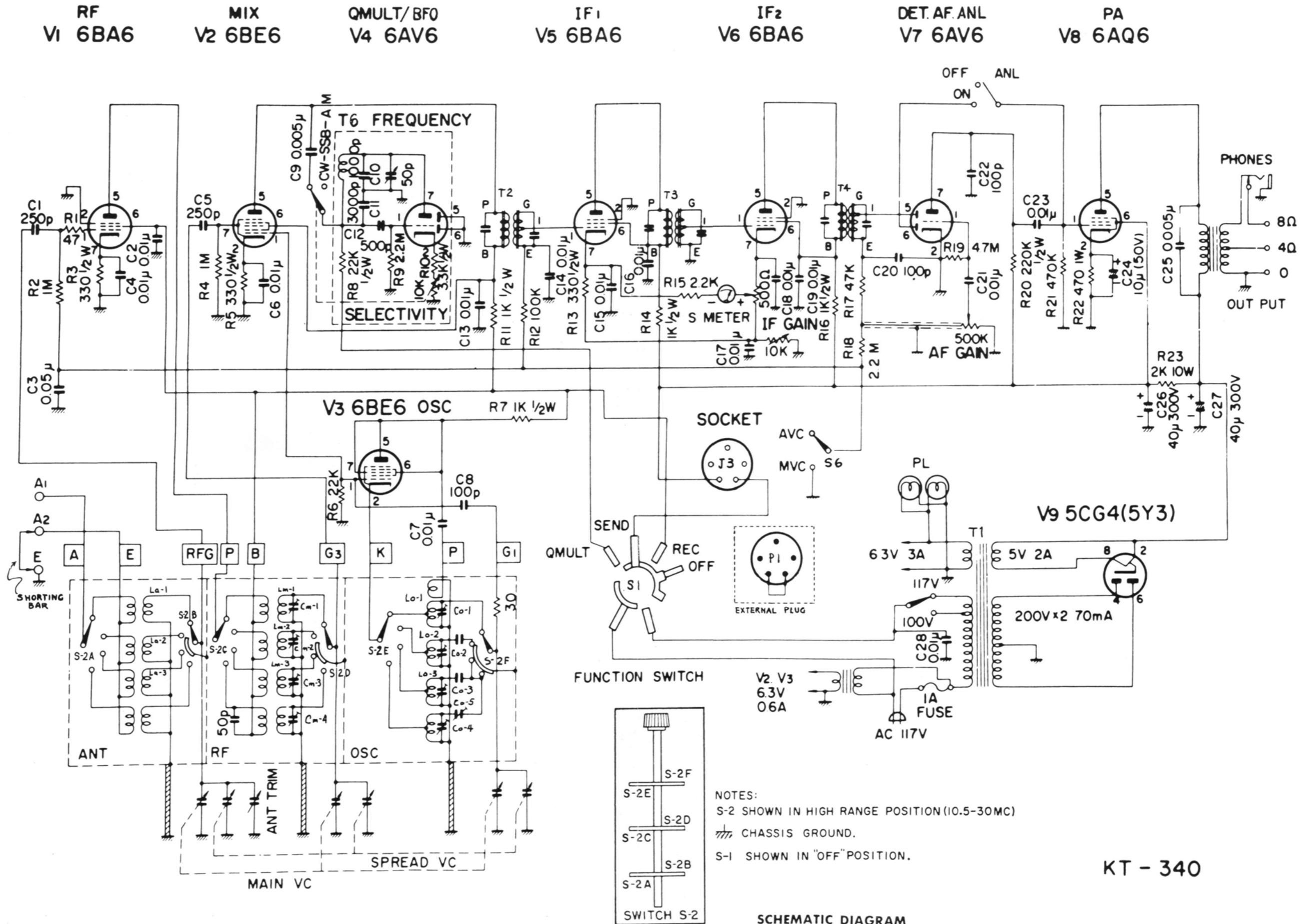
SCHEMATIC DIAGRAM
