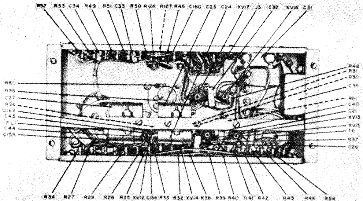
Figure 71. Speech amplifier subassembly, bottom view, A model transmitters.
