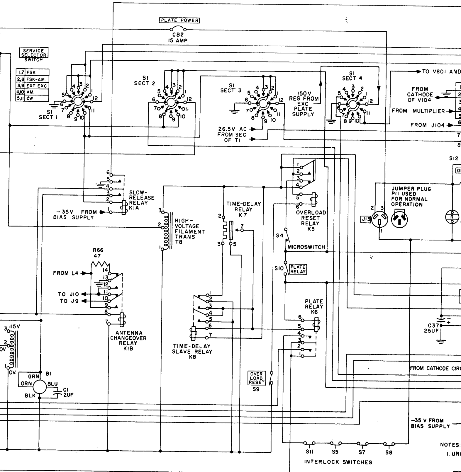
Figure 28. Primary power distribution and control circuits, basic model transmitters.
