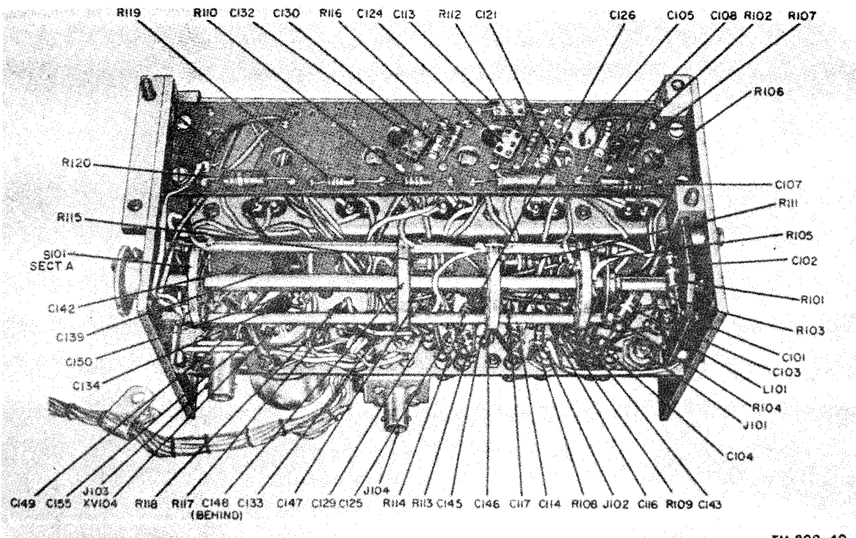
Figure 51. Multiplier subassembly in basic model, bottom view.
