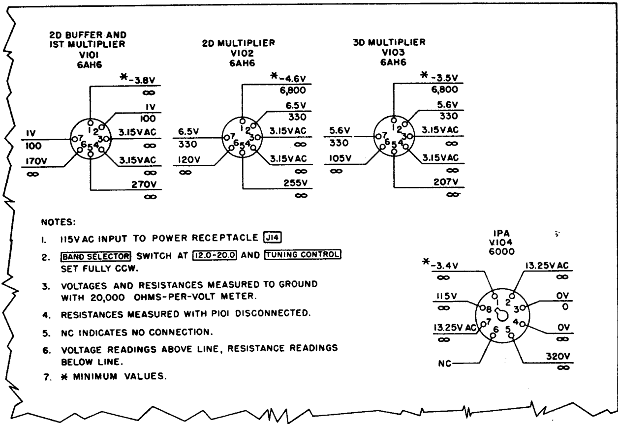
Figure 54. Multiplier subassembly, V101 through V104, voltage and resistance data.
