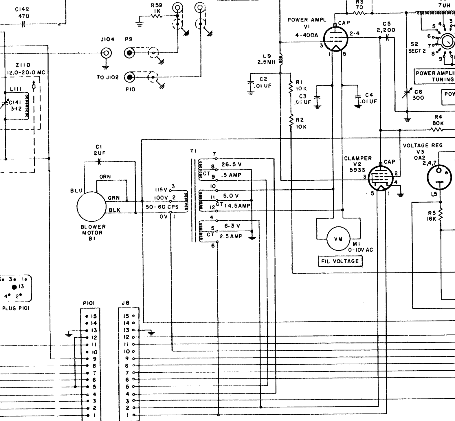
Diagram of RF deck.
