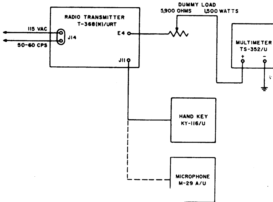
Figure 104. CW overload relay adjustment test setup.
