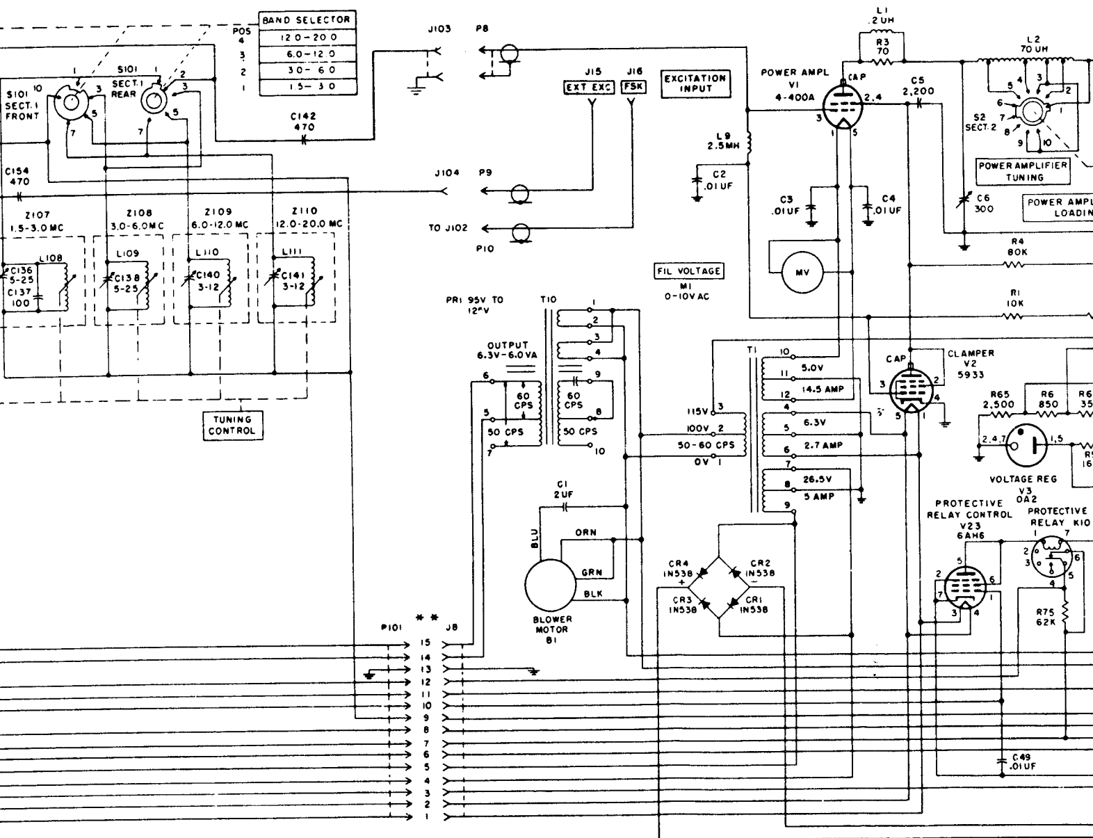
Figure 102. (Added) E model transmitters, rf deck, schematic diagram.
