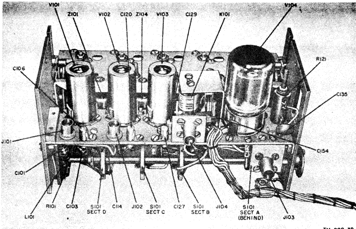
Figure 50. Multiplier subassembly, side view.
