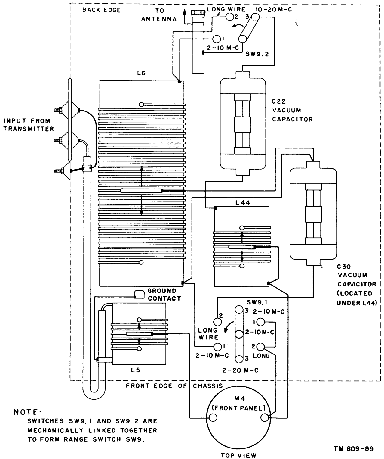
Figure 94. Antenna tuning unit, practical wiring diagram.
