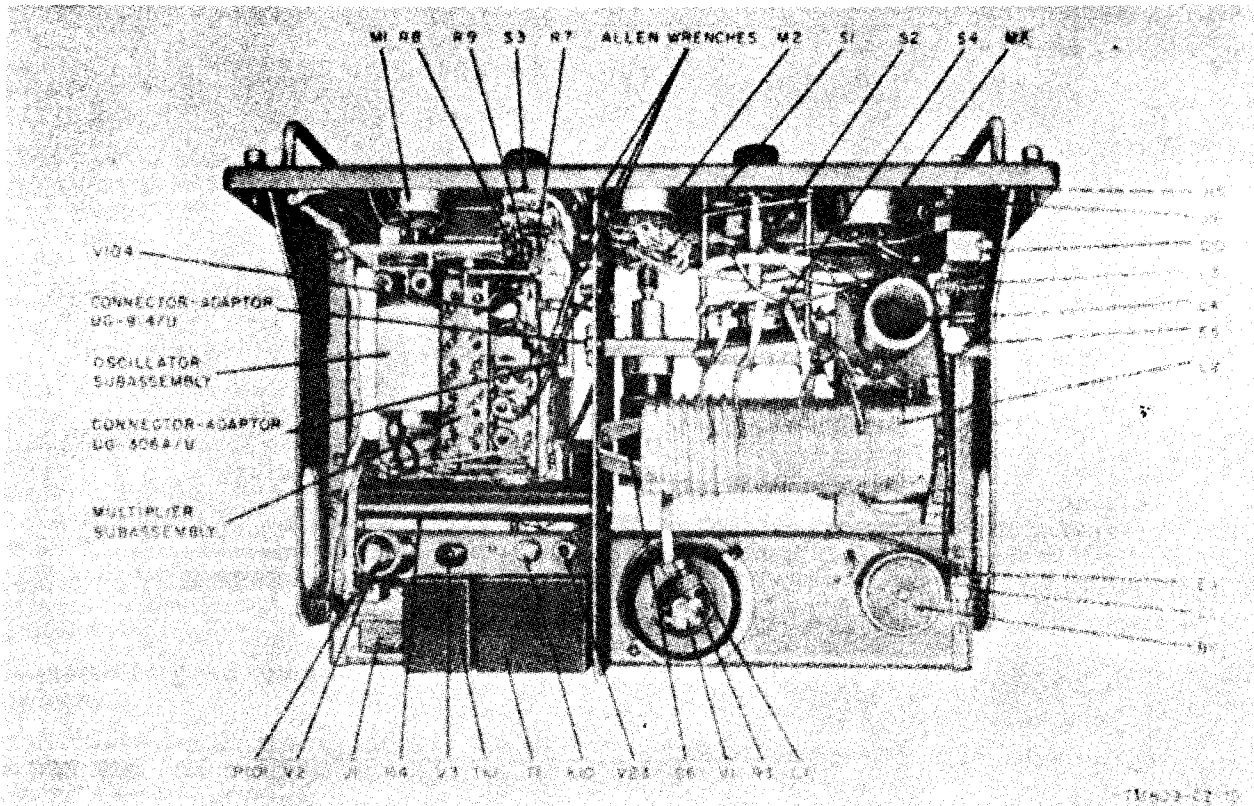
Figure 41. RF deck of C model transmitters procured in Order No. 28459-Phila-53, top view.
