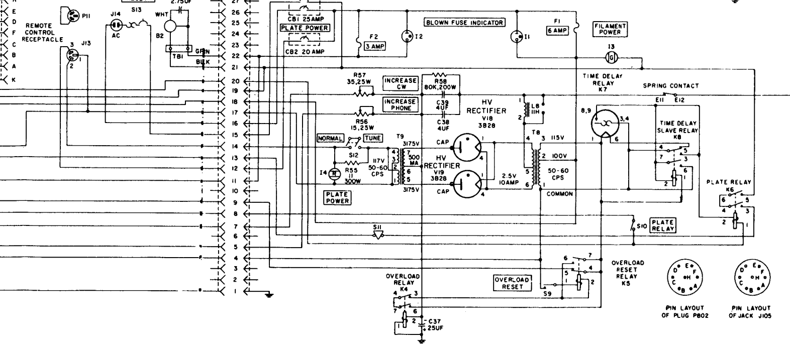
99. A model transmitter, complete schematic diagram.
