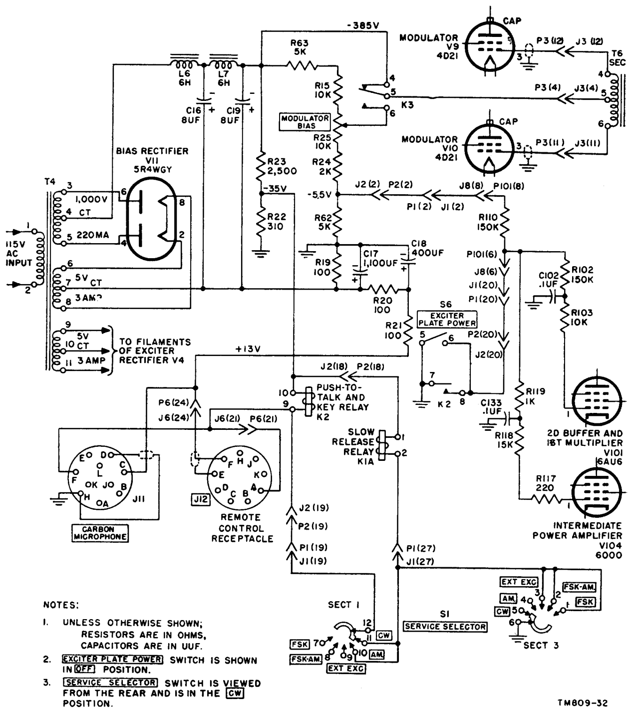
Figure 20. Bias power supply and distribution, basic model transmitters.
