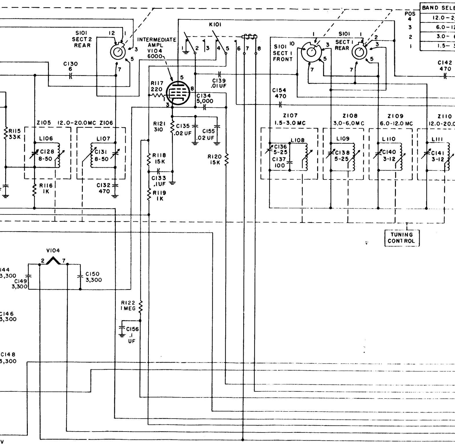
Figure 100. Band C model transmitters, schematic diagram.
