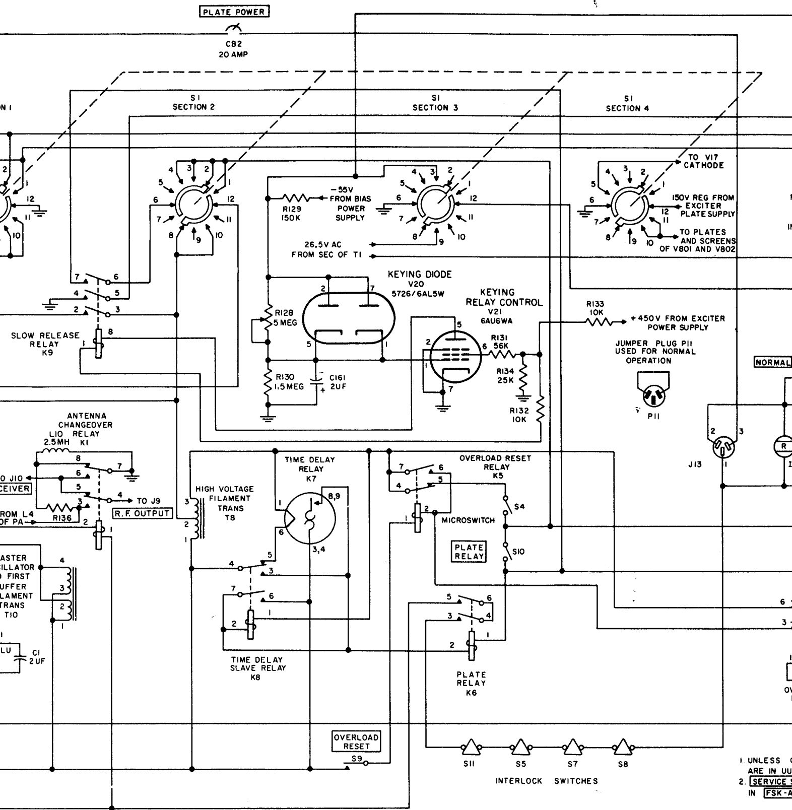
Figure 29. Primary power distribution and control circuits, A model transmitters.
