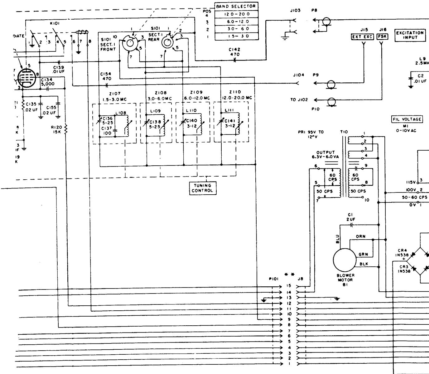
Figure 102. (Added) E model transmitters, rf deck, schematic diagram.
