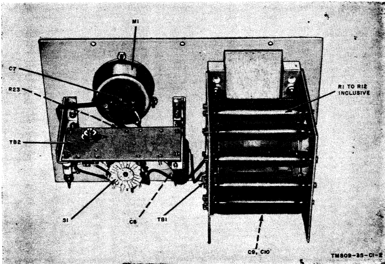
Figure 95.1. (Added) Standing wave ratio-power meter ME-165/G, interior view.
