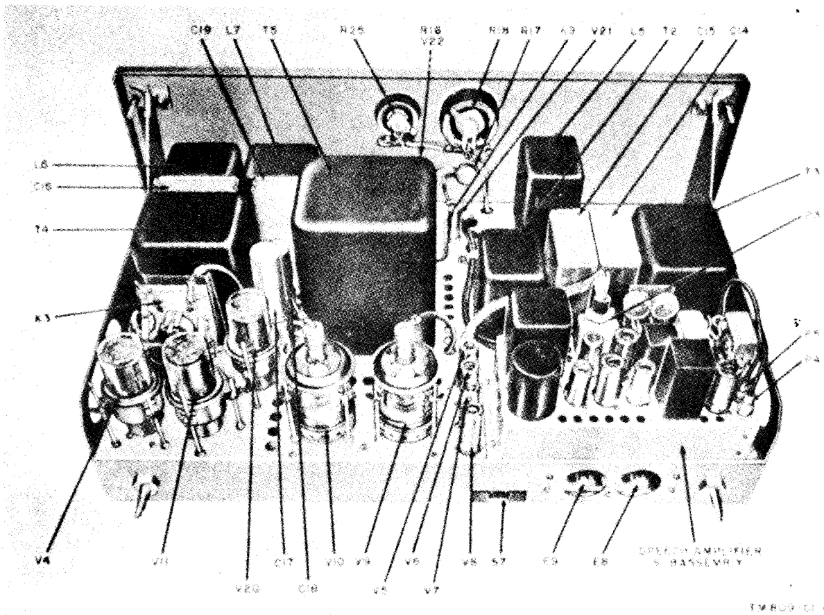
Figure 61. Modulator deck, top view, B model and C model transmitters on Order No. 49056-Phila-56.
