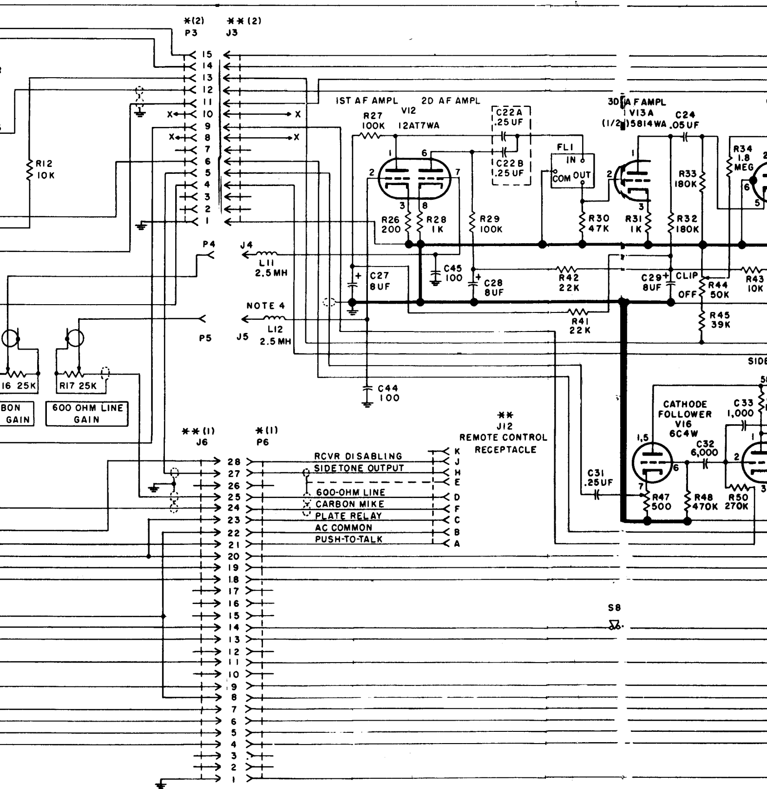
Figure 101. B and C model transmitters, schematic diagram of modulation section
