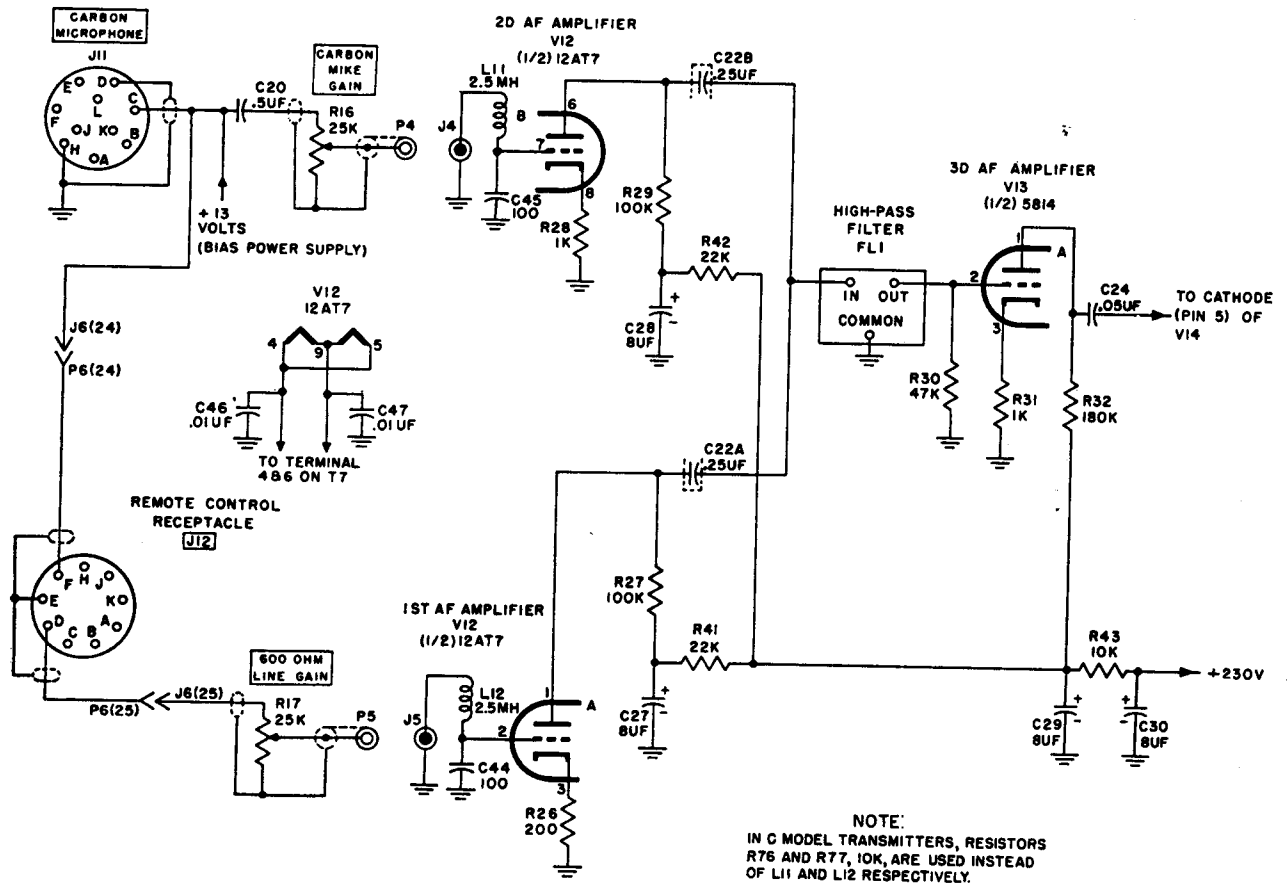
Figure 11. First, second, and third AF amplifier stages, basic, B, and C model transmitters.
