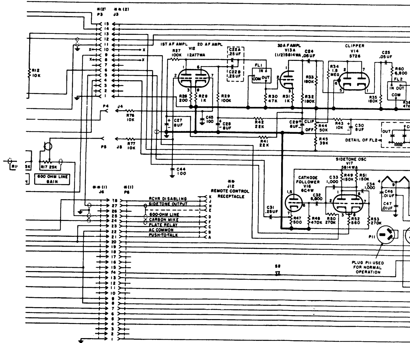
Figure 108. (Added) E model transmitters, modulator deck, power deck, and housing, schematic diagram.
