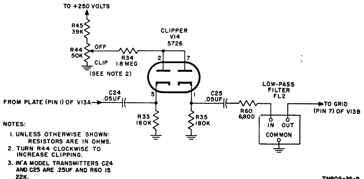
Figure 13. Clipper stage, functional diagram.
