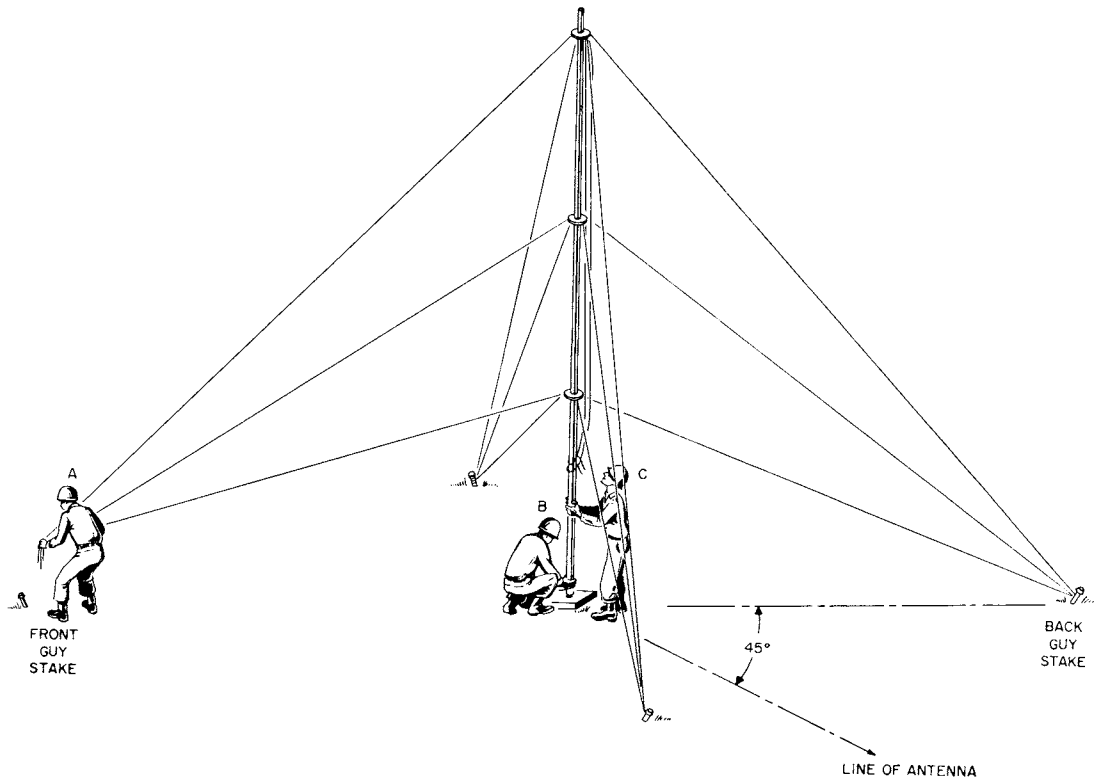
Figure 21. Raising the assembled antenna mast.
