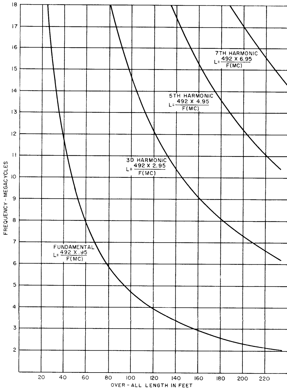
Figure 18. Graph of antenna wave length versus frequency.
