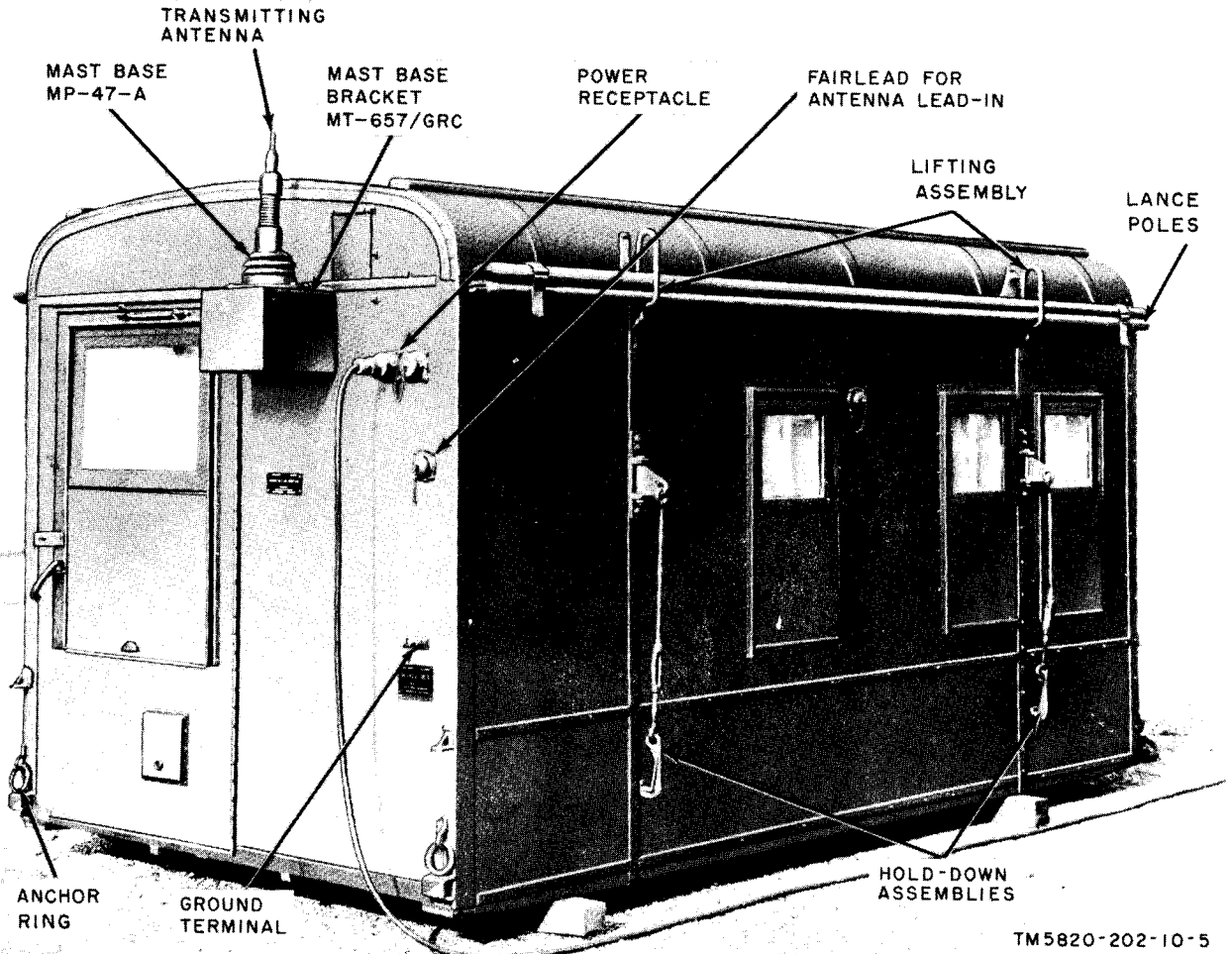
Figure 5. Shelter S-69/GRC, rear oblique view.
