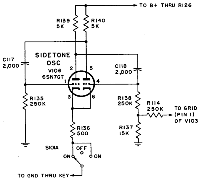
Figure 12. Sidetone oscillator and buffer, schematic diagram.
