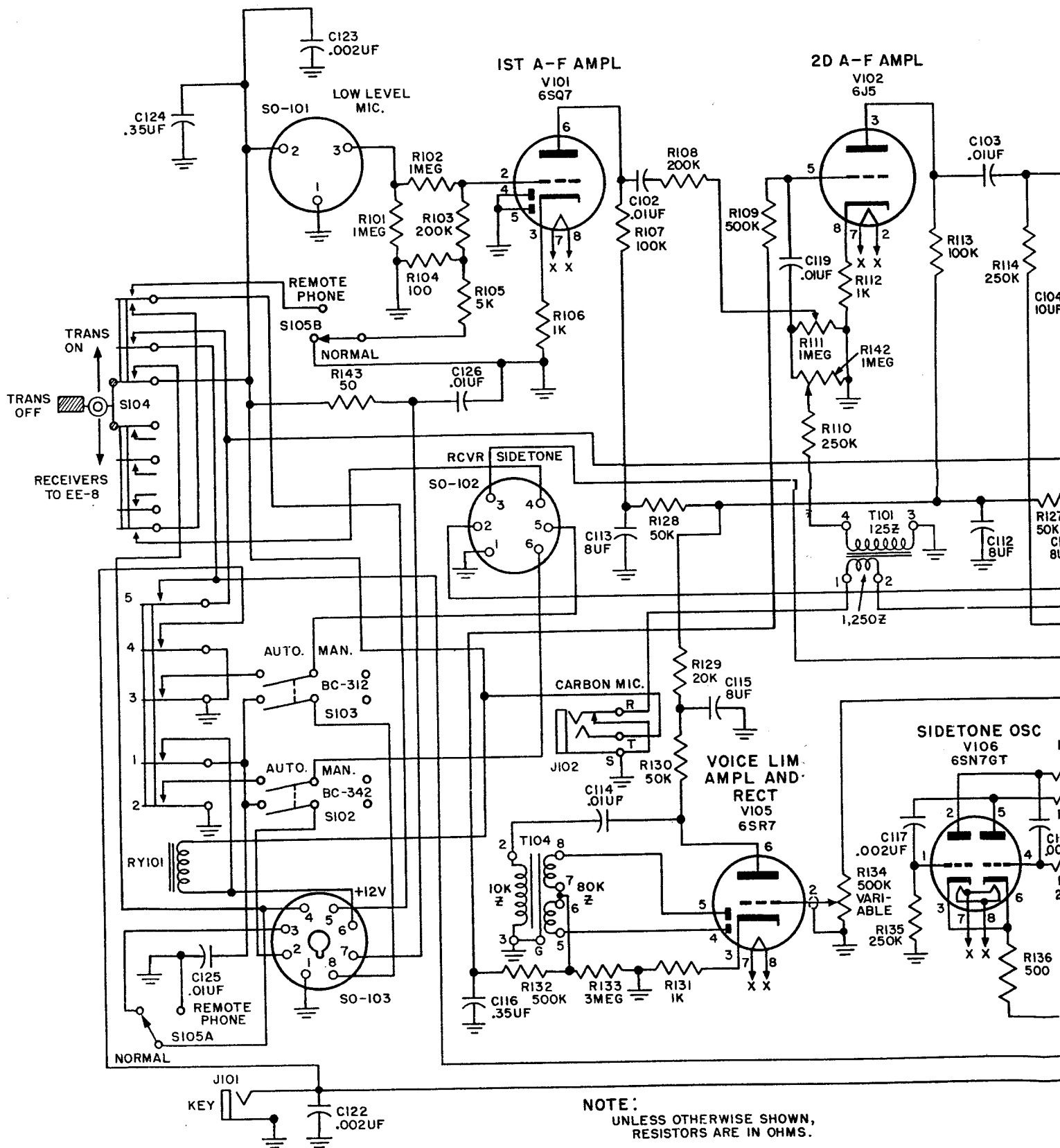
Figure 28. Speech Amplifier BC-614-F, schem
