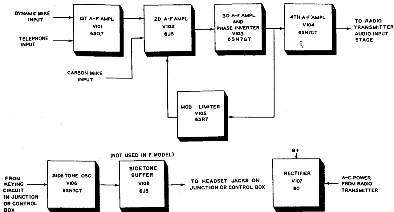
Figure 8. Speech Amplifier BC-614-(*), block diagram.
