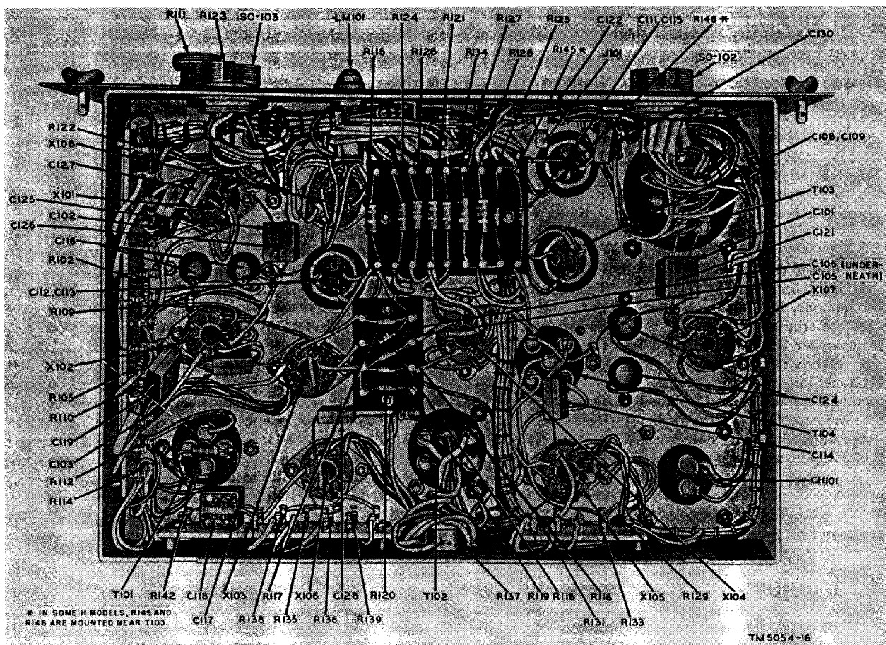
Figure 18. Speech Amplifiers BC-614-H and -I, bottom interior view of chassis.
