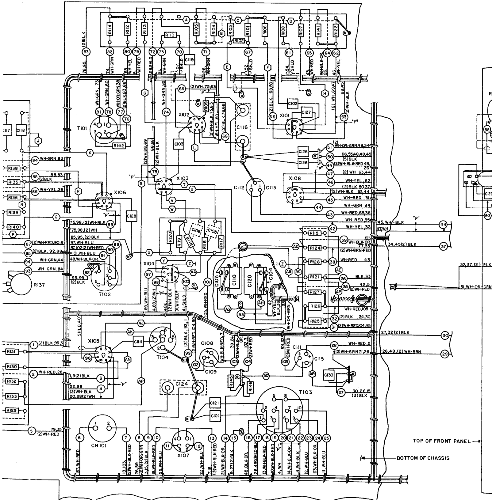
Figure 30. Speech Amplifier BC-614-H, wiring diagram of
