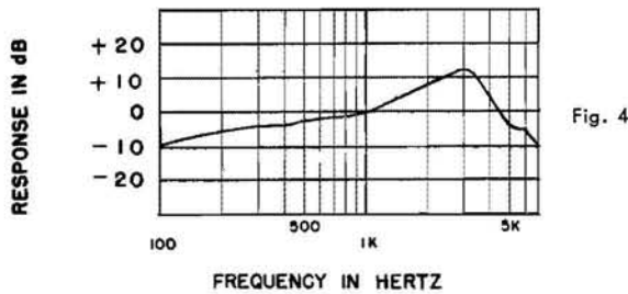
TYPICAL D-104 RESPONSE - FREQUENCY CHARACTERISTICS
