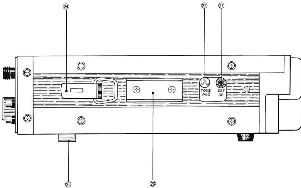
Fig. 3 Side Panel
