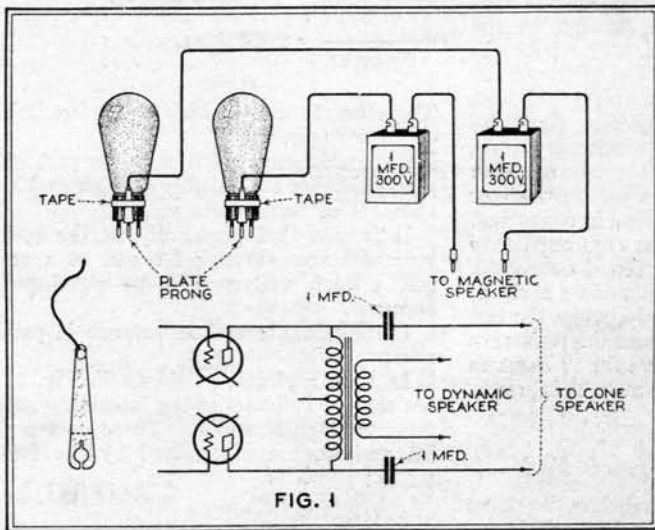
A. J. Barron, of Shawnee, Oklahoma, shows how to wire a magnetic speaker to a receiver also using a moving coil reproducer
