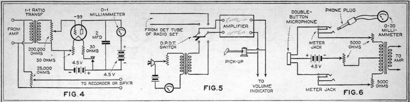
Figs. 4, 5 and 6 show respectively the circuit for a visual volume indicator, microphone-amplifier-pick-up circuit and the connections to be used for double-button microphone
