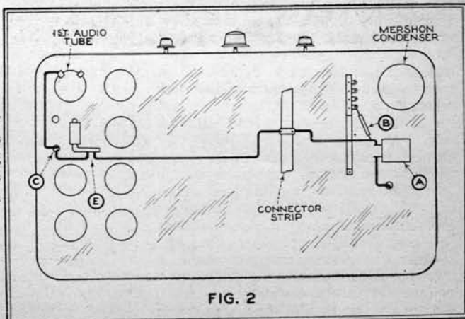
Servicing the Crosley Showbox. (The letters shown in the drawing are referred to on this page in the item from Mr. Licht)
