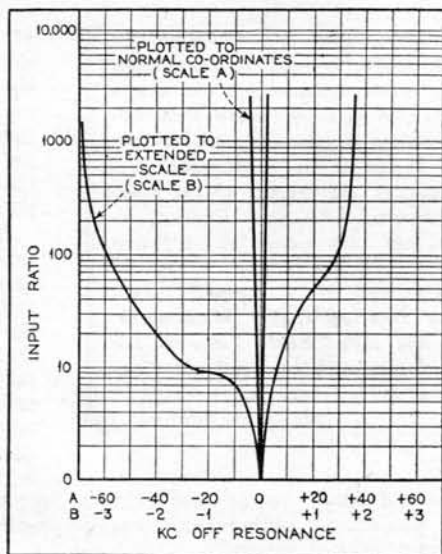
Fig. 3. (Above) Selectivity curves of the Stenode receiver. Curve A is plotted to co-ordinates accepted as standards. Curve B is plotted to an extended scale to show the shape of the tip of Curve A. These curves were taken at an arbitrary frequency of 1,000 k.c., but the figures applied to any frequencies within the range of any receiver
