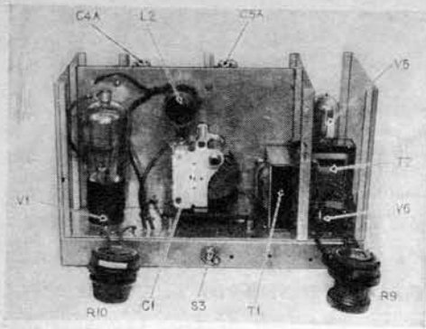
This photograph shows the tuning condenser of the oscillator circuit mounted in place before the coils have been included in the assembly
