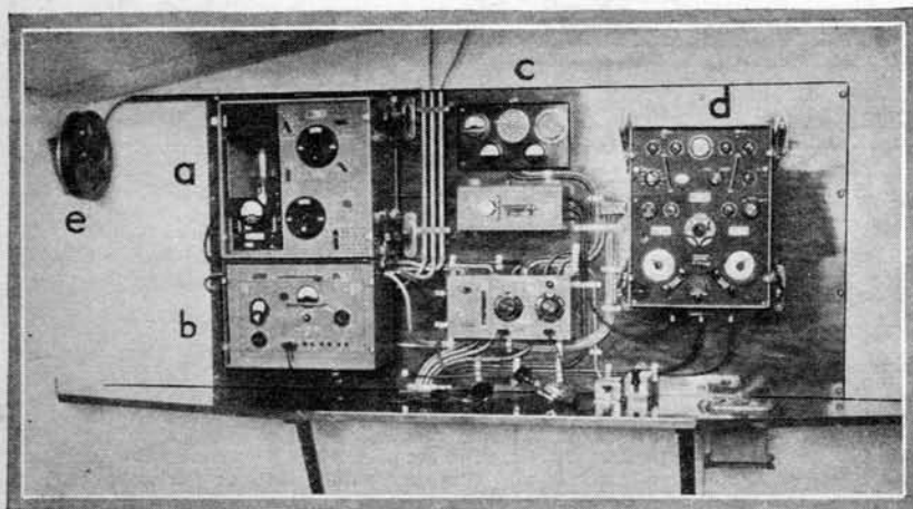
The radio cabin aboard the giant airliner DO-X. "A" shows the long-wave transmitter; "B" the short-wave transmitter; "C" the switchboard and indicator instruments; "D" the all-wave receiver, and "E" the reel for the trailing antenna
