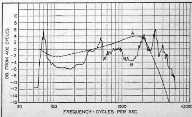
Fig. 4. Fidelity curves of the Stenode receiver. Curve A is measured at the loud speaker terminals. Curve B is that of the loud speaker measured alone. From these two curves, a general idea of the overall fidelity of the complete receiver may be obtained
