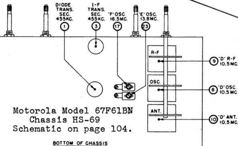
BOTTOM OF CHASSIS
