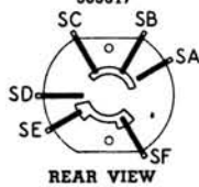
REAR VIEW
