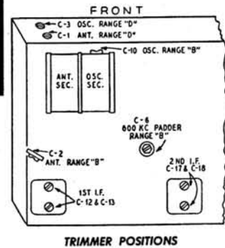
TRIMMER POSITIONS
