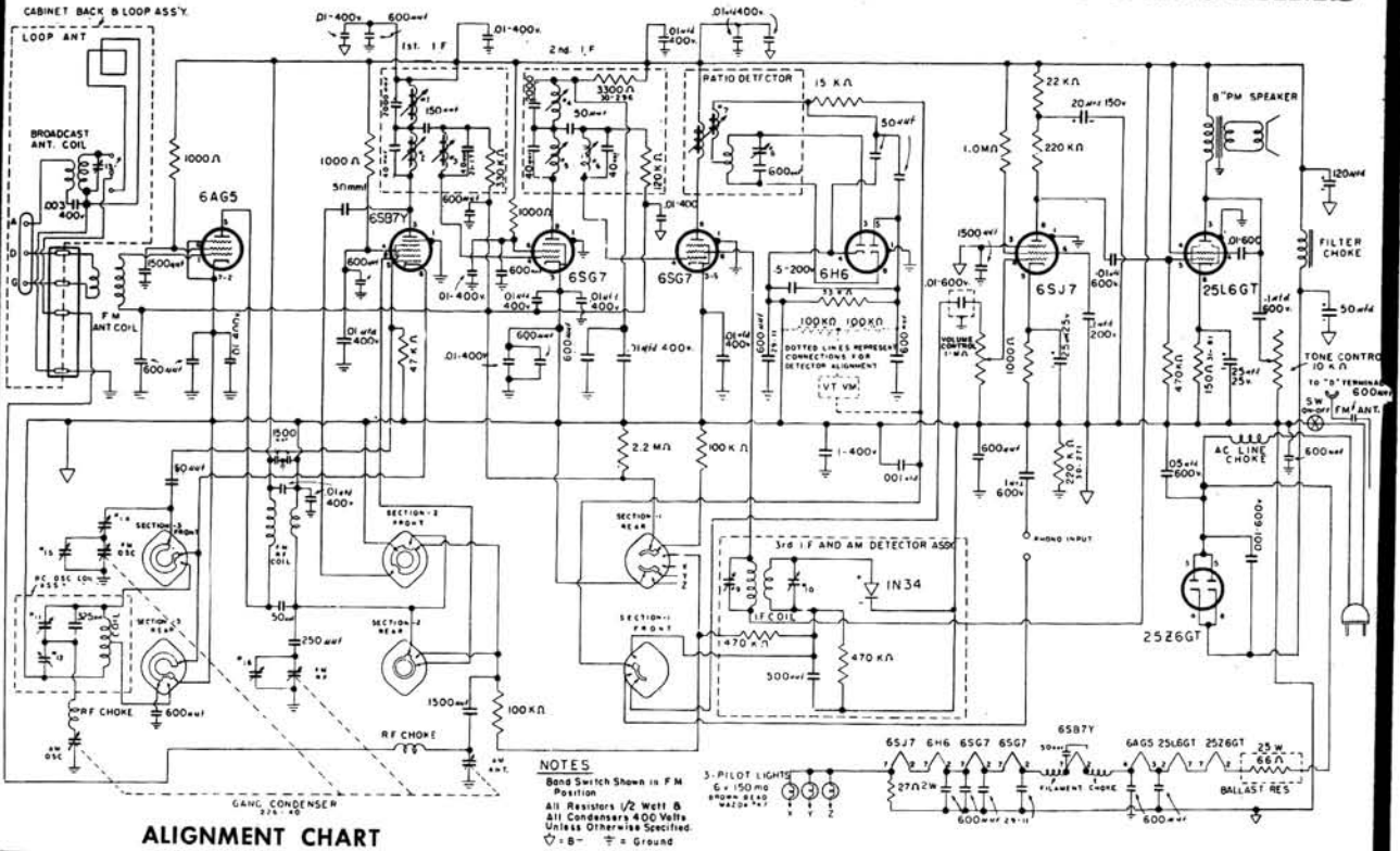
ALIGNMENT CHART
