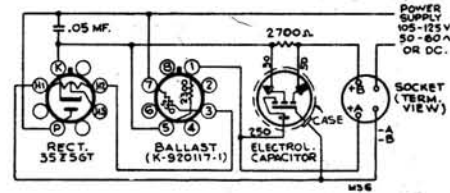
Electrifier Schematic
