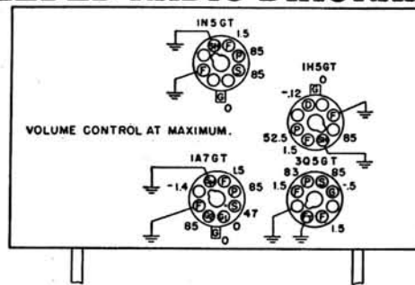
BOTTOM VIEW OF CHASSIS
