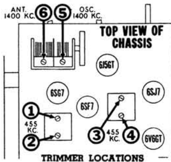
TRIMMER LOCATIONS
