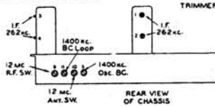
TRIMMER LAYOUT
