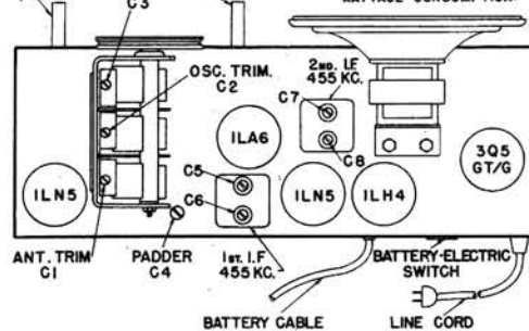
TOP VIEW OF CHASSIS
