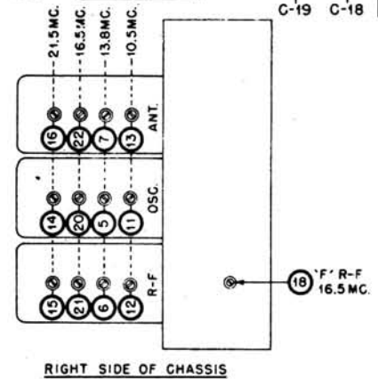
RIGHT SIDE OF CHASSIS
