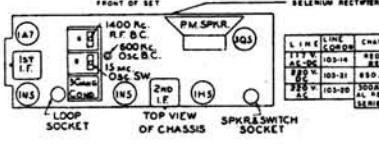
TRIMMER LAYOUT
