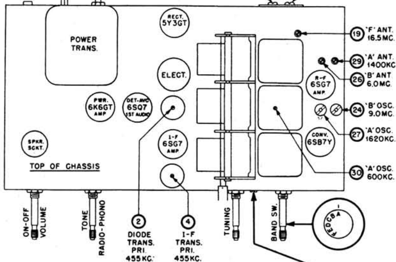
PARTS LOCATION DETAIL
