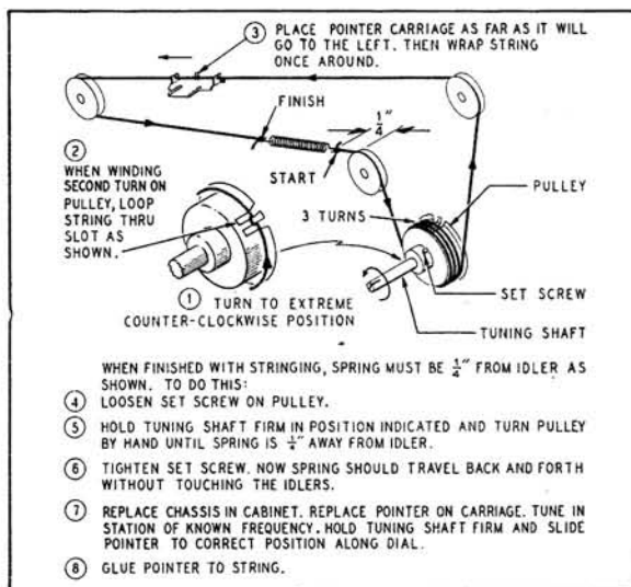
Replacement of Drive Cord
