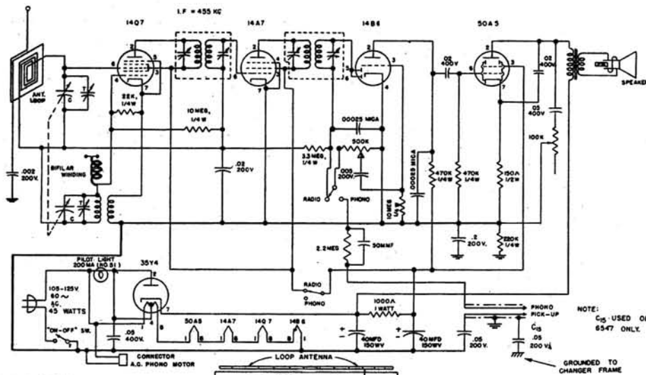
TUBE COMPLEMENT
