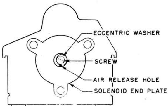
FIGURE 3. AIR RELEASE ADJUSTMENT
