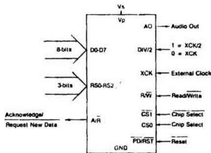
Signal Diagram
