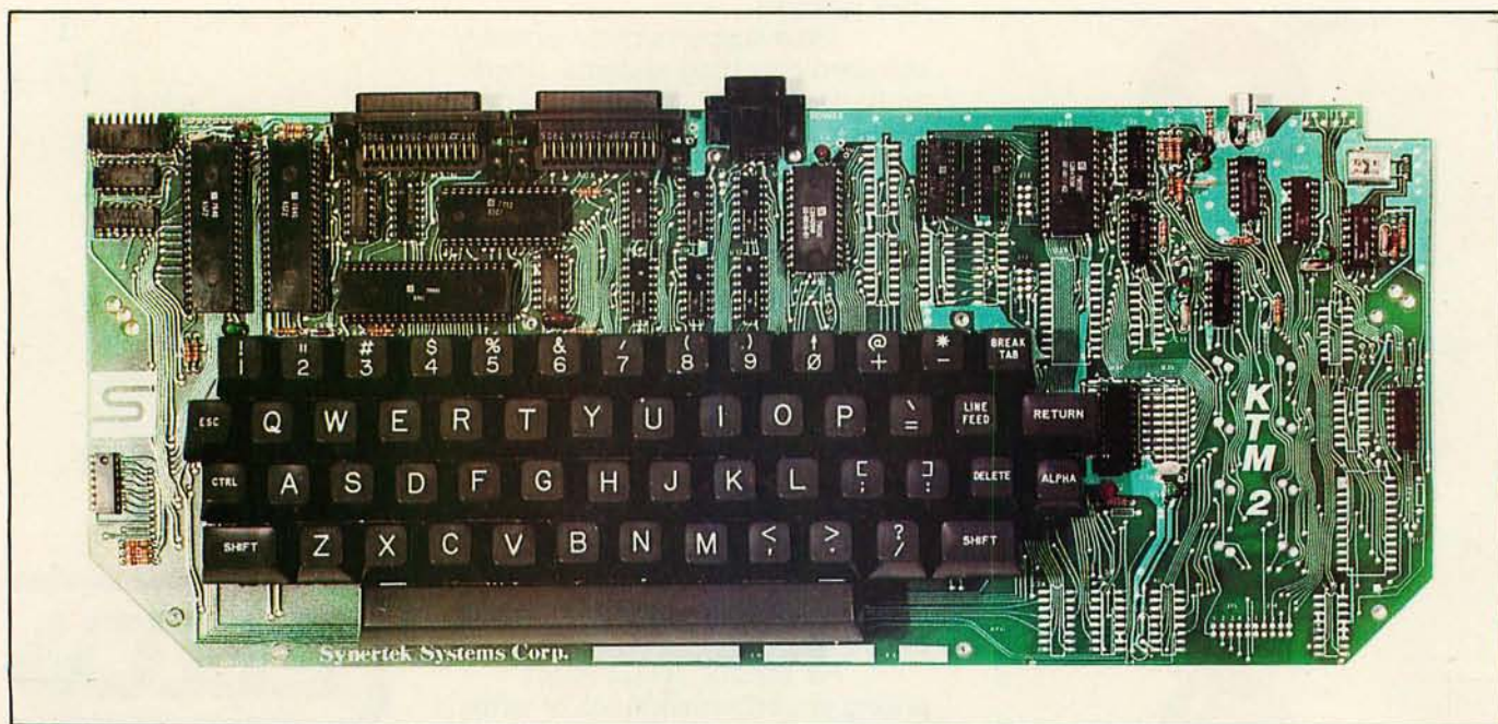
Photo 1: The KTM-2 board. The board contains a 54-key array, with all the circuitry necessary for composite-video output. This 40-character per-line version requires 1.4 A at 5 V. The 80-character version draws 1.6 A. Both are able to provide RS-232-compatible outputs with the addition of extra power supplies.
