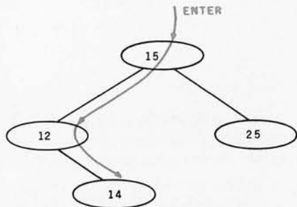
Figure 4: Adding to a binary tree. The colored arrow shows the direction of search when placing a new node in a binary tree. Here, 14 is greater than 12, so it is placed as a right child of 12. Here, the sorted order is 12, 14, 15, 25.
