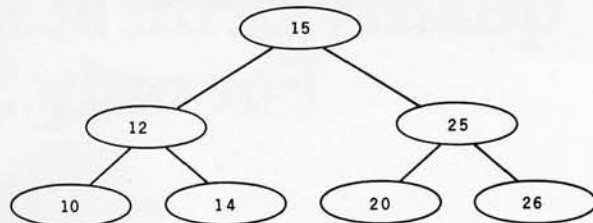
Figure 5: Example of a binary tree. Here, more nodes have been added, giving the sequence 10, 12, 14, 15, 20, 25, 26.
