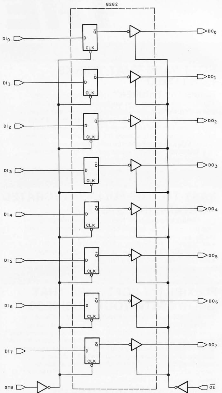
Figure 2: The 8282 8-bit buffer/latch. Similar to the familiar 8212, the 8282 has a greater drive capacity and comes in a narrower, twenty-pin dual-in-line package.
