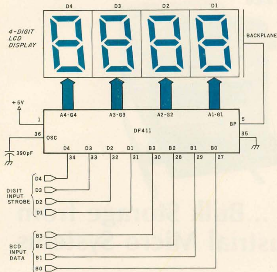
Figure 6: A four-digit LCD driver circuit, the DF411, made by Siliconix, Inc, 2201G Laurewood Rd, Santa Clara CA 95054.
