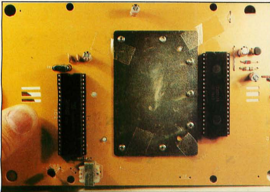
Photo 4: Rear of the printed-circuit board used in the Mego Mini-Vid game, revealing the location of the liquid crystal display shown in photo 3. The complete electronic circuitry for the game is visible. The integrated circuit on the left is an Intel/NEC 8048 8-bit microcomputer. At the right is a custom LCD dot-matrix driver component. The three sets of discrete components (clockwise from top right) are a voltage regulator, an audio amplifier, and a 6 MHz clock circuit. I bought the game on sale for $24.95.
