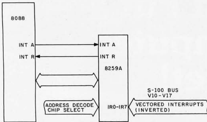
Figure 3: An 8259A Programmable Interrupt Controller can be added to the system by following this logic diagram. The 8259A requires access to the demultiplexed bidirectional data bus of the processor in order to properly interpret vectored interrupts from the S-100 bus.
