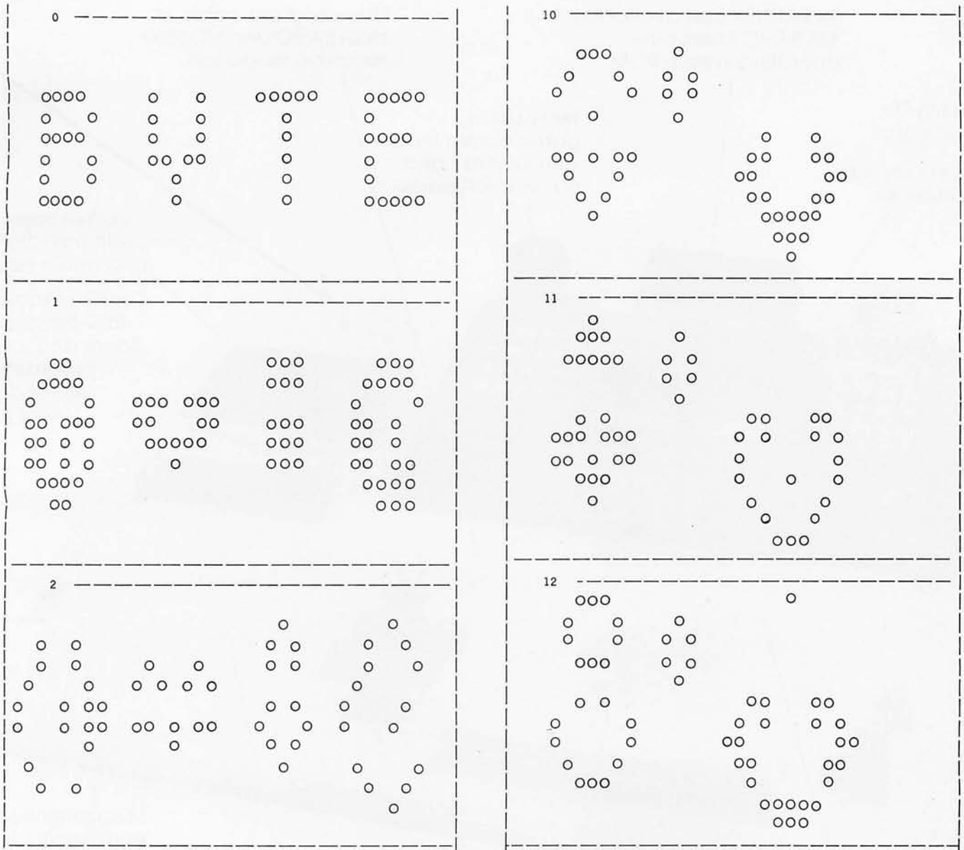
Listing 2: An example of the APL function LIFE at work. The frames shown here are from successive generations of a Life colony that begins as a collection of cells that spell the word BYTE. The generation number of each frame is shown in the upper left-hand corner.
