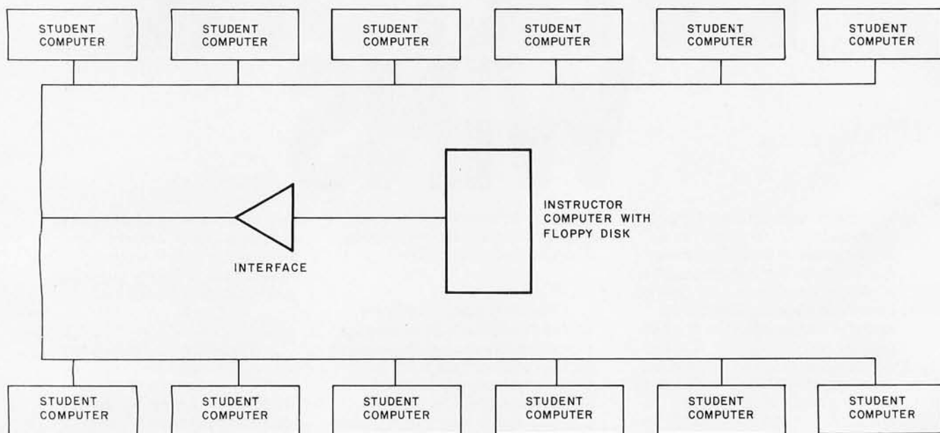
Figure 1: Block diagram of a multiple-machine loader system. The network is composed of an instructor's computer, a cable-driver interface, and up to twenty-four student computers.
