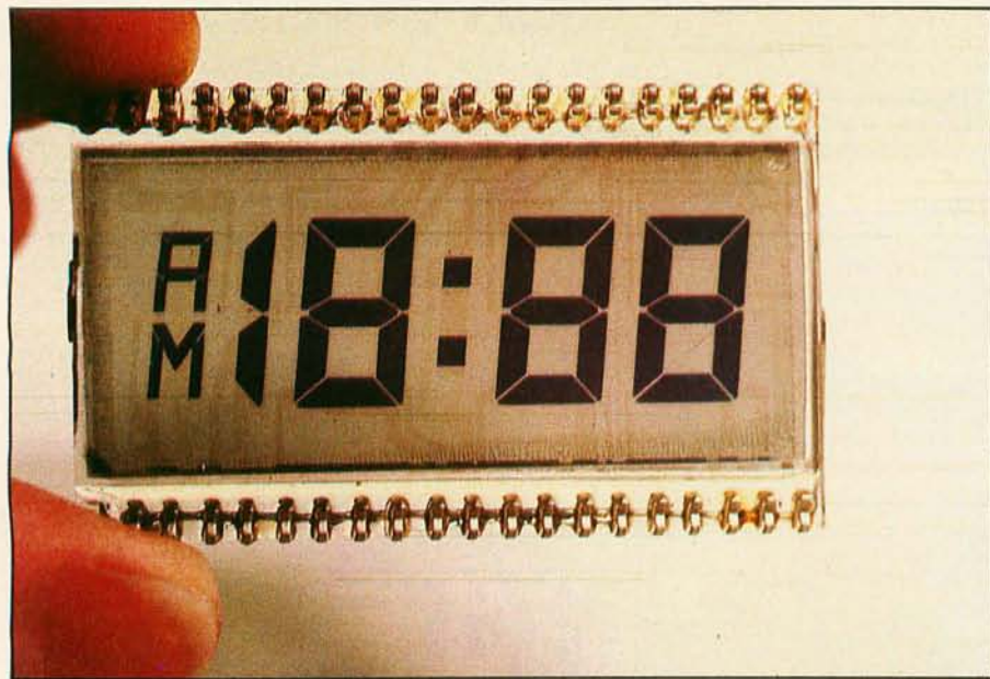
Photo 1: Standard three-and-a-half-digit clock/multimeter display. The unit shown is transmissive and has no rear reflector. All segments are energized in this photo.
