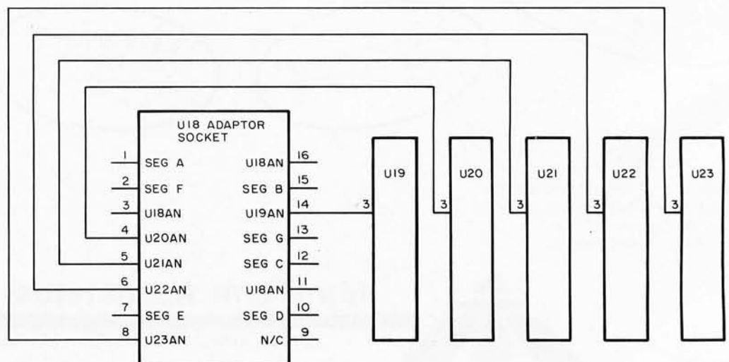
Figure 1: This diagram shows electrical connections of the 16 pin remote adaptor socket installed as U18, with patches to the pin 3 anode connections of U19 thru U23 of the KIM-1 design. The display positions of U19 thru U23 can have 14 pin sockets installed if it is desired to occasionally revert to on board displays.
