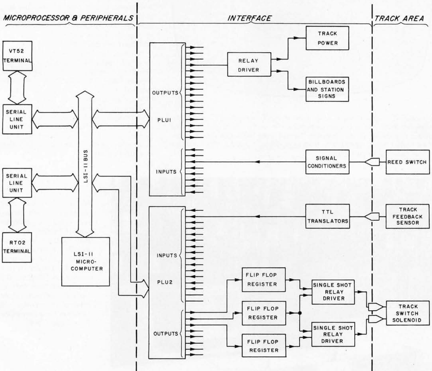
Figure 2: Block diagram of the LSI-11 control system. The data bus is connected to two terminals used to input and display information at the operator's control station. It is also connected to a special interface which is based on two hardware latches called parallel line units, or PLUs. These PLUs store command bytes coming from the microcomputer which in turn drive flip flops and relay drivers used to power the track and operate track switches. Commands from the computer are in the form of 16 bit words. Each section of the track has been assigned a specific bit, and only those bits of the word necessary to change the track sections desired will change. Information from reed switches is also latched by the PLUs and sent back to the computer to be used in closing the feedback control loop.
