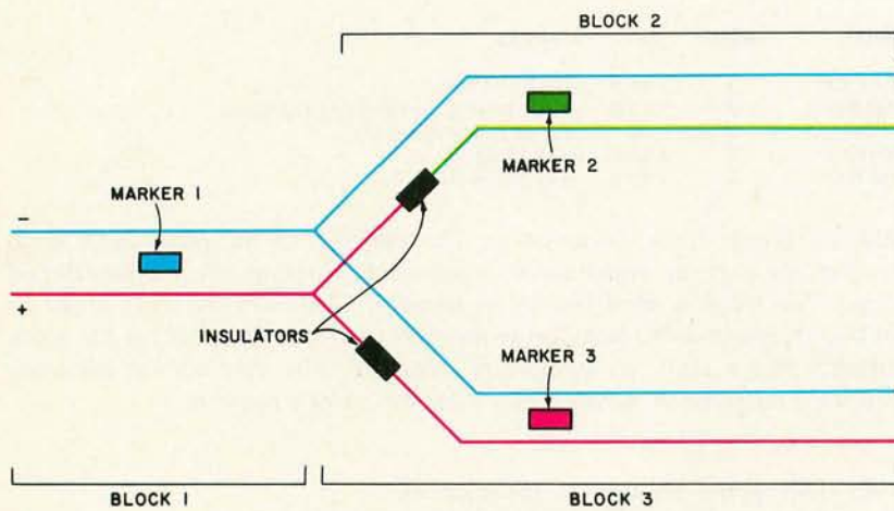
Figure 8a: An example of a marker being between two blocks. In this type of array the computer must only determine whether the train will go into block 2 or 3.
