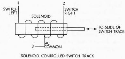
Figure 7: A turnout solenoid. This type of solenoid can be activated in either direction because of its center tapped coil. Application of voltage to the desired side of the coil determines the direction of throw.
