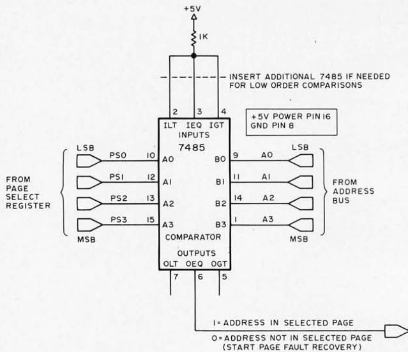
Figure 2: If a virtual memory system is implemented, there is a definite need to find out whether or not a referenced address is currently in the swapping region of memory. This can easily be accomplished by using one or more comparator chips. If the page select register is equal to the current page address reference to the swapping region, then access is normal. But if a page fault occurs (a reference to a page not presently in memory), then the paging processor is invoked while the main processor is at rest waiting for data. The 2 microprocessor strategy discussed here is but one of a number of strategies possible for implementing virtual memories.
