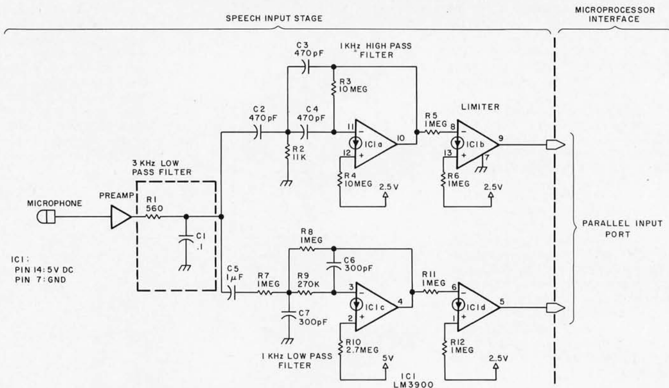
Figure 5: Speech filtering circuitry. A voice signal is picked up by the microphone and preamplified. It is then sent through a low pass filter made up of C1 and R1 whose cutoff frequency is 3 kHz. The signal is next passed through a 1 kHz high pass filter and a 1 kHz low pass filter as shown. The two signals then go to the microprocessor interface for further processing. IC1, which forms the basis for this circuit, is a quad LM 3900 op amp. The diode-like symbols shown on the four amplifiers indicate the use of "current mirrors" for the noninverting inputs. For a detailed discussion see National Semiconductor's book, Linear Integrated Circuits, page 2-250 and following.
