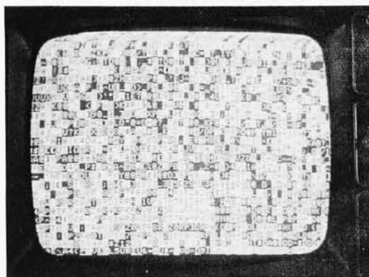
Photo 5: A garbage display field, obtained by the application of power to the memory. Each chip has a preferred start-up value, so this pattern tends to be the same whenever one turns on the display. In this picture, blanking has been suppressed, so the distortion due to non-linearities at the top of the screen is quite visible.
