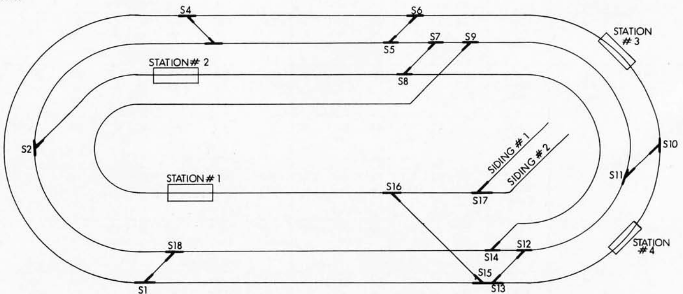
Figure 1: Model railroad track layout used in authors' system. During a typical demonstration, both trains leave their sidings under control of a Digital Equipment Corporation LSI-11 microcomputer and are routed along the tracks according to a control program in the computer. Feedback sensors are used to verify train locations at strategic times.
