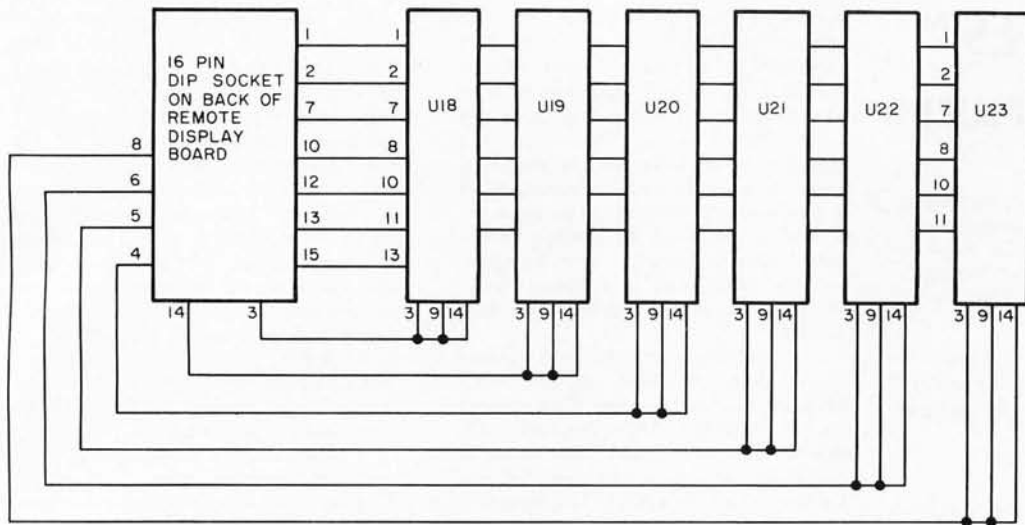
Figure 2: A remote display board. After removing the KIM-1 displays, a remote display board is constructed for mounting in a more convenient packaging arrangement. The wiring of the cable which plugs into the 16 pin socket installed at the U18 position of the KIM-1 board is listed in the diagram.
