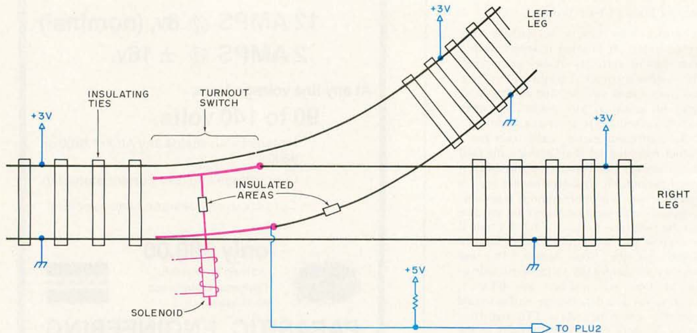
Figure 6: A typical fork (or "turnout") in the track. In this illustration, the turnout is positioned to divert the train to the left leg. These solenoid controlled mechanisms act as their own sensors. One leg of the switch is either grounded or ungrounded depending on its position. This is used to provide a logical 0 or 1 output to the computer for confirmation of the switch's position. The solenoid is illustrated in figure 7.
