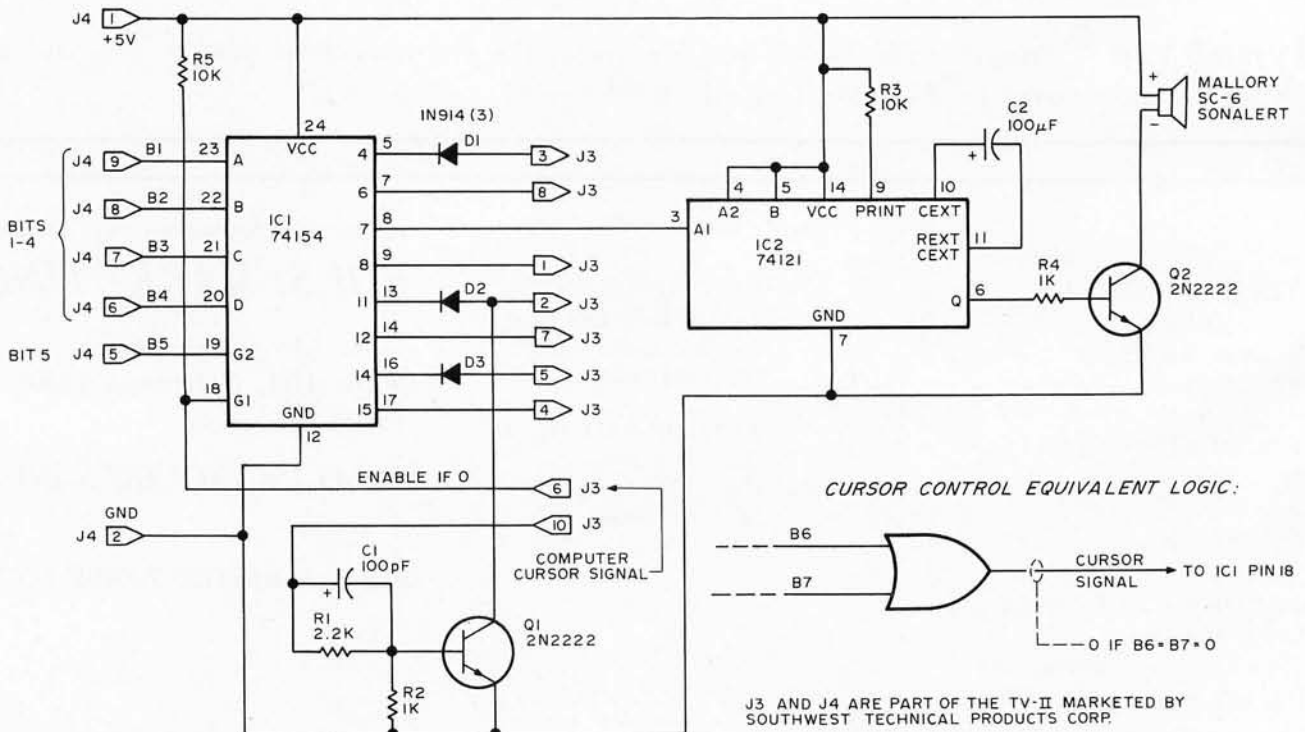
Figure 1: Diagram for the TVT II cursor controller. IC1 is a 4 to 16 line decoder that will select which control command is wanted. Transistor Q1 is in the circuit to make it compatible to the Southwest Technical Products' screen read and UART boards. Diodes D1, D2 and D3 are in the circuit to protect IC1 when it is connected in parallel to the output of a gate on the main TVT II board. IC2 is wired as a one shot to activate the SonaAlert when a control G is pressed.
