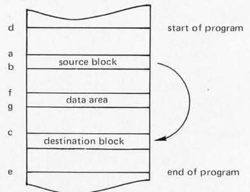
Figure 1: A special case in program relocation. The program block a thru b is to be moved to location c, but the integrity of the data block from f thru g must be preserved. The technique in this case is to change program references in two passes: up to, but not including, the data block, and then after the block. Locating all data at the end of programs will of course prevent this type of problem.
