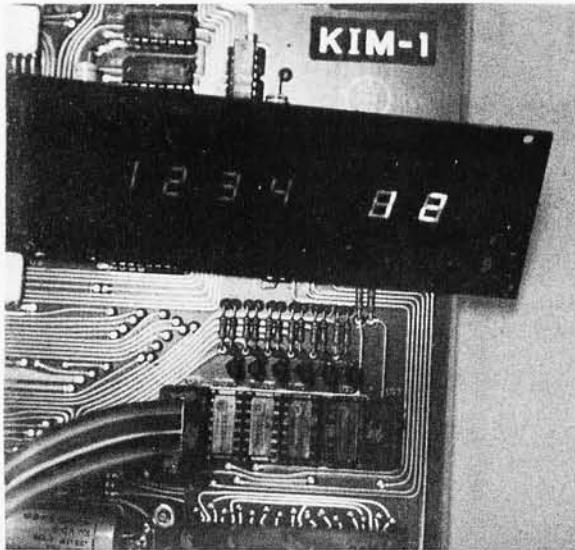
Photo 1: The homebrew remote display board, plugged into KIM via a ribbon cable. With such a remote display and a remote keyboard connected through KIM's edge connector, it is possible to create an enclosed housing which protects the processor.
