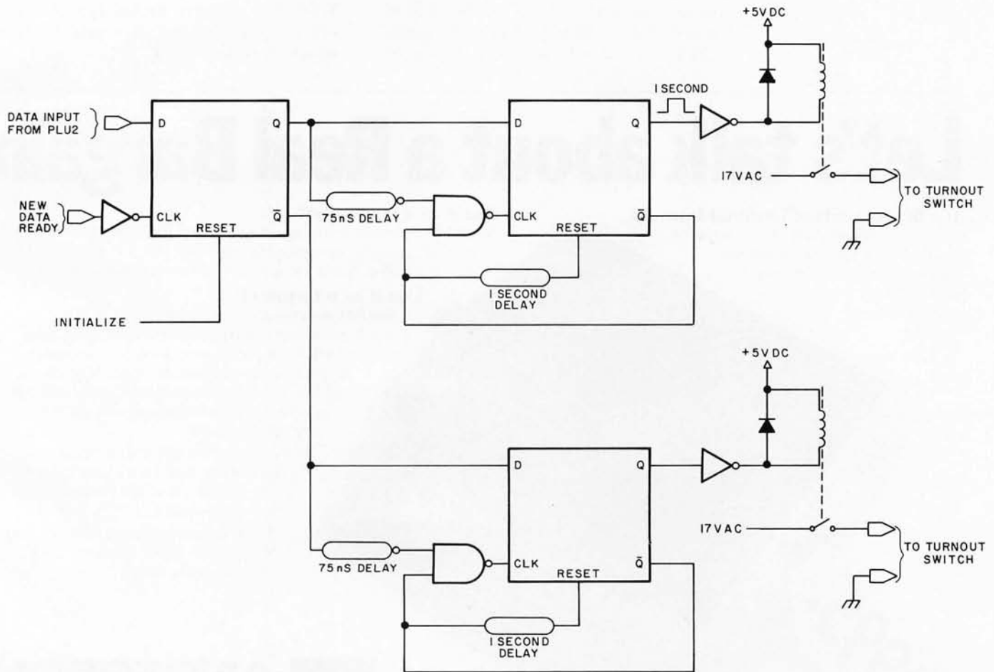
Figure 8: Coil activation circuitry. The coils used to energize the track solenoids cannot be energized 100% of the time (a 100% duty cycle) without burning up. This circuit uses flip flops and delay elements to provide a one second pulse to a relay where it is converted to 17 VAC, sufficient to activate the solenoid. This illustration, like the rest in this article, is intended to illustrate a concept rather than to serve as a basis for actual construction.
