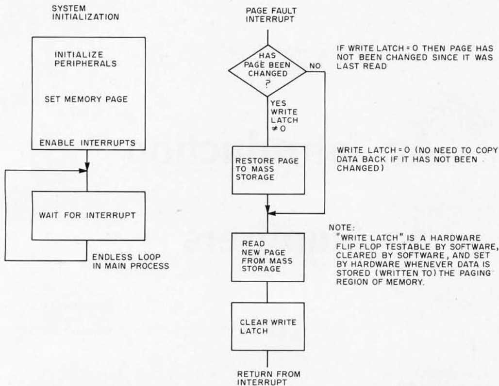
Figure 3: What to do when a page fault occurs. This is a simplified flow diagram of a virtual memory system control process, including initialization and response to a page fault interrupt. It is assumed to be running in a microprocessor dedicated to memory management.
