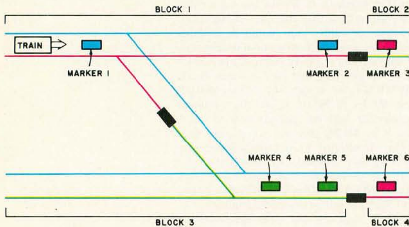
Figure 8b: This figure is slightly more complex than figure 8a. In this type of array the train may enter block 3 or block 2. The computer must determine which block the train will enter. If it is block 3 the information for block 3 must be updated for the particular train as soon as the train has passed marker 1. If the train will enter block 2 next, however, the information for block 2 must not be updated until the train has passed marker 2.
