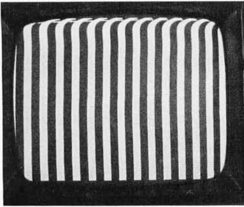
Photo 2: Exploring the circuit with the probing alligator clip produces various interesting signals. Here the clip looks at address bit 1, point 1 on figure 1. This signal changes state every other character position, giving vertical bars two character widths wide. Note the distortion at the top of the image, not normally seen due to blanking of the display.
