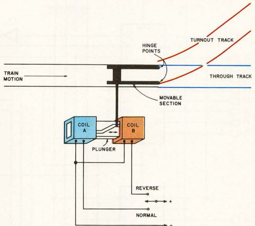
Figure 5: The basic workings of a turnout and switch machine. The two coils of wire move a piece of soft metal with a groove back and forth between them. The switch machine rides in the groove. When coil B is activated, by using the reverse mode, the metal is pulled into the B coil and the switch machine slides down in the groove changing the position of the switch machine.
