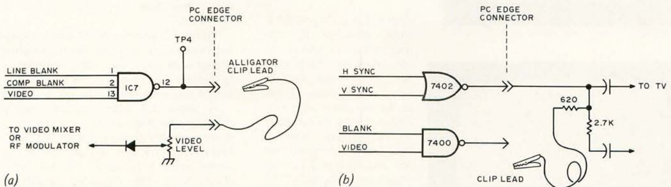
Figure 2: (a) A modification of the Gantt television display circuit, of page 18, June 1976 BYTE, to use this test instrument technique. The line from IC7 pin 12 to the video level potentiometer is broken so that input to the video mixer, and thus to the TV, is taken from some arbitrary point under test rather than the usual source. (b) The author's video output circuitry, with a similar clip lead jumper normally in place for display purposes, but free to be moved around for testing purposes.
