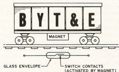
Figure 6: This is a magnetic reed switch which can be used as a marker along the track. The switch consists of two contacts that are enclosed within a glass envelope. The two metal contacts are activated magnetically when a car with a magnet attached passes over.
