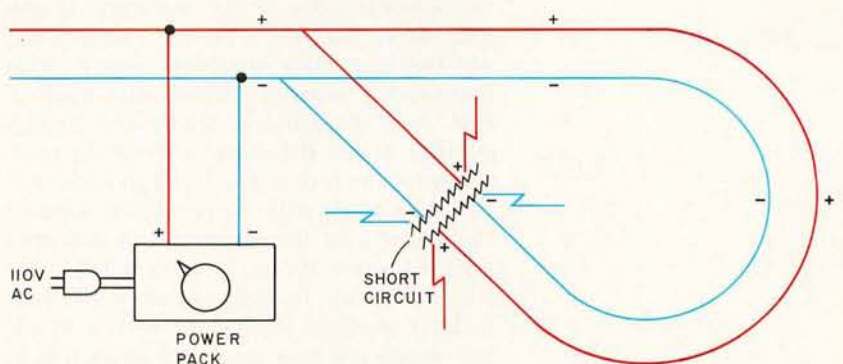
Figure 3: An illustration of the type of difficulty that arises when a track is put through a reverse loop. Following polarities it will be seen that the negative side of the track will connect to the positive side at the end of the loop and vice versa.
