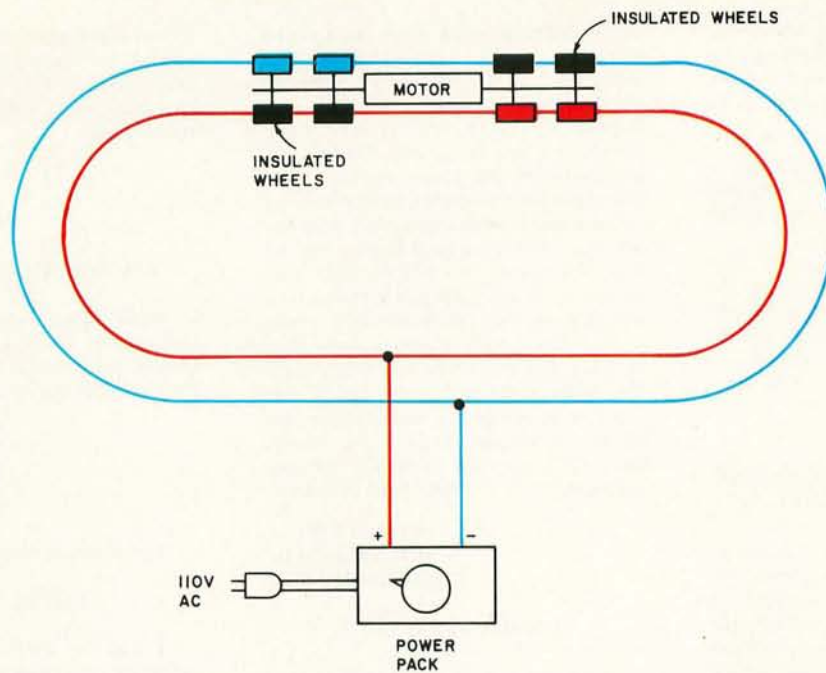
Figure 1: A simple train layout for one train showing the manner in which electricity is transmitted to the motor of the train.
