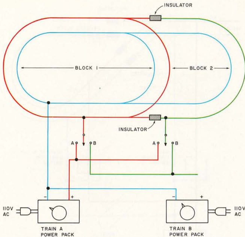
Figure 2: A basic example of block wiring. The negative rail is common to both blocks. The positive rail is divided by insulators into two sections. Each block can run a train using a separate power pack.
