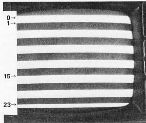
Photo 4: Looking at a single dot position. When the alligator clip is moved to point 3 on figure 1, this pattern is produced. Each character has seven horizontal dot positions, of which two are inactive spacing positions, and five are used for character generation.
