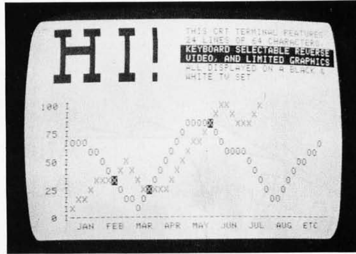
Photo 1: A "typical" display. This shows the completed display in operation. The large block letters are reverse video spaces. The use of blanking prevents generation of any signals at the top or bottom of the screen and keeps the visible portion of the display within the linear region of the TV set.
