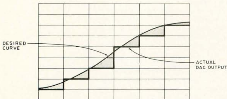
Figure 2: DAC Quantization Errors. The actual output of a computer to the analog world is a step function (in the absence of any filtering). This leads to the problem of quantization errors, depicted conceptually here by the shaded areas in between the smooth analog function and its closest step function approximation. Low precision digital to analog conversions accentuate this problem.
