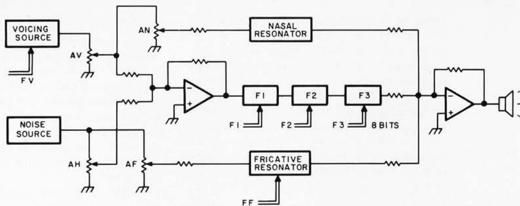
Figure 15: The Complete Synthesizer. This diagram shows the organization of a complete synthesizer which includes a wide variety of parameters. The voicing frequency and amplitude are set by parameters FV and AV. The noise pulses of stop consonants are generated with the programmable gain element AH. The fricative resonator with amplitude AF and frequency resonance FF are used to generate fricatives like "s" and "sh." The normal vowel sounds are generated by control of the formant frequencies F1, F2 and F3, and a nasal resonator with amplitude AN and fixed frequency characteristics is used to add varying amounts of nasal sounds. The result of signals processed through the nasal, formant and fricative paths is summed by a final operational amplifier and used to drive the output speaker.
