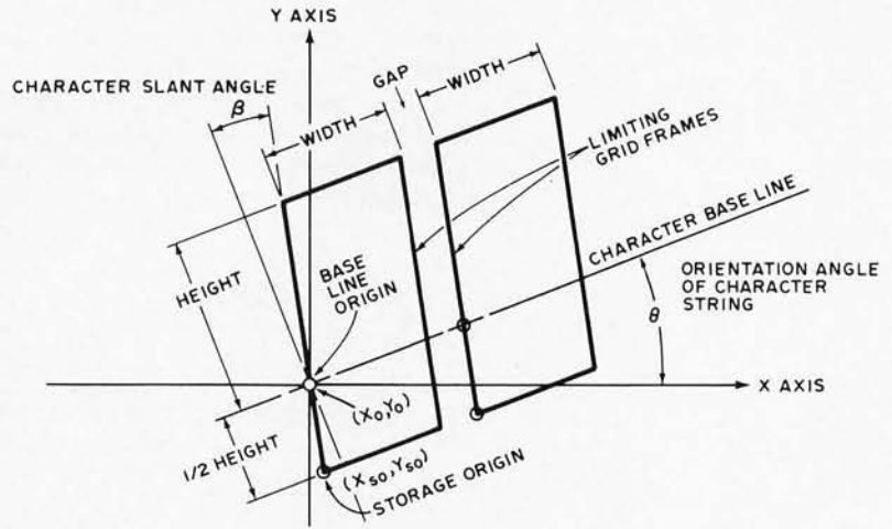
Figure 5: Character Orientation. To add an element of finesse to the plotting function, provision for general purpose rotation and slanting is a desirable feature. There are two angles to specify: angle \theta is the orientation angle of the baseline for a character string; angle \beta is the frame slant relative to a perpendicular through the base line.
