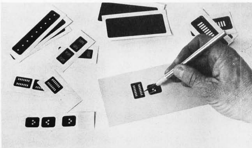
Photo 5: The Bishop Graphics "'B' Neg" Method. In this method, a negative is made directly, using self adhesive black patterns on a mylar backing. The connections between patterns are made by cutting away the black layer with a sharp knife as in the "Cut-N-Peel" method.
