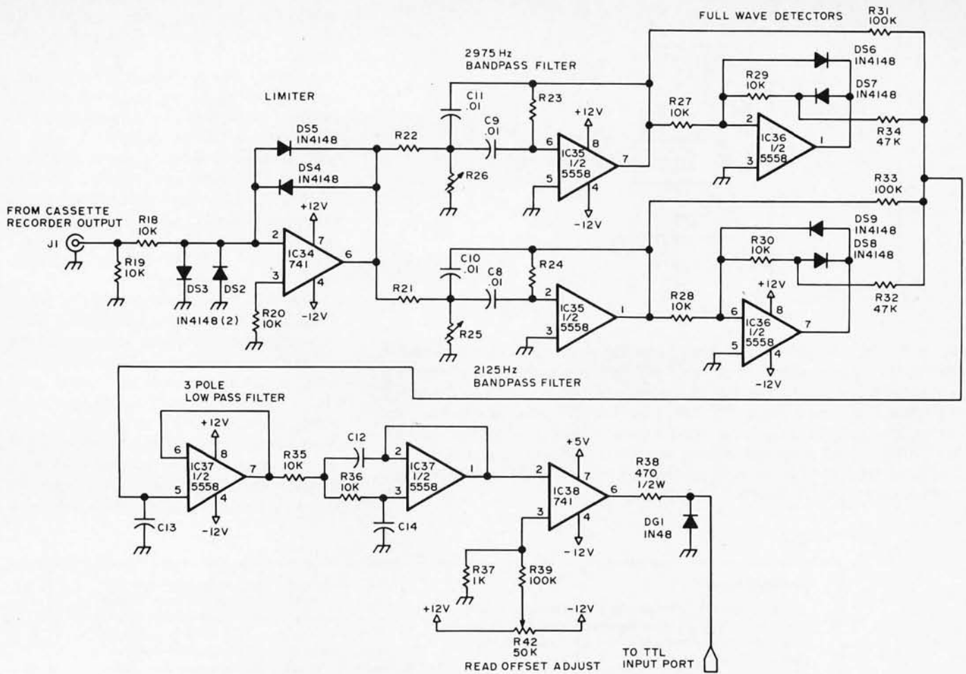
Figure 1: The schematic of the Sudio cassette input interface as found in the Digital Group systems. This interface amplifies and clips the cassette output with limiting amplifier IC34, discriminates the two data frequencies (see table 1) with bandpass filters followed by full wave detectors, passes the detected signal through a 3 pole active low pass filter, then converts the result to a TTL level which is read by a single bit input port. One example of software (see listing 1) to drive this input interface uses a programmed simulation of UART input algorithm; an actual UART or ACIA device could be substituted if desired.
