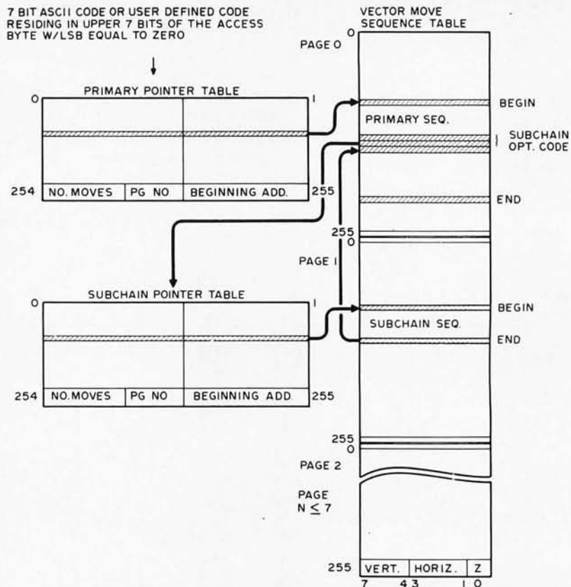
Figure 2: Relationship of the Character Generation Tables. The selected character code is rotated left by one bit to define a number from 0 to 254. This number accesses a 16 bit quantity in the primary pointer table. The primary pointer table in turn locates the beginning of a series of pen locations in the move sequence table which define the character's plot representation. Within that series, there might be a pointer to the subchain table, which in turn points to an often used fragment of the graphics representation located at a different place in the move sequence table. Note that to minimize retrieval effort on machines such as the 8008 and 8080, sequences of moves should be restricted to single pages of memory.
