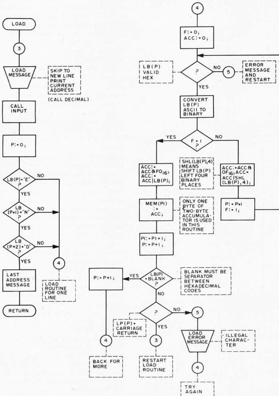
Figure 6: The LOAD Subroutine Specified as a Flow Chart. The purpose of LOAD is to set the contents of user program-mable memory beginning at a location specified by the user. The routine continues indefinitely until the characters "END" begin a line of input.
