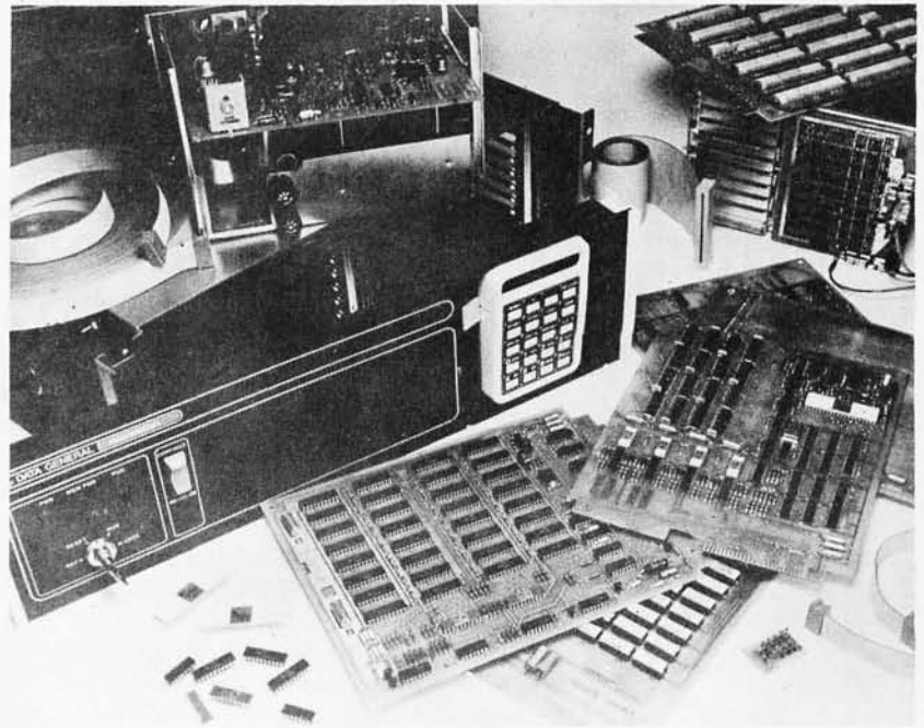
Photo 3: For the do it yourself systems house, Data General provides a complete line of modular components which can be integrated to form a microNOVA system. One of the most interesting characteristics of the microNOVAs integrated to the minicomputer level is a "Programmer's Helper" remote console packaged in a calculator style case at the end of a ribbon cable. The console is shown in its storage position in the front panel assembly at the center of this picture.
