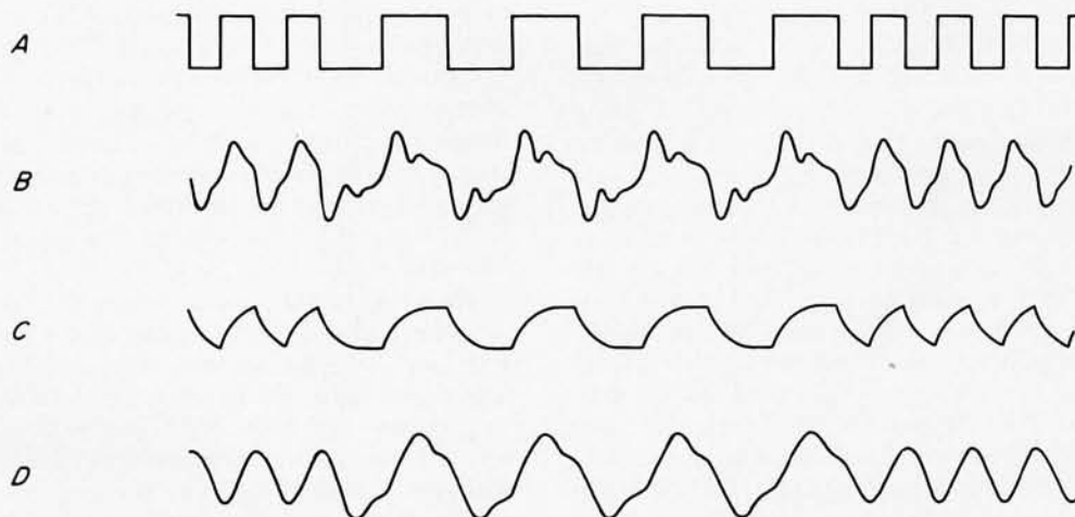
Figure 2: If a square wave signal such as waveform A is recorded on a low cost cassette recorder, the playback response may look like waveform B, which is very difficult to demodulate. If the square wave is filtered with a low pass filter before recording (waveform C), the playback response will look like waveform D, which is a usable signal.
