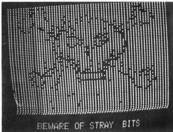
Photo 8: This illustrates a cartoon drawn using the erase mode of operation with the improved circuit of figure 3.
