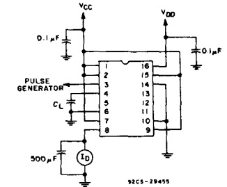
Fig. 16 - Dynamic power dissipation test circuit.
