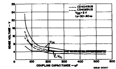
Fig. 15 Ground-line noise-immunity measurements.
