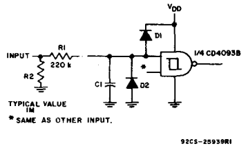
Fig. 20 - Industrial-environment to COS/MOS interface.
