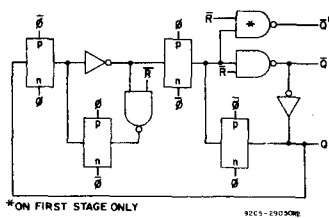
Fig. 4 - Detail of typical flip-flop stage.
