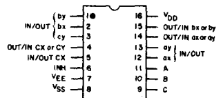
CD4053B Terminal Assignment
