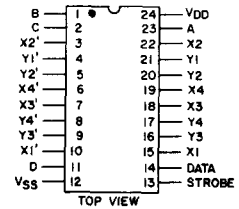
92CS-29839 CD22101 Terminal Diagram
