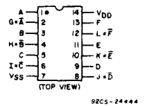
Fig. 7 - CD4069UB terminal assignment.
