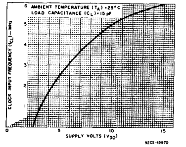
Fig. 4 - Typical clock input frequency vs. supply voltage.
