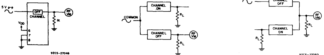
Fig. 24 - Feedthrough (all types).
