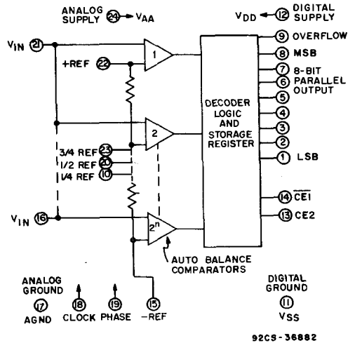
8-Bit Flash A/D Converter CA3308 (Page 631) CA3308A (Page 631)
