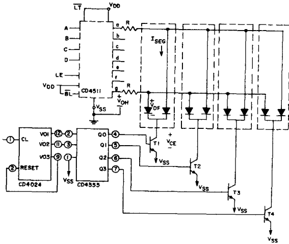
Fig. 15 — Driving common-cathode 7-segment LED displays (example Hewlett-Packard 5082-7740).
