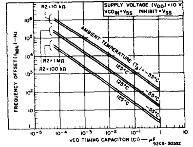
Fig. 7 - Frequency offset as a function of C1 and R2 for ambient temperatures of -55°C to 125°C.
