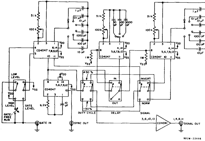
Fig. 34 - Pulse-generator circuit.
