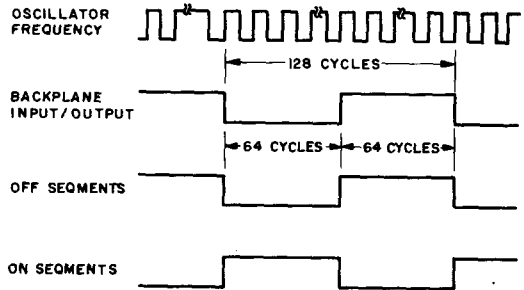
Fig. 6 - Display waveforms.
