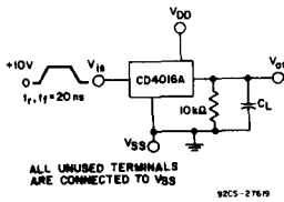
Fig. 19 - Propagation delay time signal input ( V_{IS} ) to signal output ( V_{OS} ).
