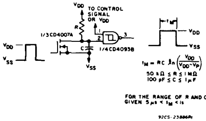
Fig. 17 - Monostable multivibrator.
