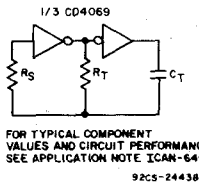
Fig. 21 - Typical RC oscillator circuit.
