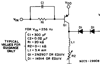
(a) Pulsed, single-transistor-inductor flyback circuit.
