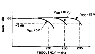
(a) TYPICAL CD4001B LINEAR GAIN
