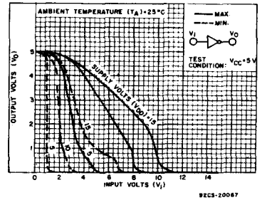
Fig. 3 — Minimum and maximum voltage transfer characteristics—CD4009UB.
