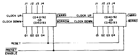
Fig. 18 - Cascaded counter packages.
