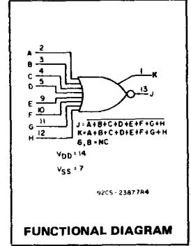
FUNCTIONAL DIAGRAM
