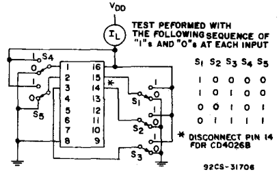
Fig. 15 - Quiescent device current.
