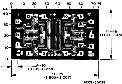
Dimensions and Pad Layout for CD4093BH
