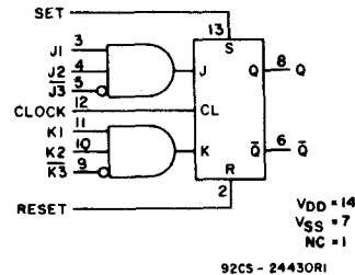
Gated J-K Master-Slave Flip-Flop, Inverting and Non-Inverting Inputs CD4096B (Page 282)
