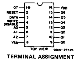
TERMINAL ASSIGNMENT
