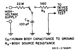
Fig. 5 - Equivalent-body discharge network.
