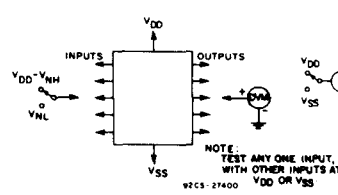
Fig. 20 - Noise immunity test circuit.
