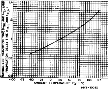
Fig. 13 — Variation of low-to-high ( t_{TLH} ) and high-to-low ( t_{TLH} ) transition time, and low-to-high ( t_{PLH} ) and high-to-low ( t_{PLH} ) propagation delay time with temperature.
