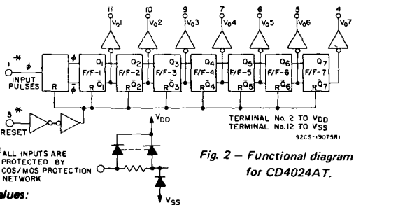
Fig. 2 - Functional diagram for CD4024AT.
