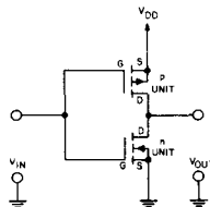
Fig. 3 - Basic COS/MOS inverter (schematic).
