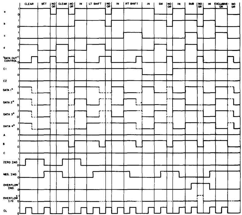
Fig. 12 — Timing diagram.
