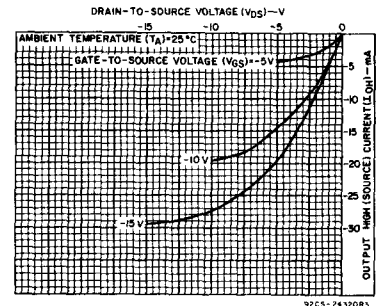
Fig. 5 - Typical p-channel output high (source) current characteristics.
