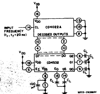
Fig. 11 - Dynamic power dissipation test circuit.
