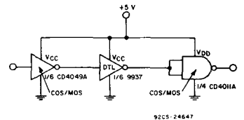
Fig. 6-COS/MOS to DTL to COS/MOS interface.
