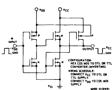
Fig. 1 — Schematic diagram of CD4009UB—1 of 6 identical stages.
