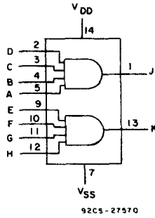
Dual 4-Input AND Gate CD4082B (Page 250)
