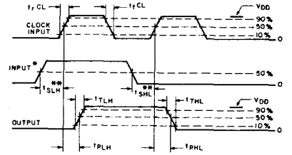
Fig. 3 - Synchronous operation propagation delay times, transition times, and set-up times.
