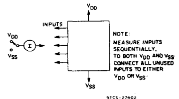
Fig. 15 - Input-current test circuit.
