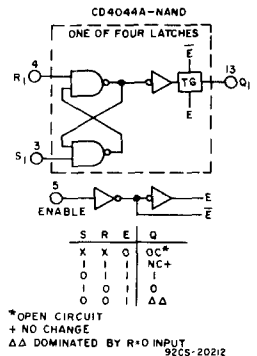
Fig. 1 - Logic diagrams and truth tables.
