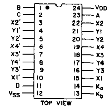
92CS-29840 CD22102 Terminal Diagram
