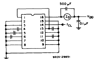
Fig. 14 - Dynamic power dissipation test circuit.
