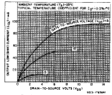
Fig. 9 – Typical output low (sink) current characteristics.
