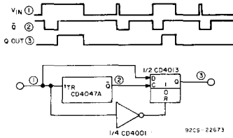
Fig. 23 - Noise-discriminator circuit.
