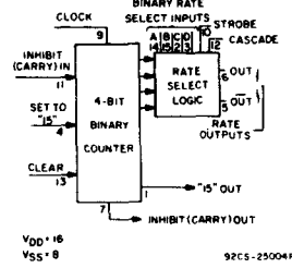
Binary Rate Multiplier CD4089B (Page 269)
