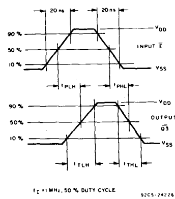
Fig. 18 - CD4555B E input to Q3 output dynamic signal waveforms.
