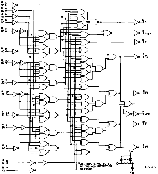
Fig. 3 - CD40181B logic diagram (active-low data).
