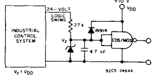
Fig. 13—Zener diode industrial control interface.
