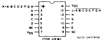
TERMINAL ASSIGNMENT
