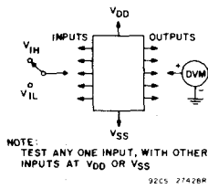
Fig. 16 - Noise immunity test circuit.
