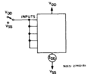
Fig. 26—Quiescent-device current test circuit.
