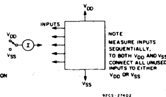
Fig. 11 — Input current.
