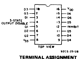
TERMINAL ASSIGNMENT
