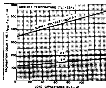
Fig. 10 — Clock-to-parallel output propagation delay vs C_L .
