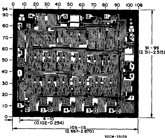
Dimensions and pad layout for CD4060B.
