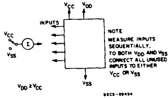
Fig. 15 - Input current.
