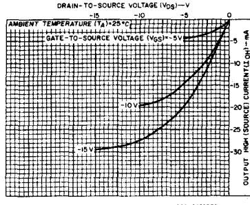
Fig. 4 — Typical output high (sink) current characteristics.
