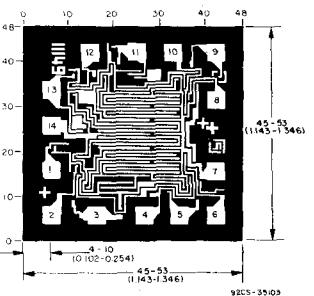
Dimensions and pad layout for CD4069UBH. The photographs and dimensions of each CMOS chip represent a chip when it is part of the wafer. When the wafer is separated into individual chips, the angle of cleavage may vary with respect to the chip face for different chips. The actual dimensions of the isolated chip, therefore, may differ slightly from the nominal dimensions shown. The user should consider a tolerance of \pm 3 mils to \pm 16 mils applicable to the nominal dimensions shown.
