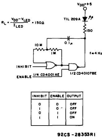
Fig. 7 - LED driver circuit.
