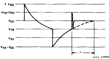
Fig. 15 - CD4047A one-shot RC waveform.
