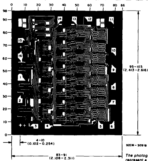
CD4724BH DIMENSIONS AND PAD LAYOUT
