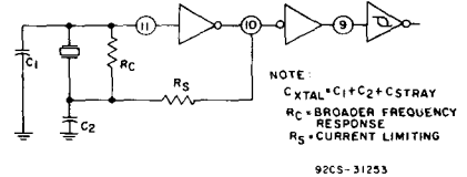
Fig. 13 — Typical crystal circuit.
