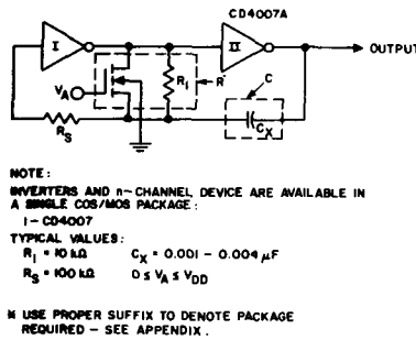
Fig. 19 - Voltage controlled oscillator.
