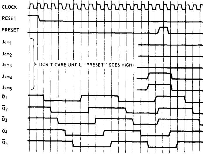
Fig. 15 -- Timing diagram.
