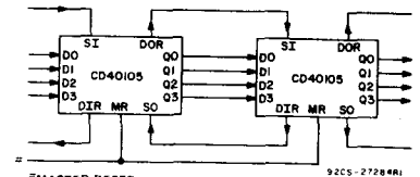
Fig. 3 - Expansion, 4-bits wide-by-16 N-bits long.
