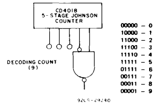
Fig. 9 - External gate required by Johnson counter; counting sequence requiring only one bit change at a time.
