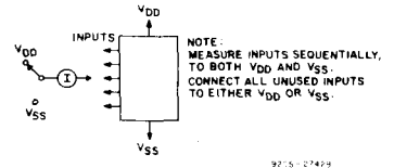
Fig. 17 - Input leakage current test circuit.
