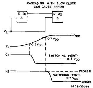
Fig. 6—Error effect that results from a slow clock in cascaded circuits.
