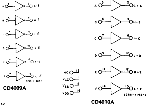
Fig. 1 — Logic diagrams.
