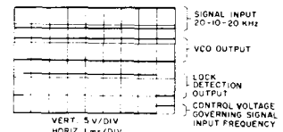
Fig. 16— Lock-detection-circuit waveforms.
