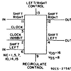
32-Stage Static Left/Right Shift Register
