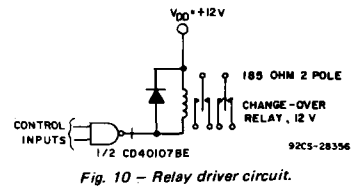
Fig. 10 - Relay driver circuit.
