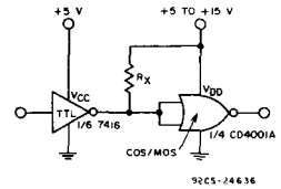
Fig. 4-TTL to COS/MOS at a V DD greater than 5 volts.
