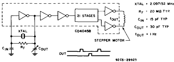
Fig. 1 - CD4045, COS/MOS 21-stage counter, used to generate crystal oscillator output and to drive stepper motor.
