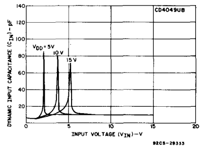
Fig. 9 Dynamic input capacitance curves for the CD4049UB. T_A = 25^\circ C .
