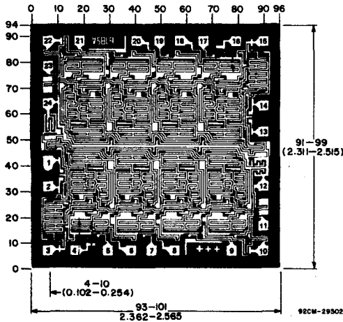
Fig. 15 - Bus register.
