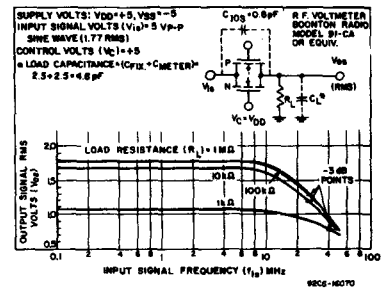
Fig. 11—Typical frequency response—switch on.
