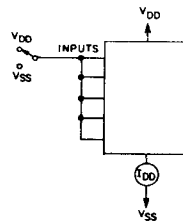
Fig. 13 - Quiescent device current test circuit.
