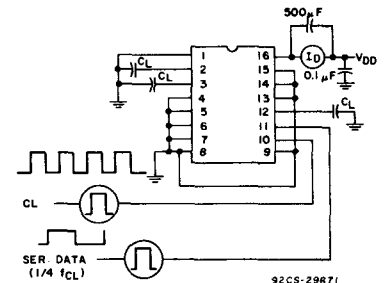
Fig. 10 — Dynamic power dissipation test circuit.
