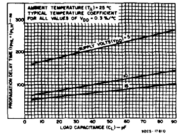
Fig. 8 - Typical propagation delay time vs. C L .
