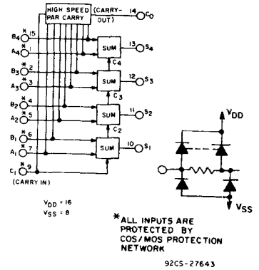
Fig. 1 — CO4008B logic diagram.
