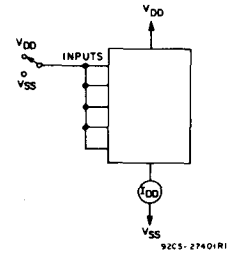
Fig. 19 - Quiescent device current test circuit.
