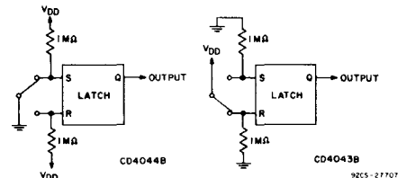
Fig. 12 — Switch bounce eliminator.
