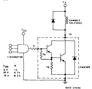
Fig. 16—COS/MOS system driving a printer-hammer solenoid with the aid of a Darlington transistor.
