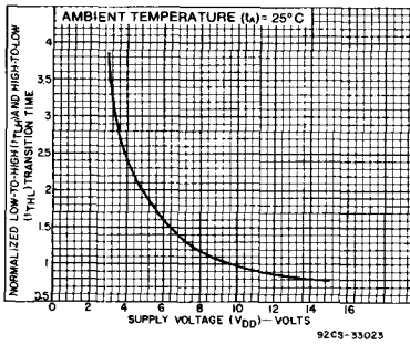
Fig. 14 — Variation of low-to-high ( t_{TLH} ) and high-to-low ( t_{TLH} ) transition time with supply voltage.
