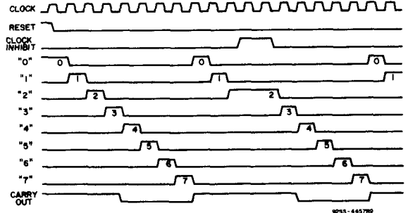
Fig. 2 - Timing diagram.
