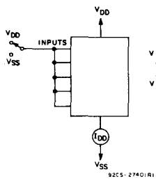
Fig. 20 - Quiescent device current test circuit.
