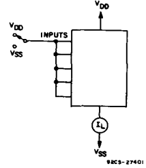
Fig.18 – Quiescent device current test circuit.
