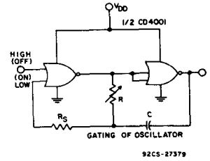
Fig. 7 - Astable multivibrator in which a NOR or NAND gate is used as the first inverter to permit gating of the multivibrator.
