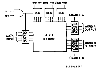
Fig. 1 - Block diagram.
