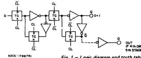
Fig. 1 — Logic diagram and truth table (one register stage).
