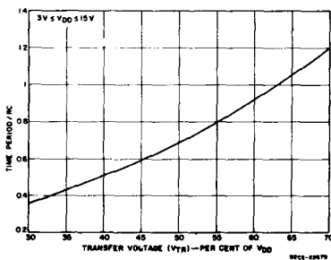
Fig. 12 - Simple one-shot time period as a function of transfer voltage. 92CS-22679
