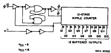
Fig. 4 - Functional diagram.
