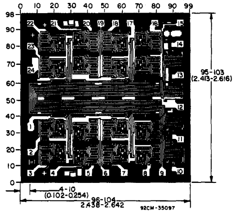
Dimensions and pad layout for CD4097BH.
