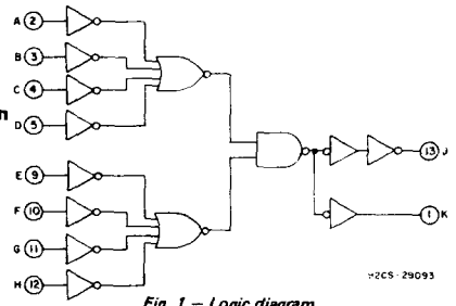
Fig. 1 - Logic diagram.
