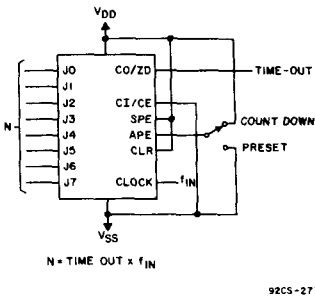
Fig. 19 - Programmable timer.
