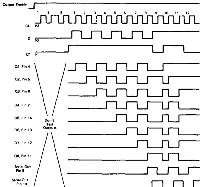
Fig. 5 - Waveforms used in functional testing.
