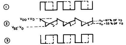
Fig. 8 - Waveforms showing effects of transfer voltage on multivibrator frequency.
