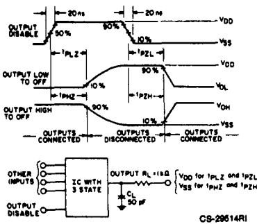
Fig. 18 - Three-state propagation delay wave shapes and test circuit.
