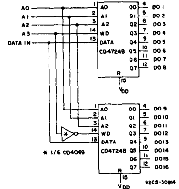
Fig. 14— 1 of 16 decoder/demultiplexer.
