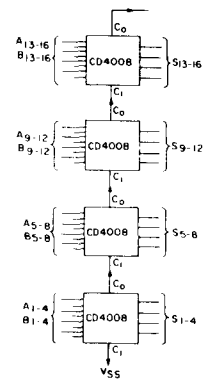
Fig. 10 - Typical connection for a 16-bit adder.
