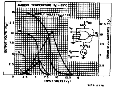
Fig. 3 - Typical current & voltage transfer characteristics.
