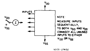
Fig. 16 - Input current.
