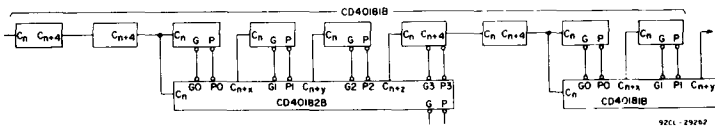
Fig. 15 – Combined two-level look-ahead and ripple-carry ALU.
