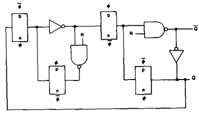
Fig. 2 - Detail of typical flip-flop stage.
