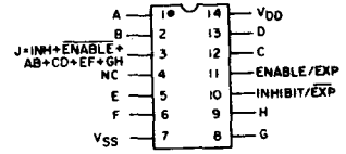
92CS-23869R1 Top View TERMINAL ASSIGNMENT
