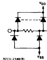
Fig. 1 - Logic diagram - 1 of 4 Schmitt triggers.
