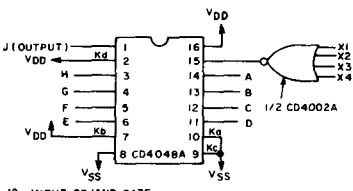
12- INPUT OR/AND GATE J = (A+B+C+D) \cdot (E+F+G+H) \cdot (X1+X2+X3+X4) Fig. 4 - 12-input OR/AND gate.
