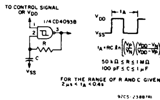
Fig. 18 - Astable multivibrator.
