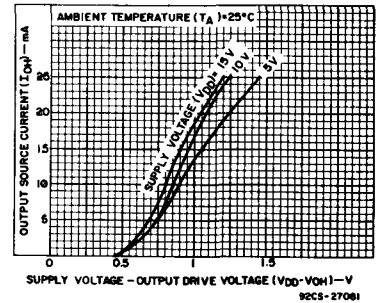
Fig. 13 - Typical voltage drop (V DD to output) vs. output source current as a function of supply for the CD4511.
