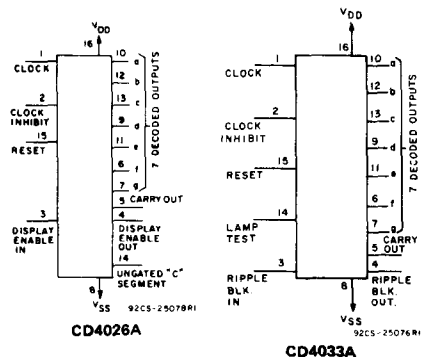
FUNCTIONAL DIAGRAMS
