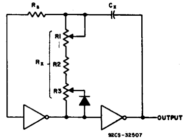
Fig. 4 - Method of controlling the duty cycle of the RC oscillator.
