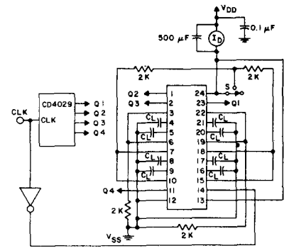
Fig. 14 - Dynamic power dissipation test circuit for CD22101.
