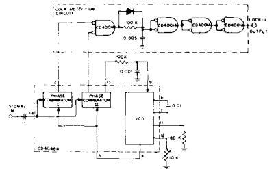
Fig. 15— Lock-detection circuit.
