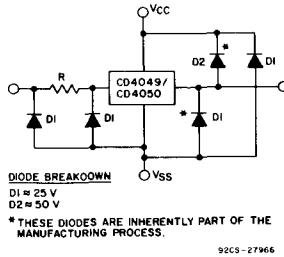
Fig. 3 - Modified protection network.
