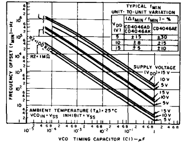
Fig. 9(b)— Typical frequency offset vs. C_1 for R_2 = 10\text{ K}\Omega , 100\text{ K}\Omega , and 1\text{ M}\Omega .
