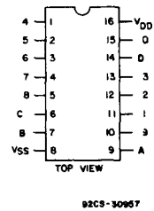
CD40147B TERMINAL ASSIGNMENT
