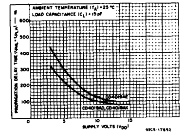
Fig. 4 - Maximum propagation delay time vs. supply voltage.
