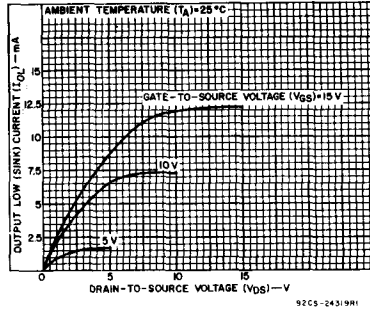
Fig. 8 — Minimum output low (sink) current characteristics.
