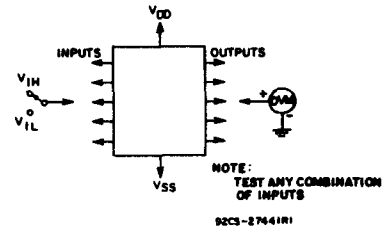
Fig. 12 - Noise immunity test circuit.
