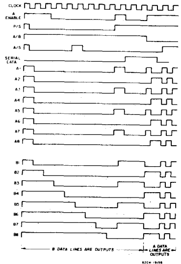
Fig. 4 - Timing diagram.
