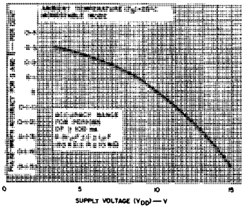
Fig. 24 - Typical Q- and Q-bar-pulse-width accuracy vs supply voltage (tM ≥ 100 ms).
