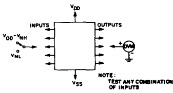
Fig. 14 — Noise immunity test circuit.
