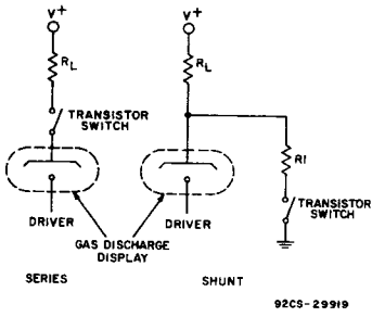
Fig. 14 - Basic series and shunt circuits for multiplexing gas-discharge displays.
