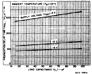
Fig. 6 — Typical propagation delay time as a function of load capacitance (clock to \text{CO}/\overline{\text{ZD}} ).
