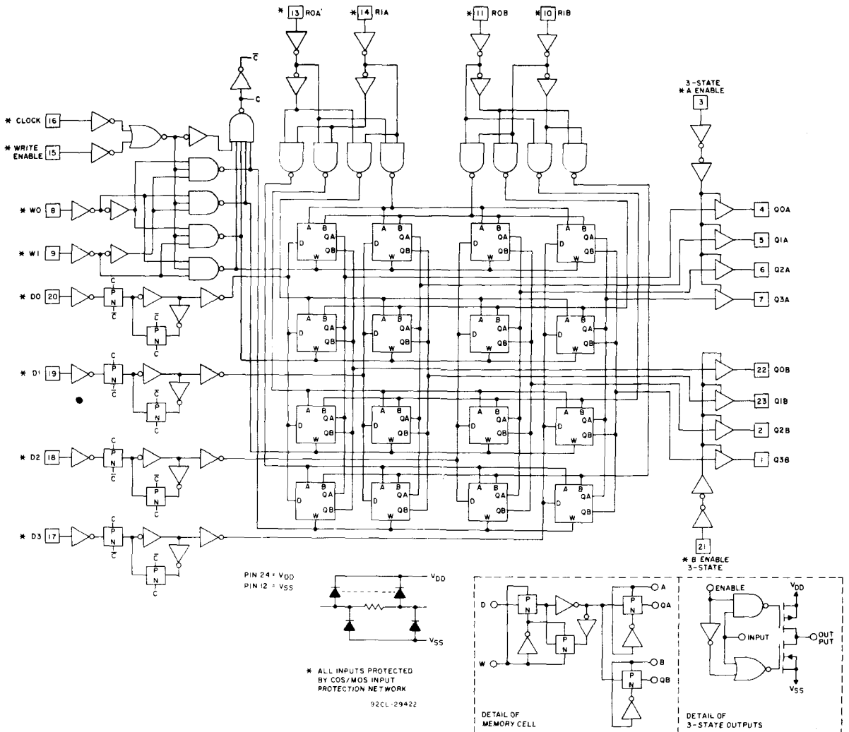
Fig. 13— Schematic diagram
