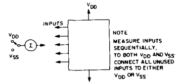
Fig. 15 - Input current test circuit.
