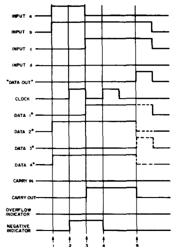
Fig. 13 — Add cycle waveforms.
