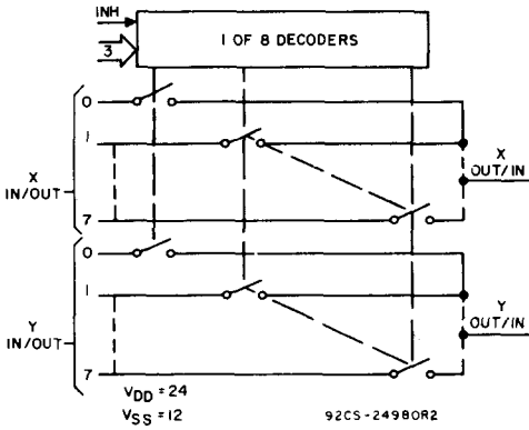
V DD = 24 V SS = 12 92CS-24980R2 Differential 8-Channel Multiplexer/Demultiplexer CD4097B (Page 231)
