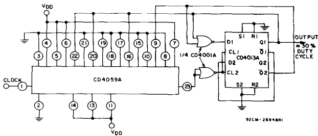
Fig. 16 - Division by 47,690 in \div 2 mode.
