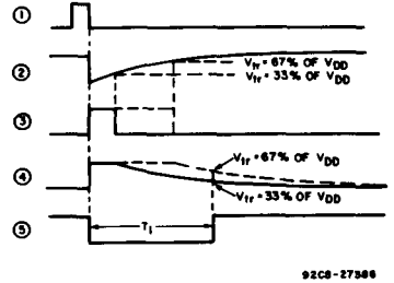
Fig. 14 - Waveforms showing the cancelling effects of transfer-voltage variations of the two COS/MOS inverters when two equal time constants are used.
