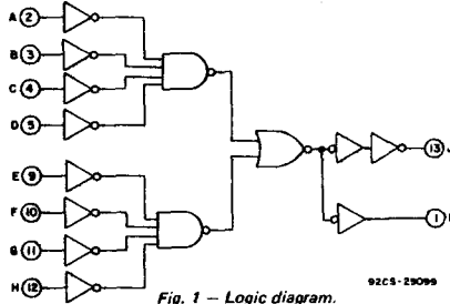
Fig. 1 - Logic diagram.
