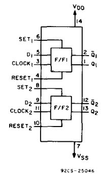
Fig. 5 - Functional diagram of dual D flip-flop type CD4013.
