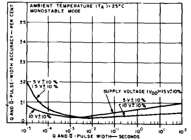
Fig. 25 - Typical Q- and Q-bar pulse-width accuracy vs Q and Q-bar pulse width for a variation of ±10% from value indicated.
