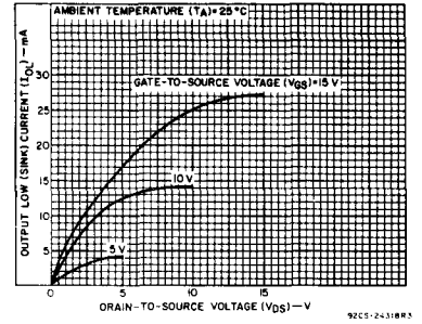
Fig. 8 - Typical output low (sink) current characteristics.
