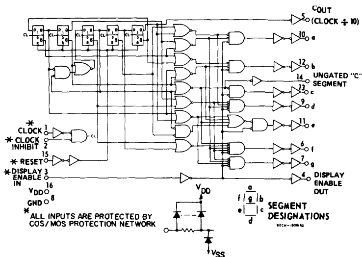
Fig. 1 - CD4026A logic diagram.
