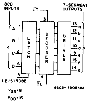
92CS-25083R2 BCD-to-7-Segment Latch Decoder Driver CD4511B (Page 311)
