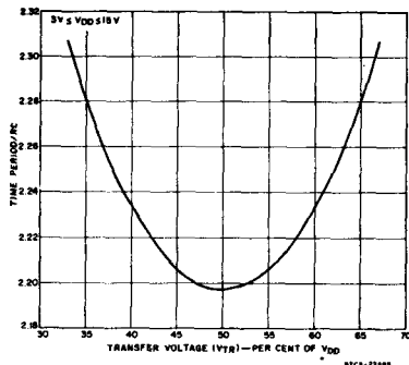
Fig. 9 - CD4047 time period as a function of transfer voltage. 92CS-22685
