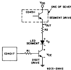
Fig. 12 - Segment and digit drive circuit for LED.
