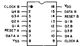
TERMINAL DIAGRAM
