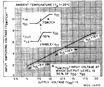
Fig. 9 - Typical input switching as a function of high-level supply voltage.
