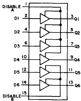
92CS-32392R1 Hex Buffer 3-State Non-Inverting CD4503B (Page 298)
