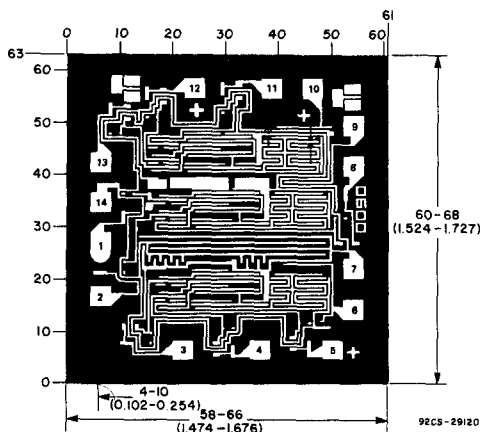
Dimensions and pad layout for CD4075B.
