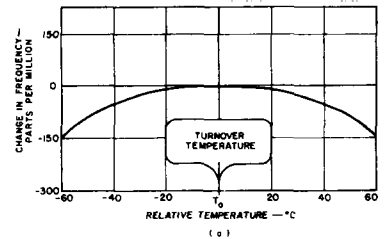
Fig. 7— Effect of temperature on crystal frequency.
