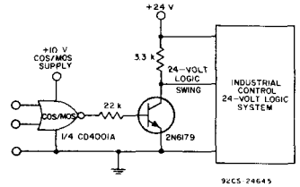
Fig. 14—COS/MOS to industrial-control interface.
