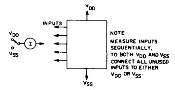
Fig. 8 - Input current test circuit.
