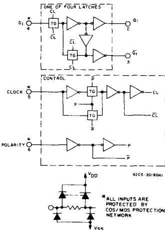
Fig. 1 - Logic block diagram and truth table.
