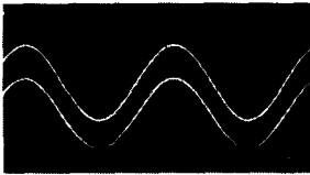
SCALE: X = 0.2 ms/DIV Y = 2.0 V/DIV V_{DD} = V_C = +7.5\text{V} , V_{SS} = -7.5\text{V} , R_L = 10\text{k}\Omega C_L = 15\text{pF} f_{IS} = 1\text{KHz} V_{IS} = 5\text{V p-p} DISTORTION = 0.2%
