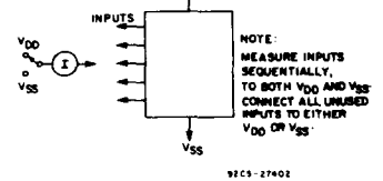
Fig. 16 — Input leakage current test circuit.
