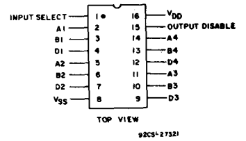
TERMINAL ASSIGNMENT
