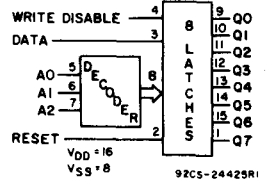
92CS-24425R1 8-Bit Addressable Latch CD4099B (Page 291)
