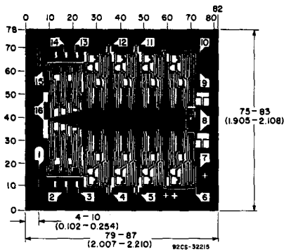
DIMENSIONS AND PAD LAYOUT FOR CD4555BH.
