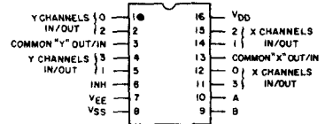
CD4052B Terminal Assignment
