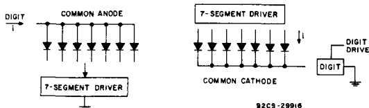
Fig. 8 - Common cathode and common anode light-emitting diode configurations.
