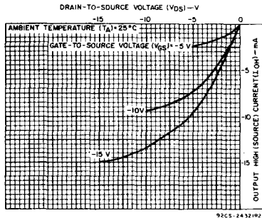
Fig. 7—Minimum p-channel output high (source) current characteristics.
