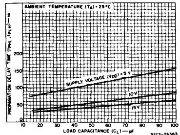
Fig. 6 - Typical propagation delay (E 1 to G S , E 1 to E 0 ) vs. load capacitance.
