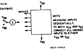
Fig. 11 - Input current.
