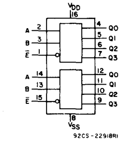
Dual Binary-to-1-of-4 Decoder/Demultiplexer Output "High" on Select
