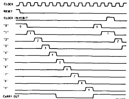
Fig. 2 - Timing diagram.
