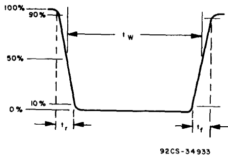
Fig. 6 - Output pulse waveform.
