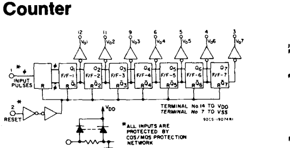
Fig. 1 - Functional diagram for CD4024AD, AE, AF.
