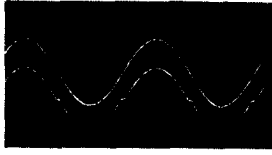
SCALE: X = 0.2 mV/DIV Y = 2.0 V/DIV V_{DD} = V_C = +2.5V, V_{SS} = -2.5V, R_L = 10K\Omega C_L = 15 pF f_{IS} = 1 KHz, V_{IS} = 5V p.p. DISTORTION = 3 %
