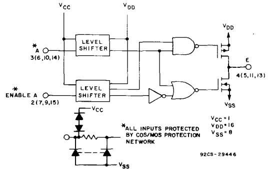
Fig. 1 - CD40109B logic diagram (1 of 4 units).
