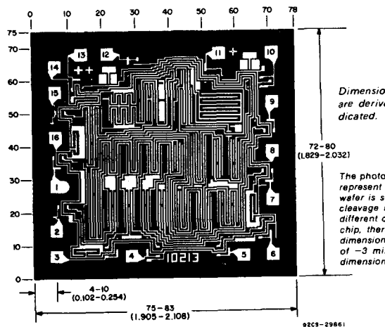
Dimensions and pad layout for CD4512BH
