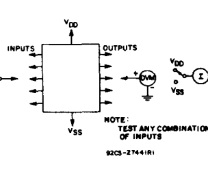
Fig. 11 — Input voltage test circuit.
