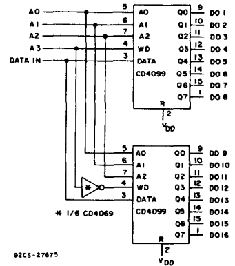
Fig. 14 - 1 of 16 decoder/demultiplexer.
