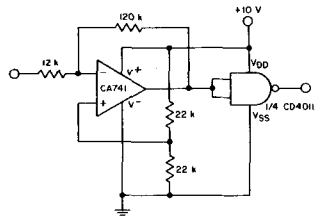
Fig. 21—Interface of op-amp and COS/MOS with common supply rail.
