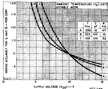
Fig. 10 - Supply Q and \bar{Q} -period accuracy vs supply voltage (high frequency).
