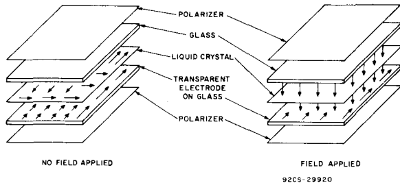
Fig. 6 - Basic operation of field-effect type liquid crystal device showing molecule alignment and major elements.
