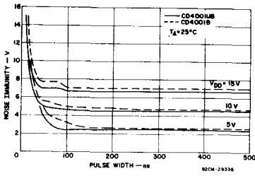
(a) CD4001B, CD4001UB
