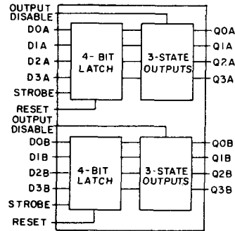
92CS-27494R1 Dual 4-Bit Latch CD4508B (Page 301)
