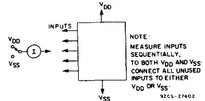
Fig. 24—Input-current test circuit.
