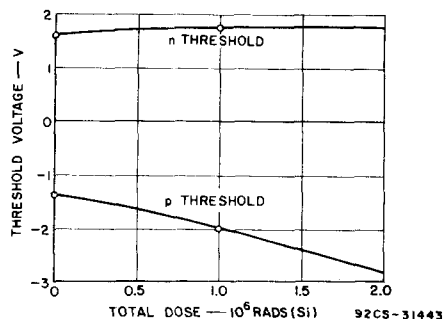
Typical threshold-voltage variations of RCA MEGARAD CD4000-series CMOS integrated circuits as a function of total-dose gamma radiation.
