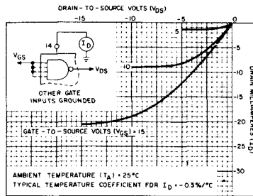
Fig. 2b - Typical p-channel characteristics.
