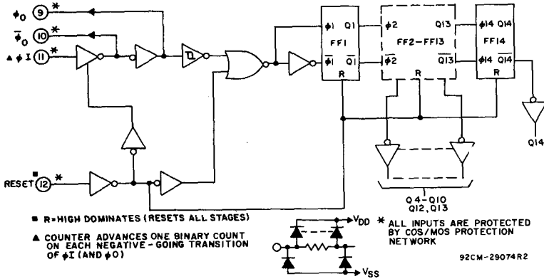
Fig. 1 - Logic diagram.
