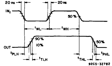
Fig. 22—Input waveforms for switching-time test circuit.
