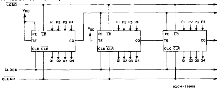
Fig. 18 — Cascaded counter packages in the parallel-clocked mode.
