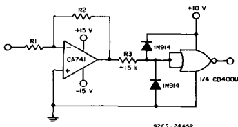
Fig. 20—Split-rail op-amp to COS/MOS interface.
