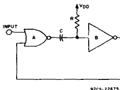
Fig. 11 - CMOS/MOS monostable circuit. 92CS-22675
