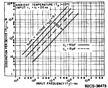
Fig.6 — Typical power dissipation vs. frequency.
