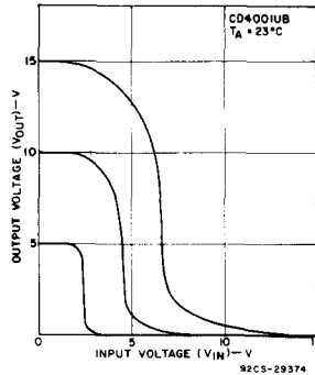
Fig. 4 CD4001UB voltage transfer characteristic.
