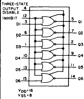
92CS-22921R1 Strobed Hex Inverter/Buffer CD4502B (Page 295)
