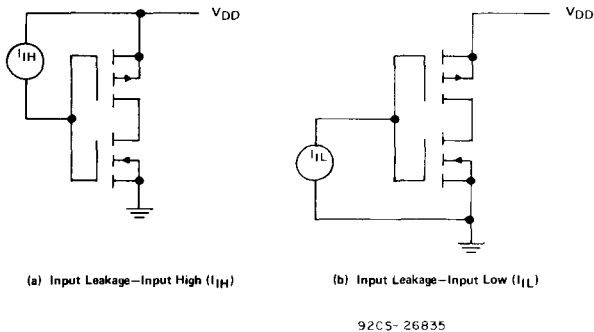
Fig. 9 — Measurement of input leakage.
