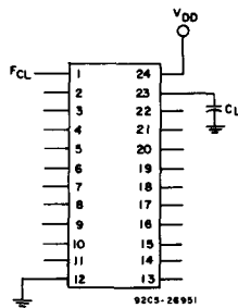
Fig. 19 - Power dissipation test circuit (all \div modes).
