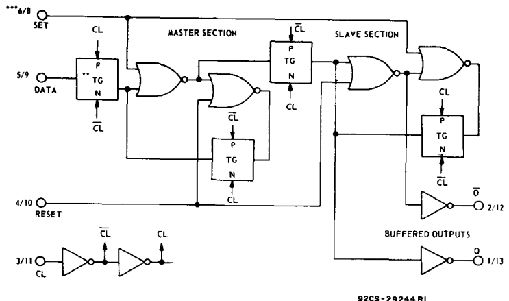
Fig. 2 - Detailed diagram of master-slave flip-flop, the sequential memory element of most static counters including the CD4024.
