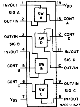
Quad Bilateral Switch CD4066A (Page 616) CD4066B (Page 228)
