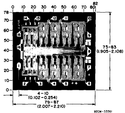
DIMENSIONS AND PAD LAYOUT FOR CD4556BH.
