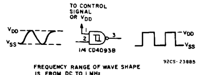
Fig. 16 - Wave shaper.
