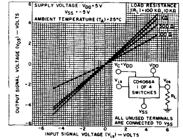
Fig. 4 - Typical ON characteristics for 1 of 4 channels.
