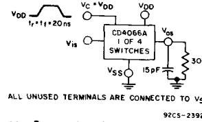
Fig. 11 - Propagation delay t PLH , t PHL control-signal output.
