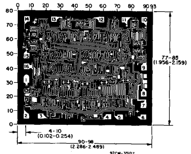
Dimensions and pad layout for CD4056BH
