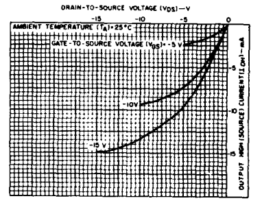
Fig. 4 - Minimum output high (source) current characteristic.
