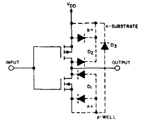
Fig. 4 - Basic inverter showing parasitic diodes.
