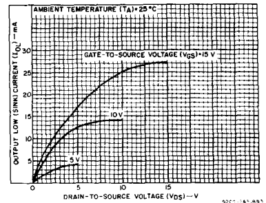
Fig. 3 - Typical n-channel output low (sink) current characteristics.
