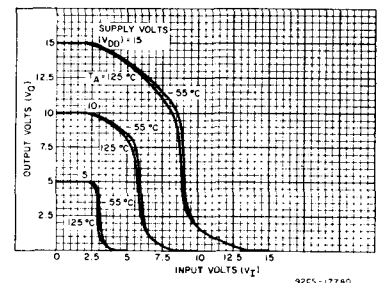
Fig. 5 - Typical COS/MOS transfer characteristics as a function of temperature.
