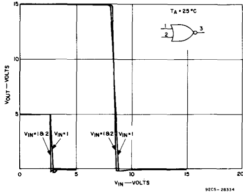
Fig. 5 — Voltage transfer characteristics of a buffered 2-input NOR gate (CD4001B).
