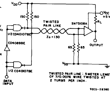
Fig. 14 - Line-driver circuit.
