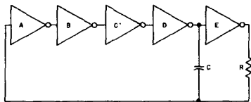
Fig. 8 - CD4047A oscillator section 92CS-22676
