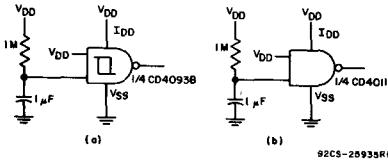
Fig. 15 - Reset circuit: a comparison of the CD4093B with the CD4011.
