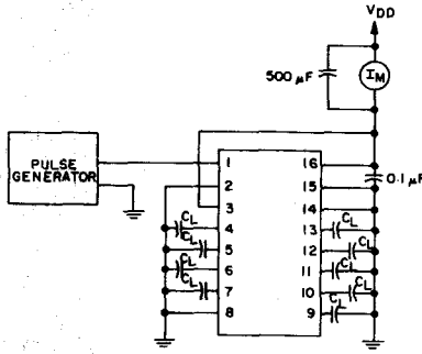
Fig. 14 - Dynamic power dissipation test circuit for CD4033B.
