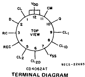
TERMINAL DIAGRAM
