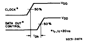
Fig. 7 - Data hold time.
