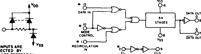
Fig. 12 - Functional diagram.
