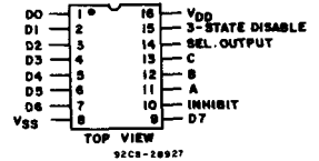
TERMINAL ASSIGNMENT
