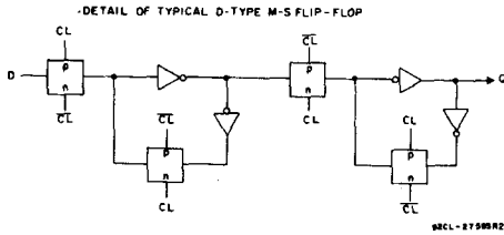
Fig. 3 - Logic diagram.
