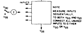
Fig. 20 - Input current test circuit.
