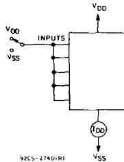
Fig. 10 — Quiescent current test circuit.
