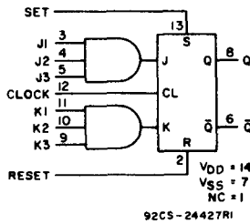
Gated J-K Master-Slave Flip-Flop, Non-Inverting Inputs CD4095B (Page 282)
