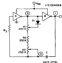
Fig. 9 - Astable multivibrator in which a duty-cycle control is added.
