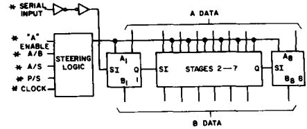
Fig. 1 - Functional diagram.
