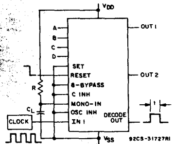
Fig. 28—Time interval configuration using external clock; reset and output monostable to achieve a pulse output.
