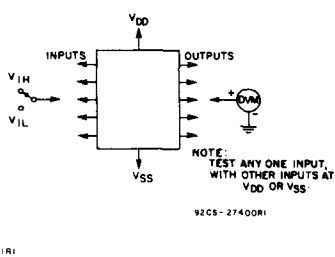
Fig. 21 - Noise immunity test circuit.
