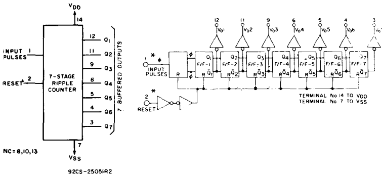
Fig. 1 - Functional and logic diagrams for a COS/MOS 7-stage binary counter type CD4024.
