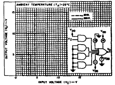
Fig. 2 — Minimum and maximum voltage transfer characteristics.
