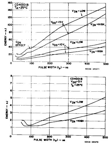
Fig. 24 High- and low-input state noise-energy immunity for the CD4001B gate as a function of input pulse width. T A = 25°C.
