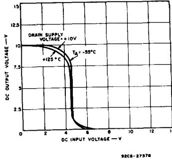
Fig. 6 - Transfer characteristic as a function of temperature.
