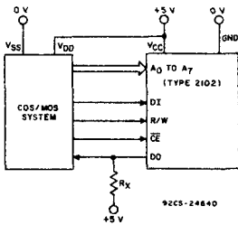
Fig. 9—Direct interface between COS/MOS and 1k memory, type 2102.
