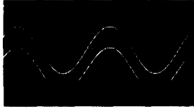
SCALE: X = 0.2 mV/DIV Y = 2.0 V/DIV V_{DD} = V_C = +7.5V, V_{SS} = -7.5V, R_L = 10K\Omega C_L = 15 pF f_{IS} = 1 KHz, V_{IS} = 5V p.p. DISTORTION = 0.2 %
