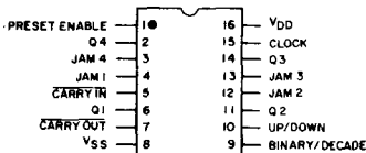
CD4029B Terminal Diagram
