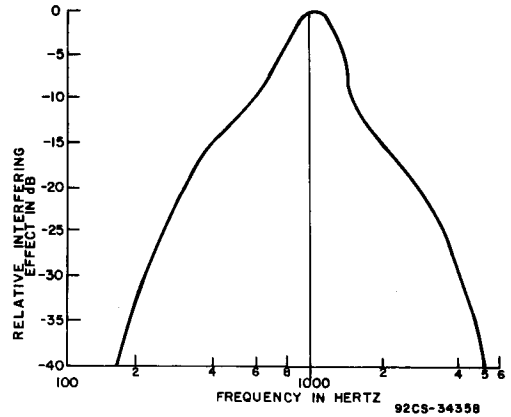
Fig. 1 - Weighting curve used with Western Electric 144 handset.
