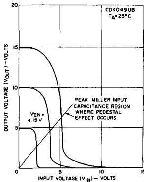
(c) CD4049UB T_A = 25^\circ C .
