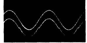
SCALE: X = 0.2 ms/DIV Y = 2.0 V/DIV V_{DD} = V_C = +2.5\text{V} , V_{SS} = -2.5\text{V} , R_L = 10\text{k}\Omega C_L = 15\text{pF} f_{IS} = 1\text{KHz} V_{IS} = 5\text{V p-p} DISTORTION = 3%
