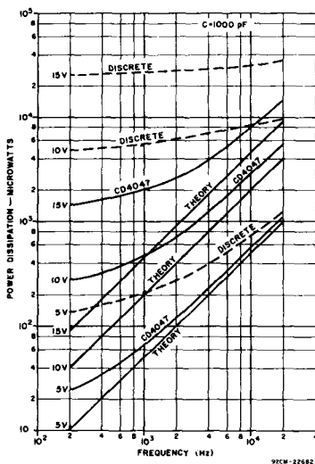
Fig. 10 - Comparison of P_{diss} for discrete oscillator and CD4047 with theory. 92CM-22682
