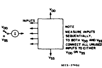
Fig.7 — Input current test circuit.
