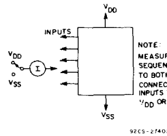
Fig. 11 — Input-leakage current.
