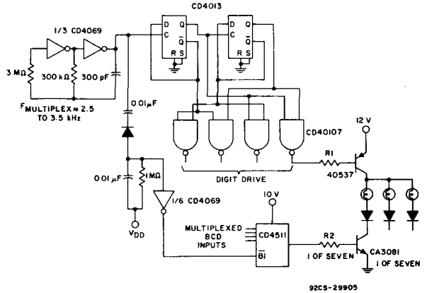
Fig. 19 - Circuit for interfacing a multiplexed incandescent-type digital display.
