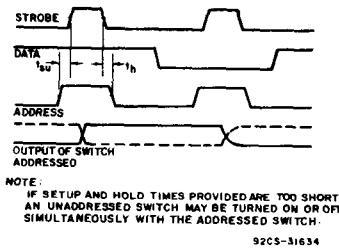
Fig. 20 — Address to strobe setup and hold times.
