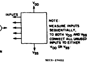
Fig. 12 — Input current test circuit.
