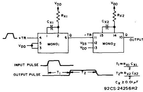
Fig. 15 - Pulse delay.
