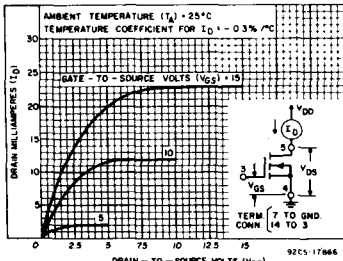
Fig. 8 - Typical output n-channel drain characteristics.
