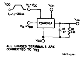
Fig. 13 - Test circuit for square-wave input response.
