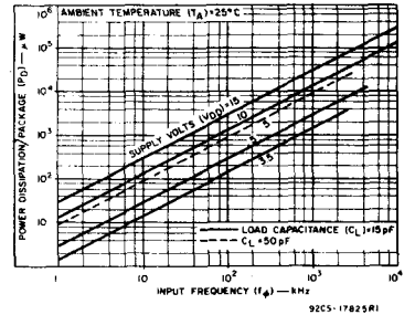
Fig.11 — Typical dissipation characteristics.
