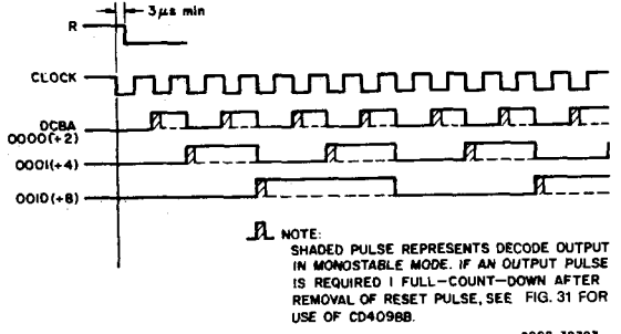
Fig. 31—CD4536B Timing Diagram.
