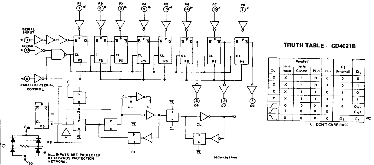
Fig. 2 - Logic diagram for CD4021B.
