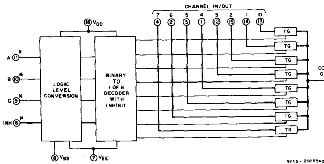
Fig. 1 - Functional diagram of CD4051B.
