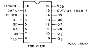
Fig. 1 — Terminal assignment.
