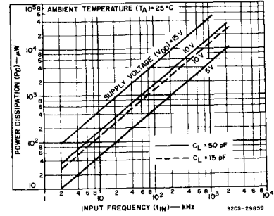
Fig. 7 — Typical dynamic power dissipation as a function of frequency.
