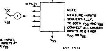
Fig. 21 - Input leakage current test circuit.
