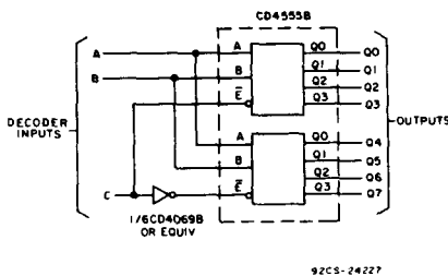
Fig. 20 - 1-of-8 decoder using CD4555B.
