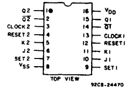
TERMINAL ASSIGNMENT
