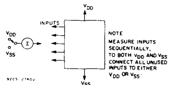
Fig.14 — Input current test circuit.
