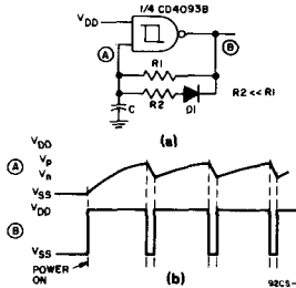
Fig. 17 - Astable oscillator with control'd mark-to-space ratio.
