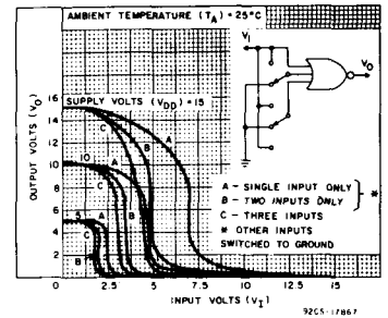
Fig. 4 - Typical voltage-transfer characteristics for NOR gate.
