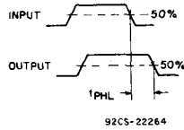
Fig. 18 - Waveforms for t_{PHL} and t_{PHL} (AND).
