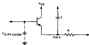
Fig. 16 - CD4047A clamping circuit.
