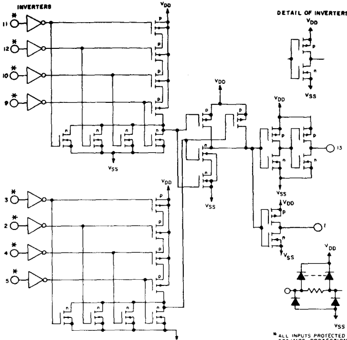
Fig. 7 - Schematic diagram.
