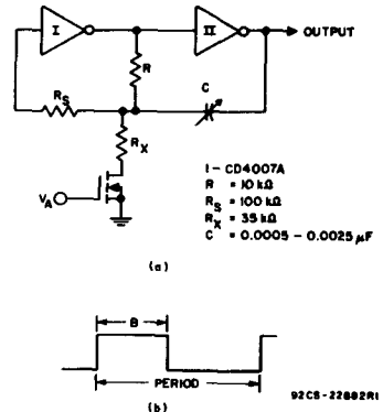
Fig. 20(a) - Voltage controlled pulse-width circuit, (b) output waveform.
