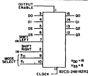
4-Bit Universal Bidirectional Shift Register 3-State Outputs
