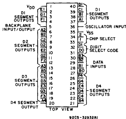
CD22105, CD22105A Terminal Assignment
