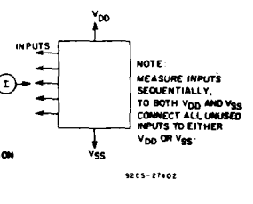
Fig. 10 — Input voltage test circuit.
