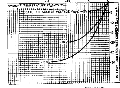
Fig. 7 - Typical output high (source) current characteristics.
