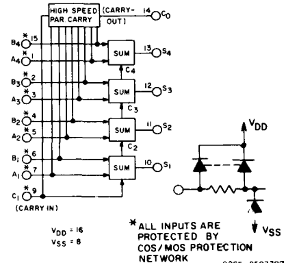
Fig. 1 - CD4008A logic diagram.
