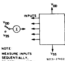
Fig. 22 - Input current test circuit.
