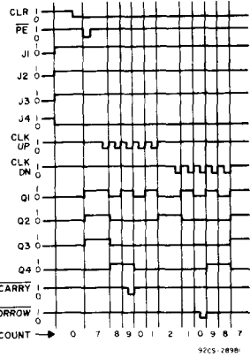
Fig. 3 - CD40192B timing diagram.
