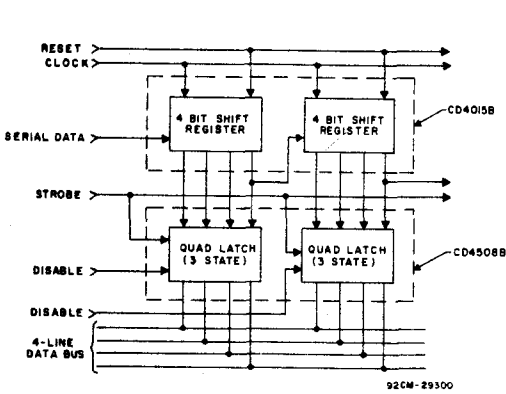
Fig. 15 - Bus register.
