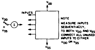
Fig. 14 — Input leakage current test circuit.
