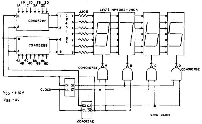
Fig. 8 - Multiplexed LED circuit.
