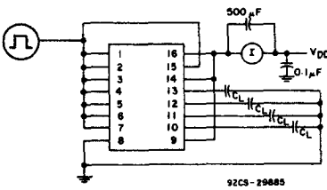
Fig. 9 — Dynamic power dissipation test circuit.
