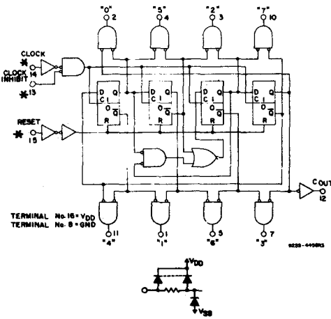
Fig. 1 - Logic diagram.
