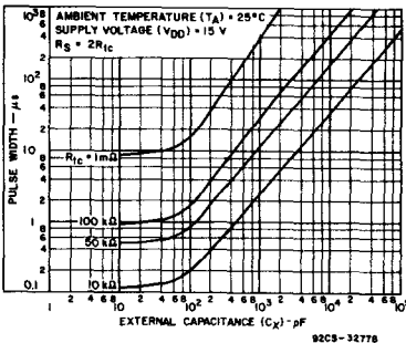
Fig. 17—Typical pulse width as a function of external capacitance ( V_{DD} = 15 \text{ V} ).
