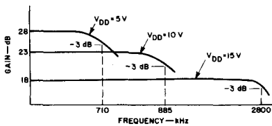
(b) TYPICAL CD4001UB LINEAR GAIN
