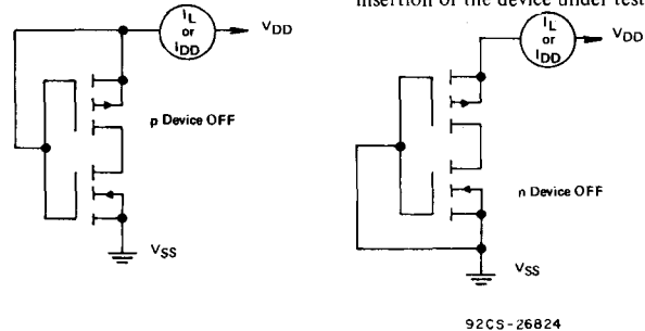
Fig. 8 — Measurement of quiescent leakage current.
