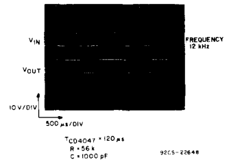
Fig. 33 - Envelope-detector-circuit waveforms.
