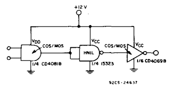
Fig. 5-COS/MOS to HN1L to COS/MOS interface.
