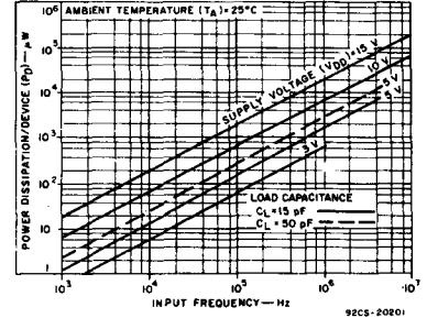
Fig. 8 — Typical dissipation characteristics.
