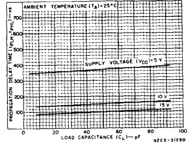
Fig. 8 — Typical propagation delay time ( Q_1 to Q_4 Output) as a function of load capacitance.
