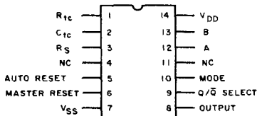
TERMINAL ASSIGNMENT
