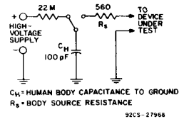
Fig. 5 - Equivalent-body discharge network.
