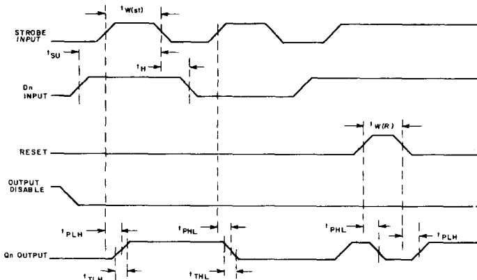
Fig. 12 — Test waveforms.
